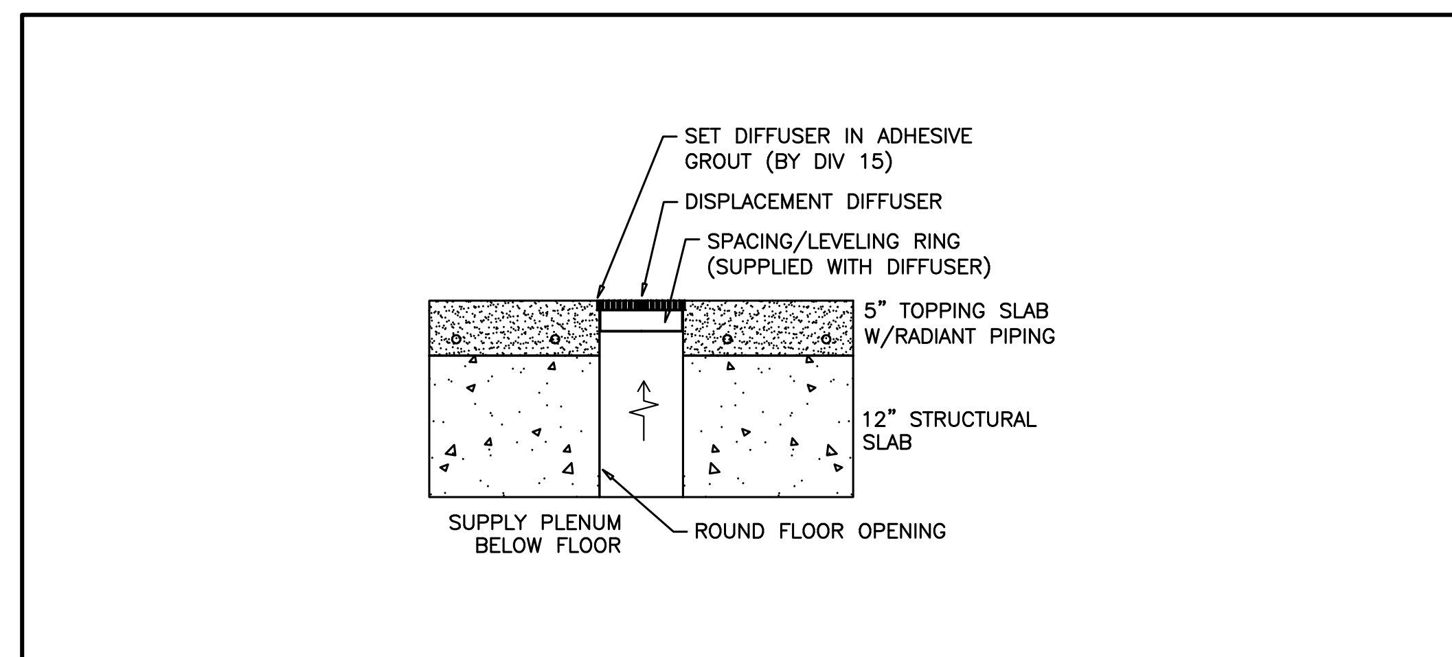
4 CATHEDRAL FLOOR DIFFUSER M3.1 1"=1'0"
