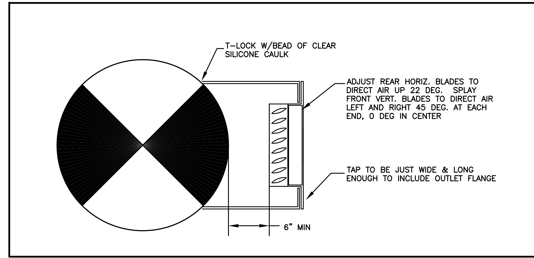
2 EXPOSED SIDEWALL GRILLE DETAIL M3.1 NTS
