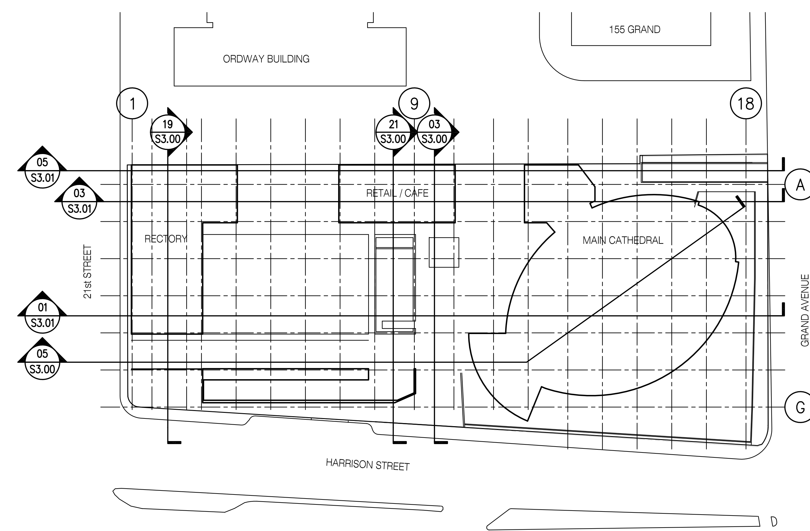
KEY PLAN FOR SECTIONAL VIEWS SCALE: NONE S300-01-04 01
