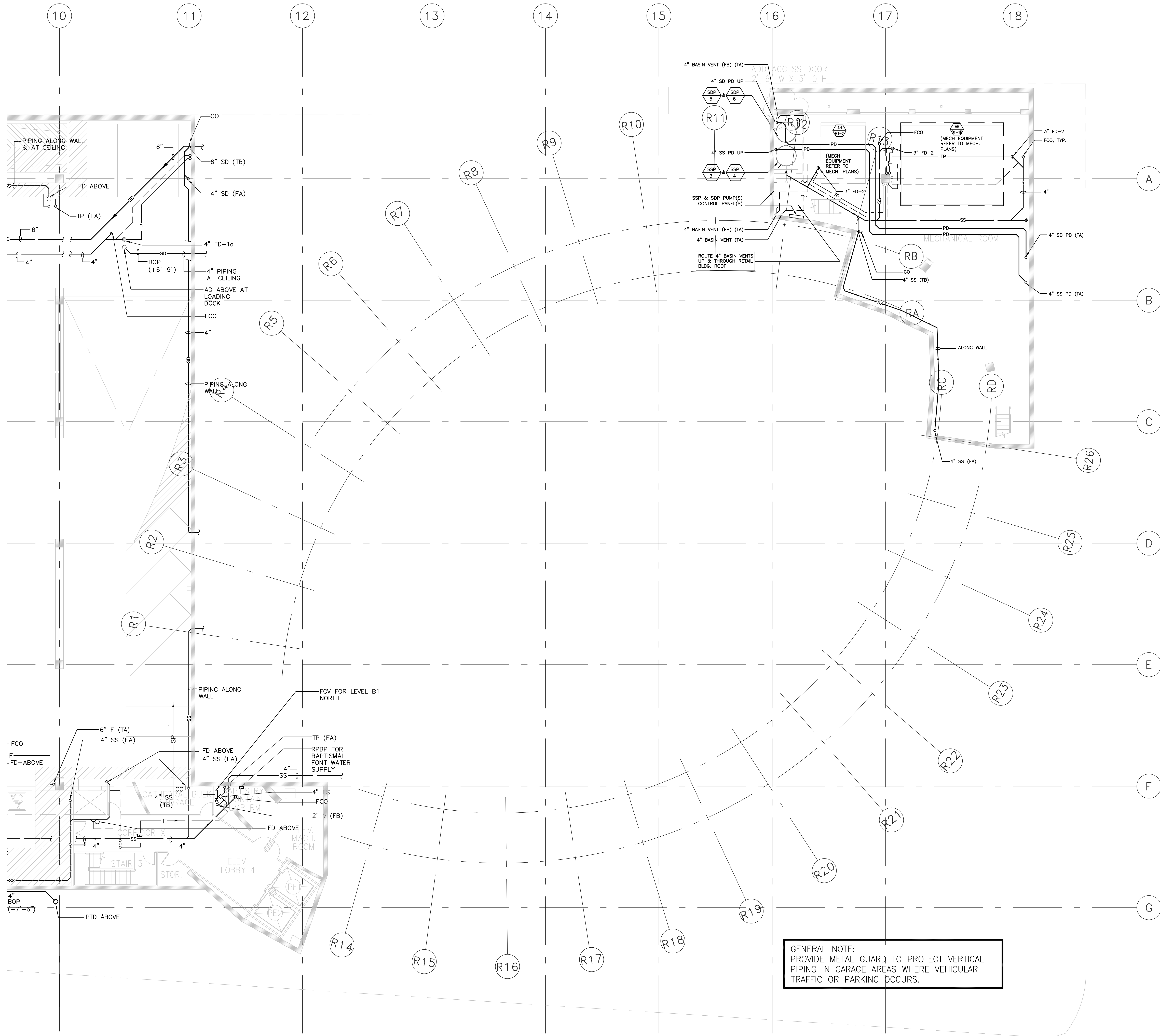
1 PARTIAL LEVEL B1 PLUMBING PLAN P2.B1.1 1/8" = 1'-0"
