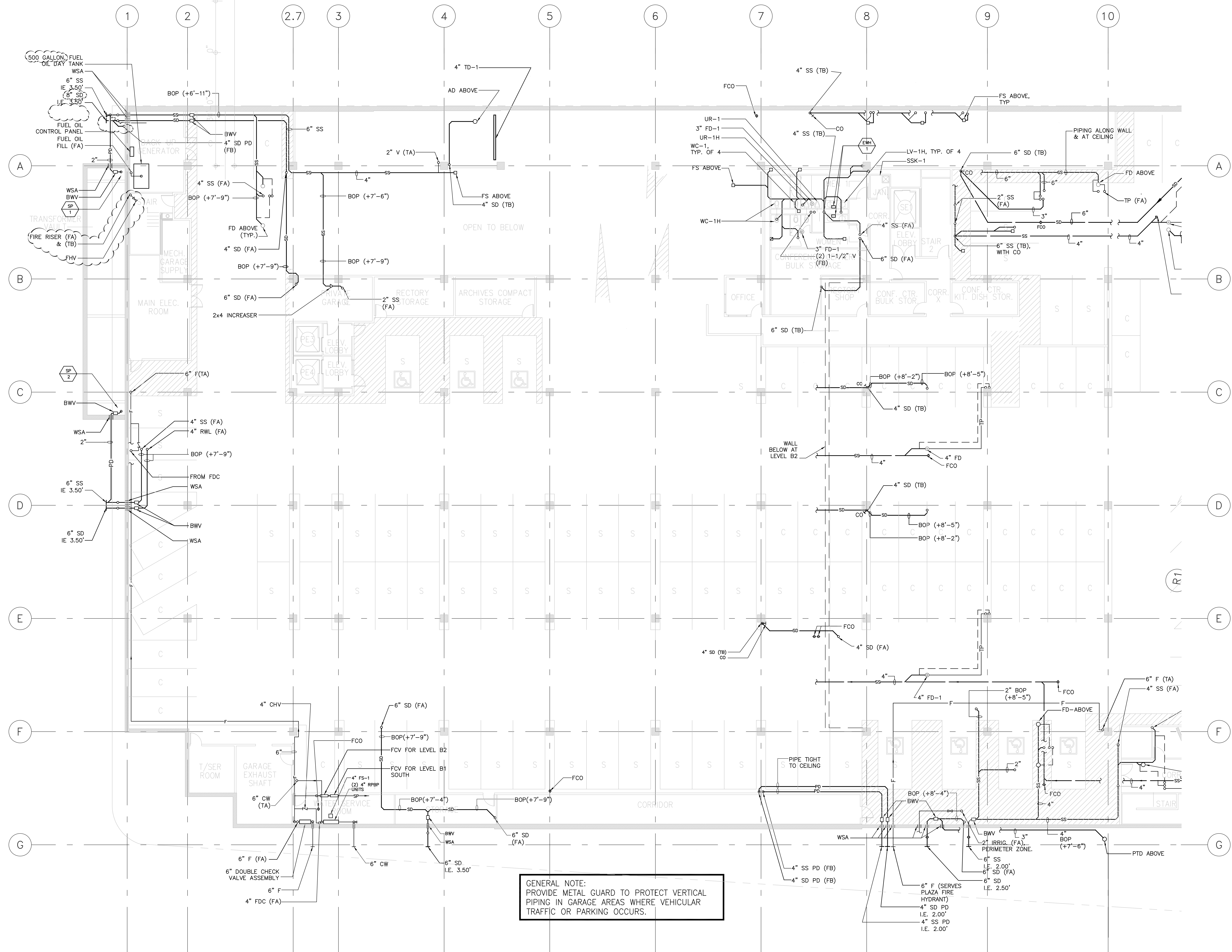
1 PARTIAL LEVEL B1 PLUMBING PLAN P2.B1.1 1/8" = 1'-0"
