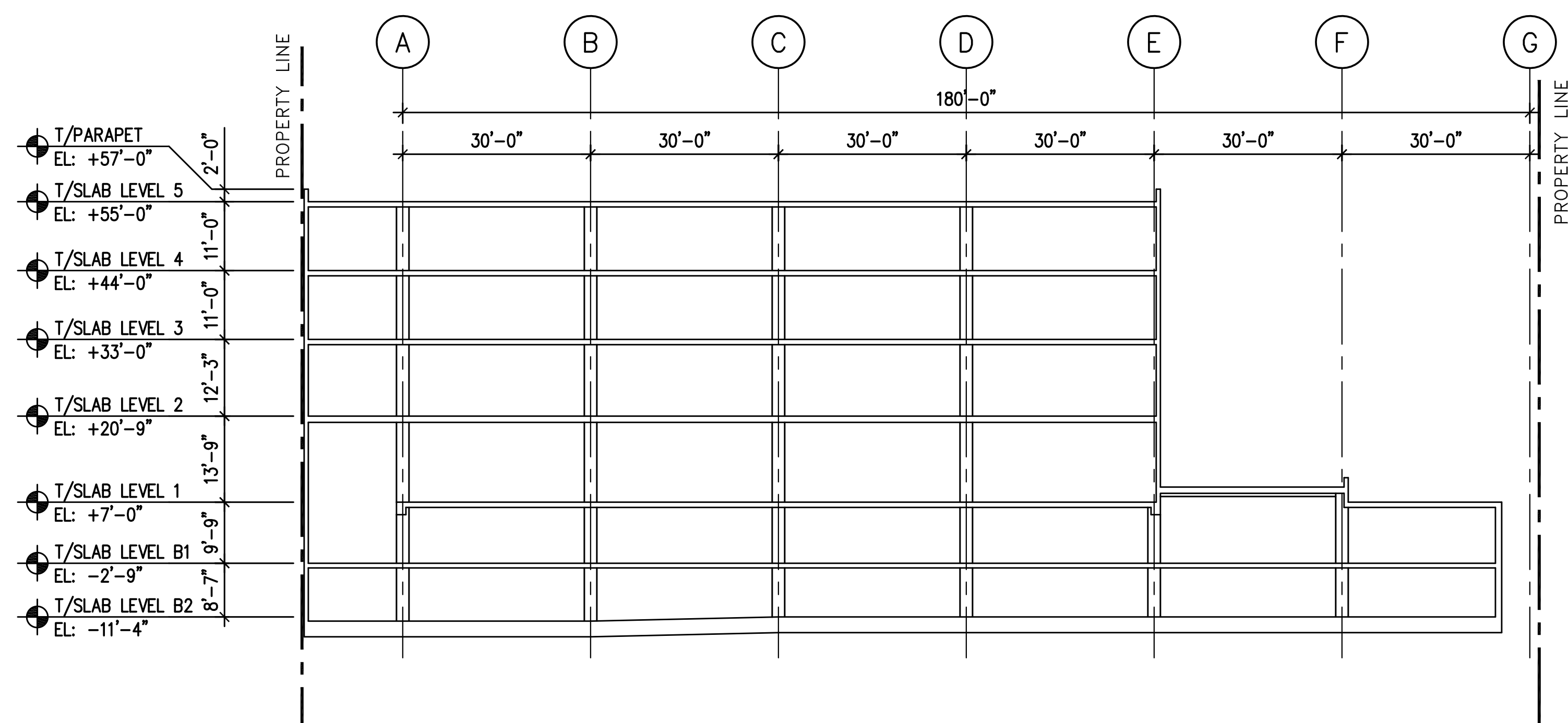
OVERALL SITE SECTION BETWEEN GRIDLINE 2 AND 2.7 SCALE: 1/16" = 1'-0" S300-01-04 19
