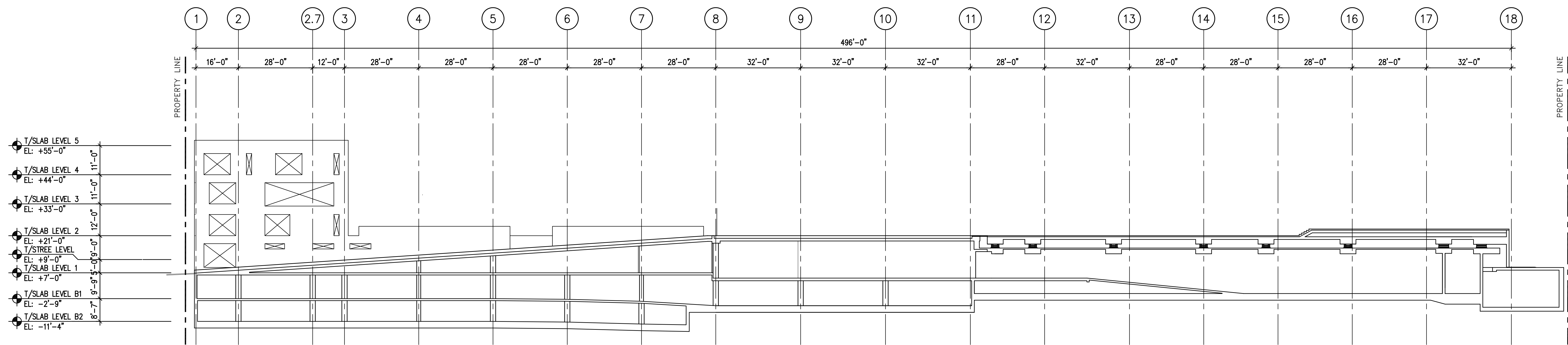
OVERALL SITE SECTION THROUGH PILGRIMS WALK SCALE: 1/16" = 1'-0" S300-01-04 05
