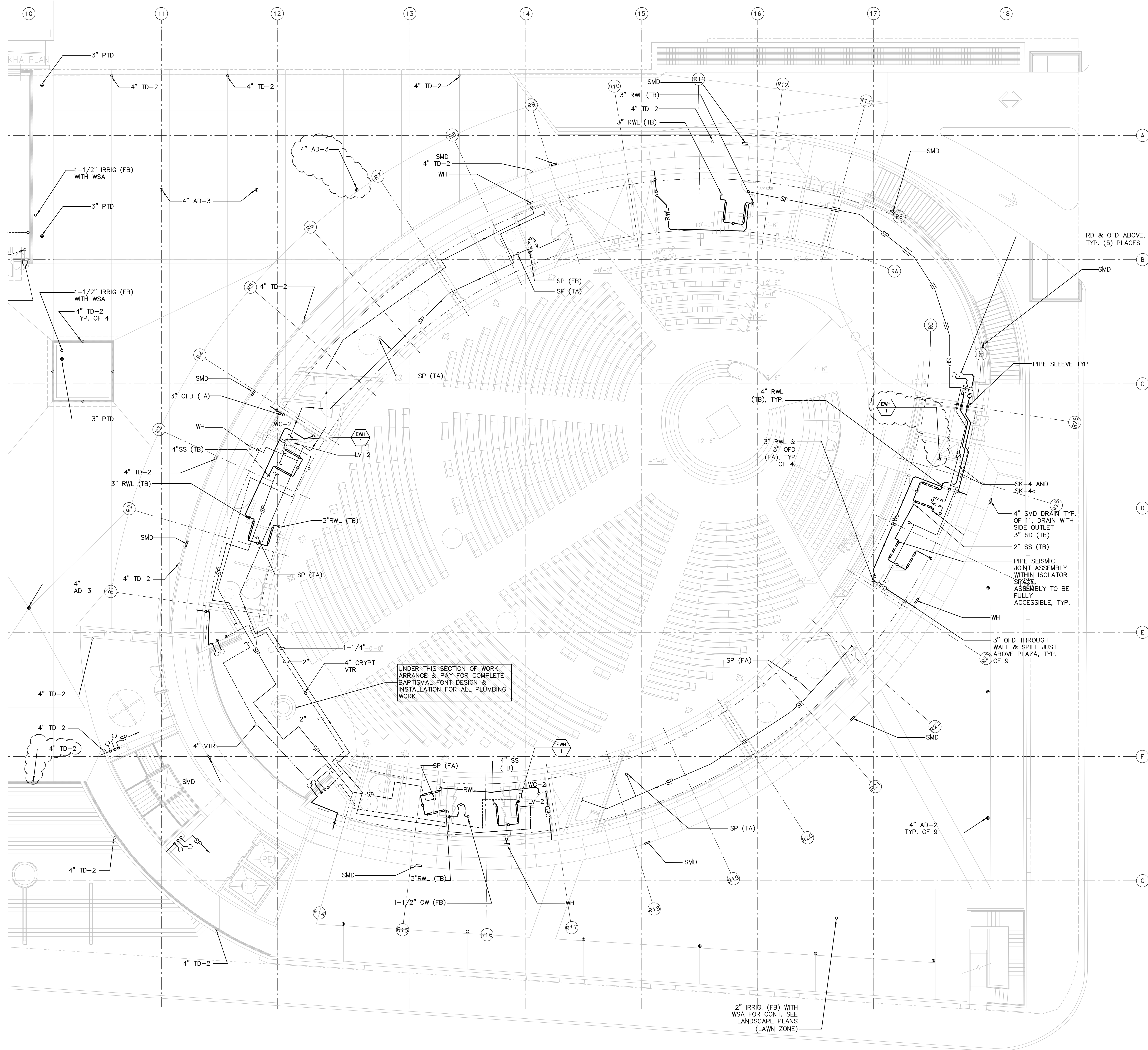
1 PARTIAL SECOND FLOOR PLUMBING PLAN P2.2.4 1/8" = 1'-0"
