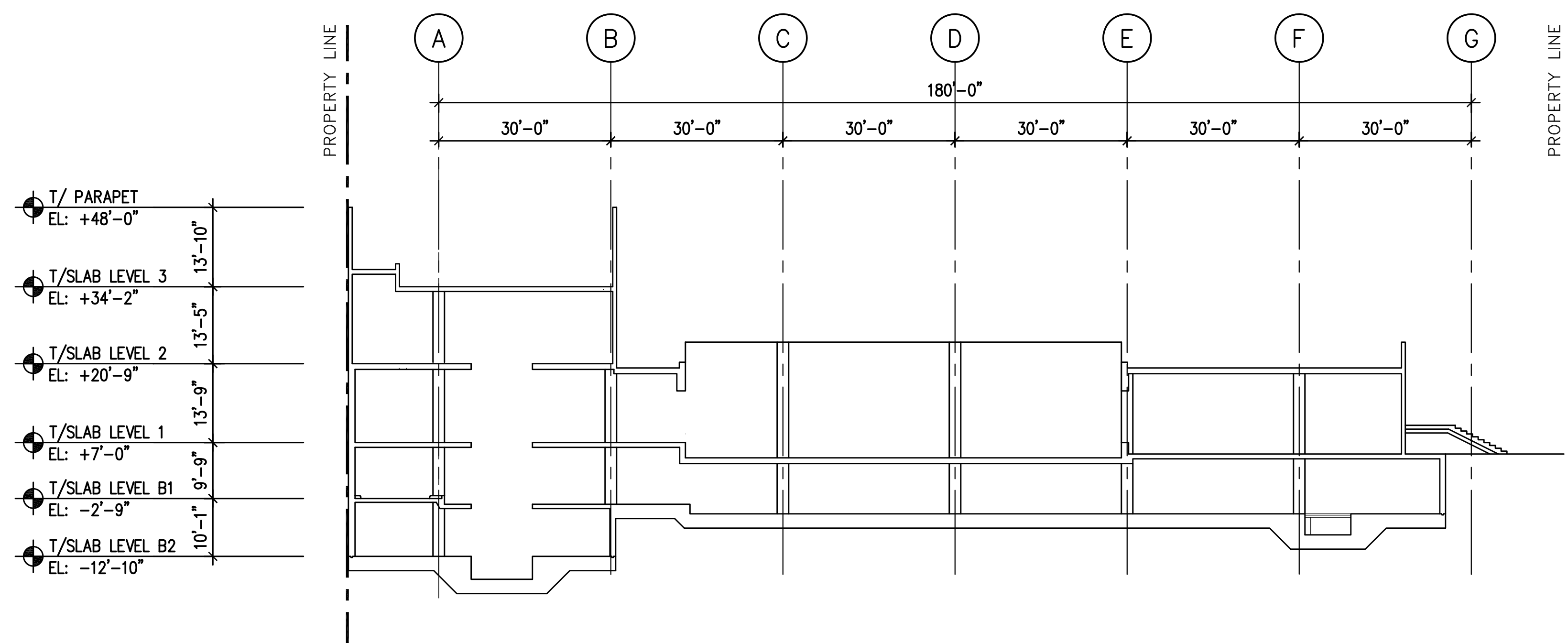
OVERALL SITE SECTION BETWEEN GRIDLINE 8 AND 9 SCALE: 1/16" = 1'-0" S300-01-04 21
