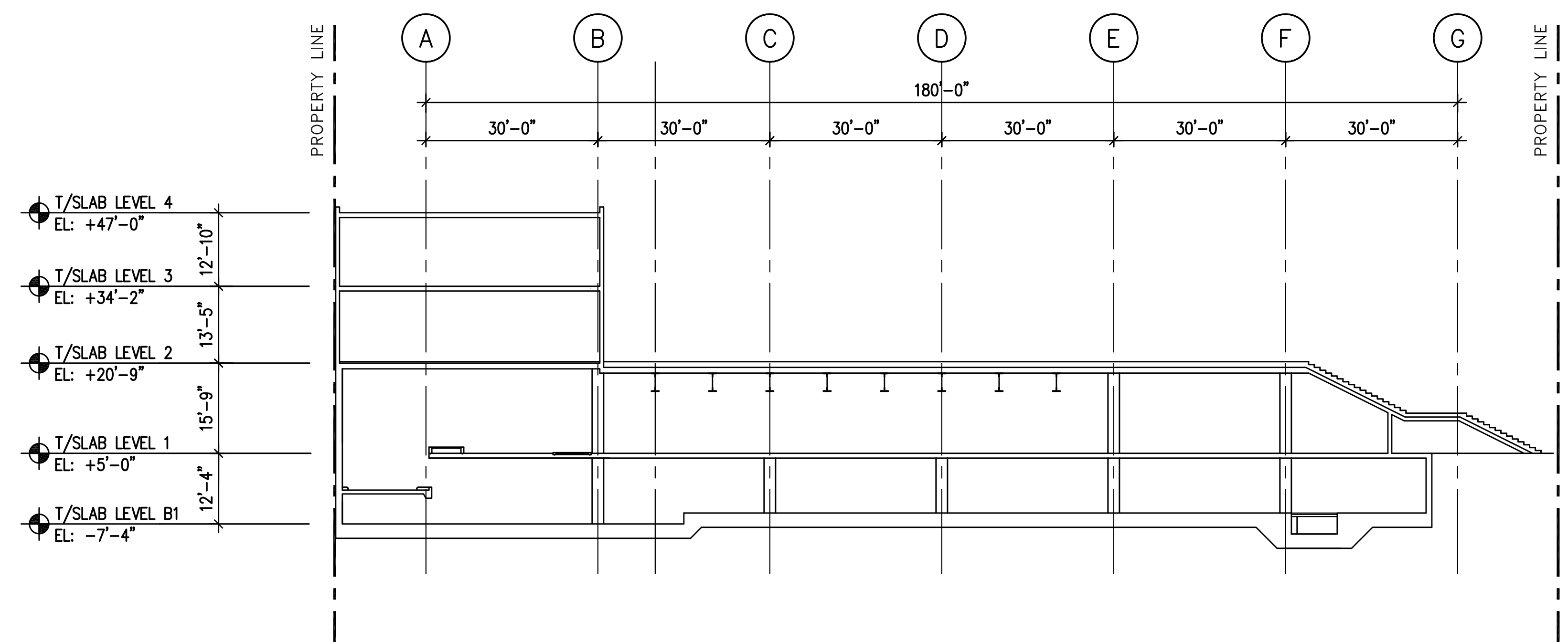
OVERALL SITE SECTION BETWEEN GRIDLINE 9 AND 10 SCALE: 1/16" = 1'-0" S300-01-04 03
