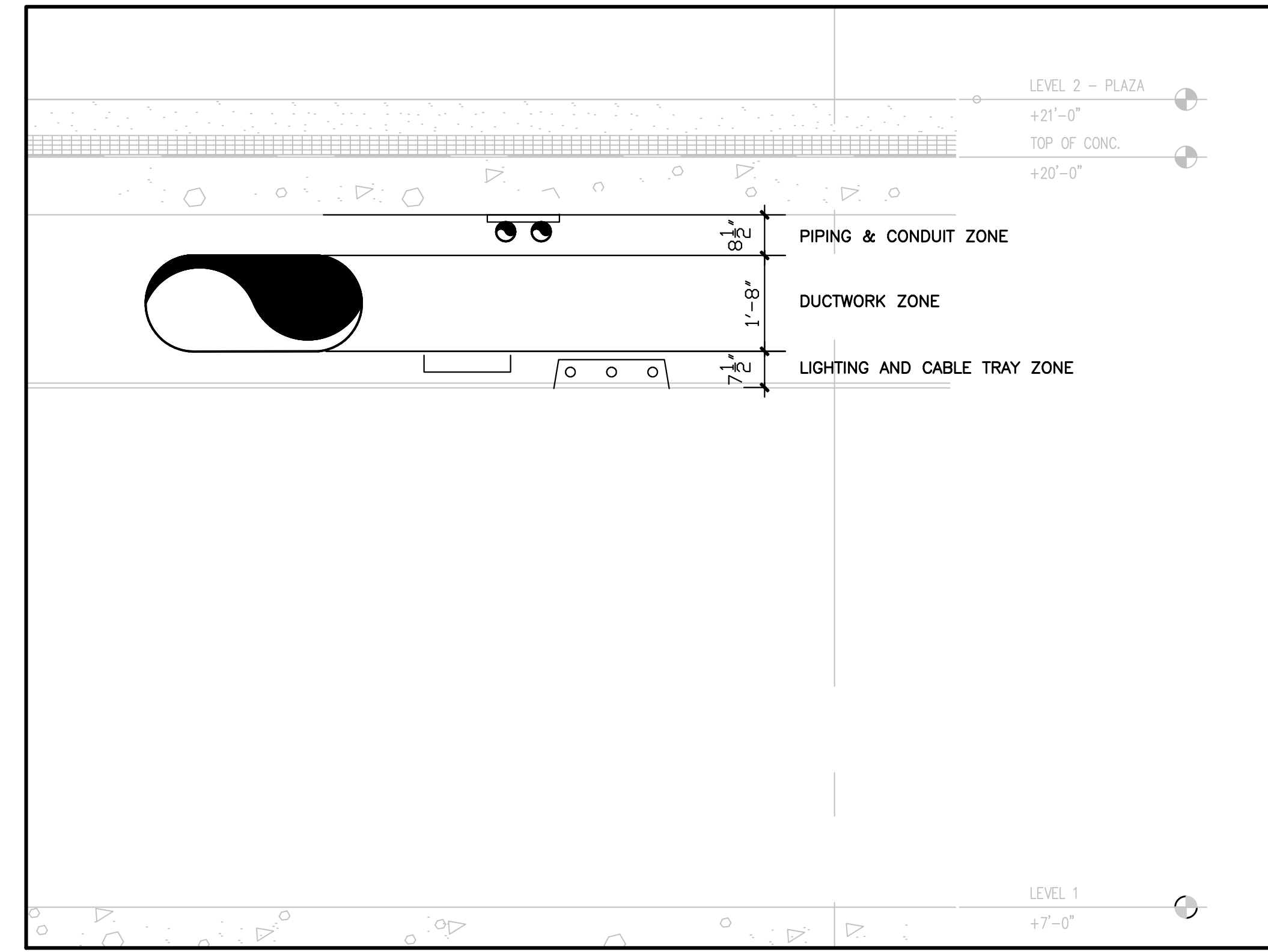
5 TYPICAL CEILING COORDINATION SECTION M3.1 1/2"=1'0"
