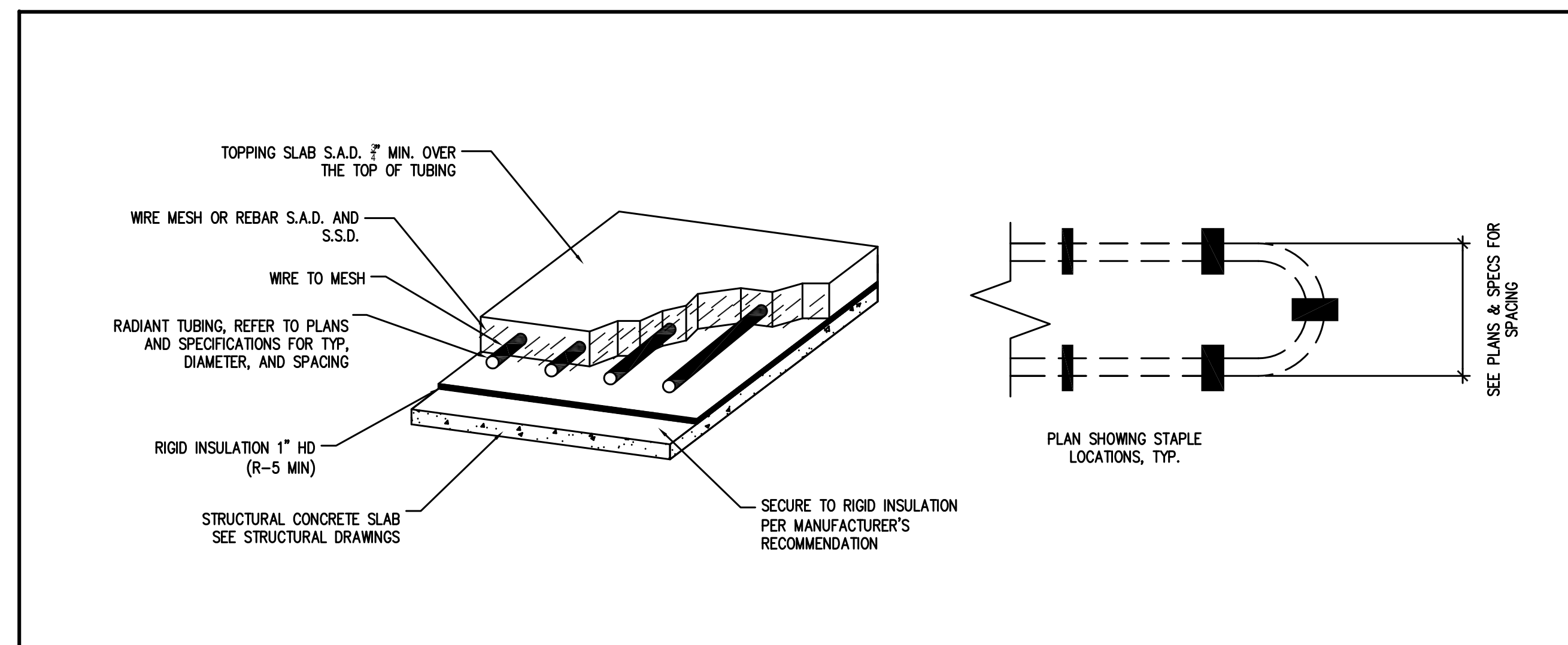
3 RADIANT SLAB DETAIL M3.1 NTS
