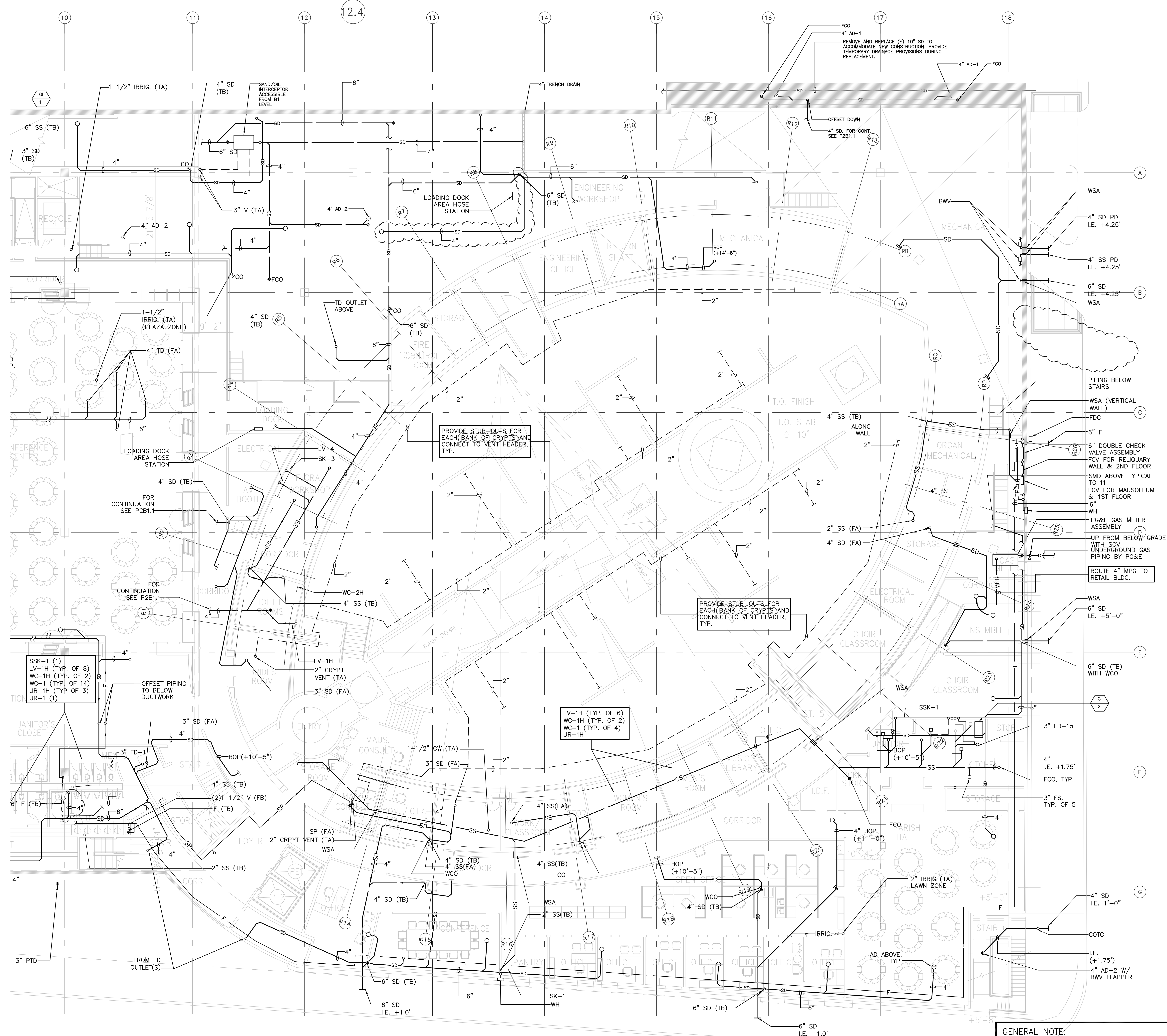
1 PARTIAL FIRST FLOOR PLUMBING PLAN P2.1.4 1/8" = 1'-0"
