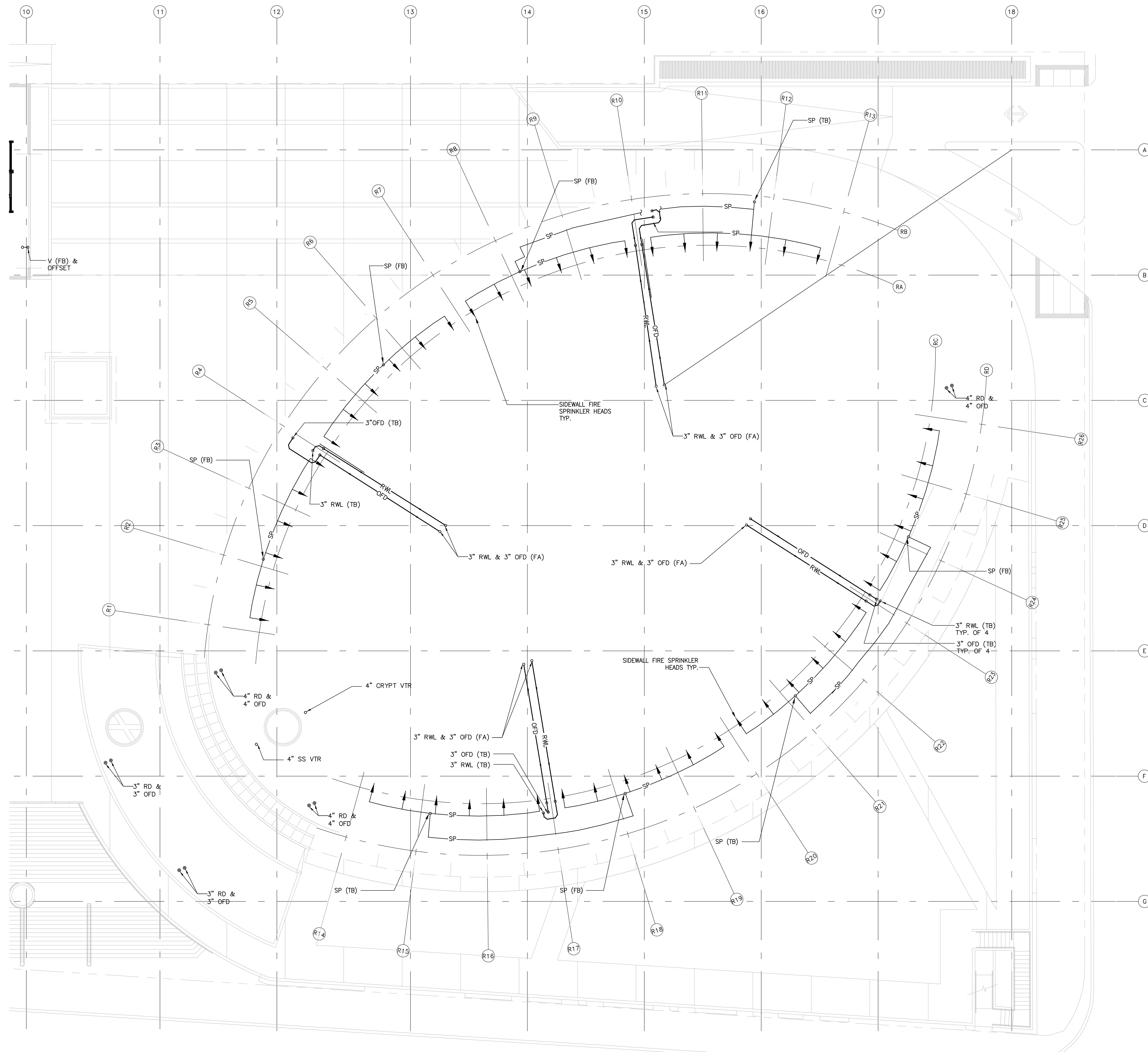
1 PARTIAL THIRD FLOOR PLUMBING PLAN P2.3.4 1/8" = 1'-0"
