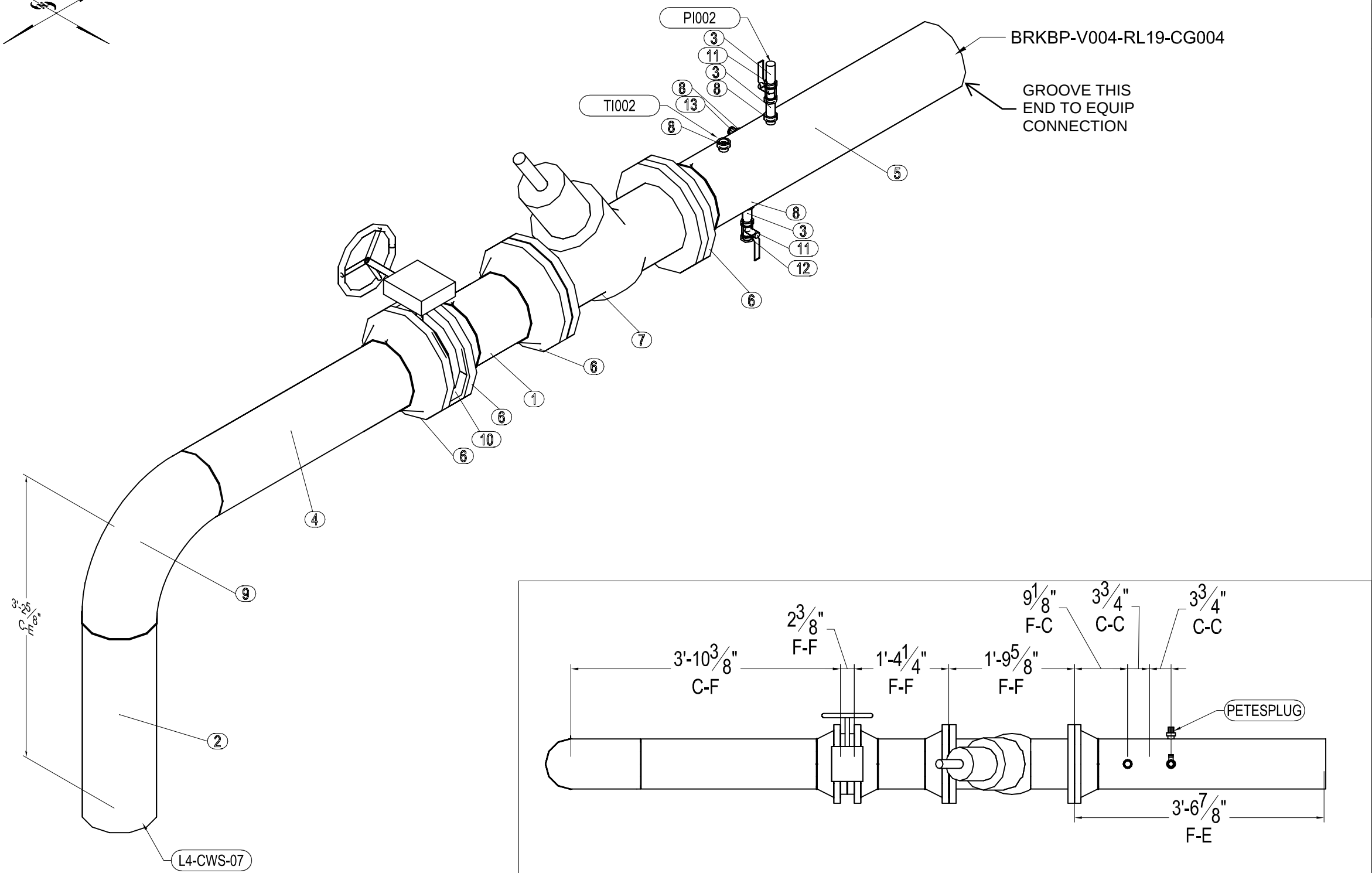
ISO VIEW
