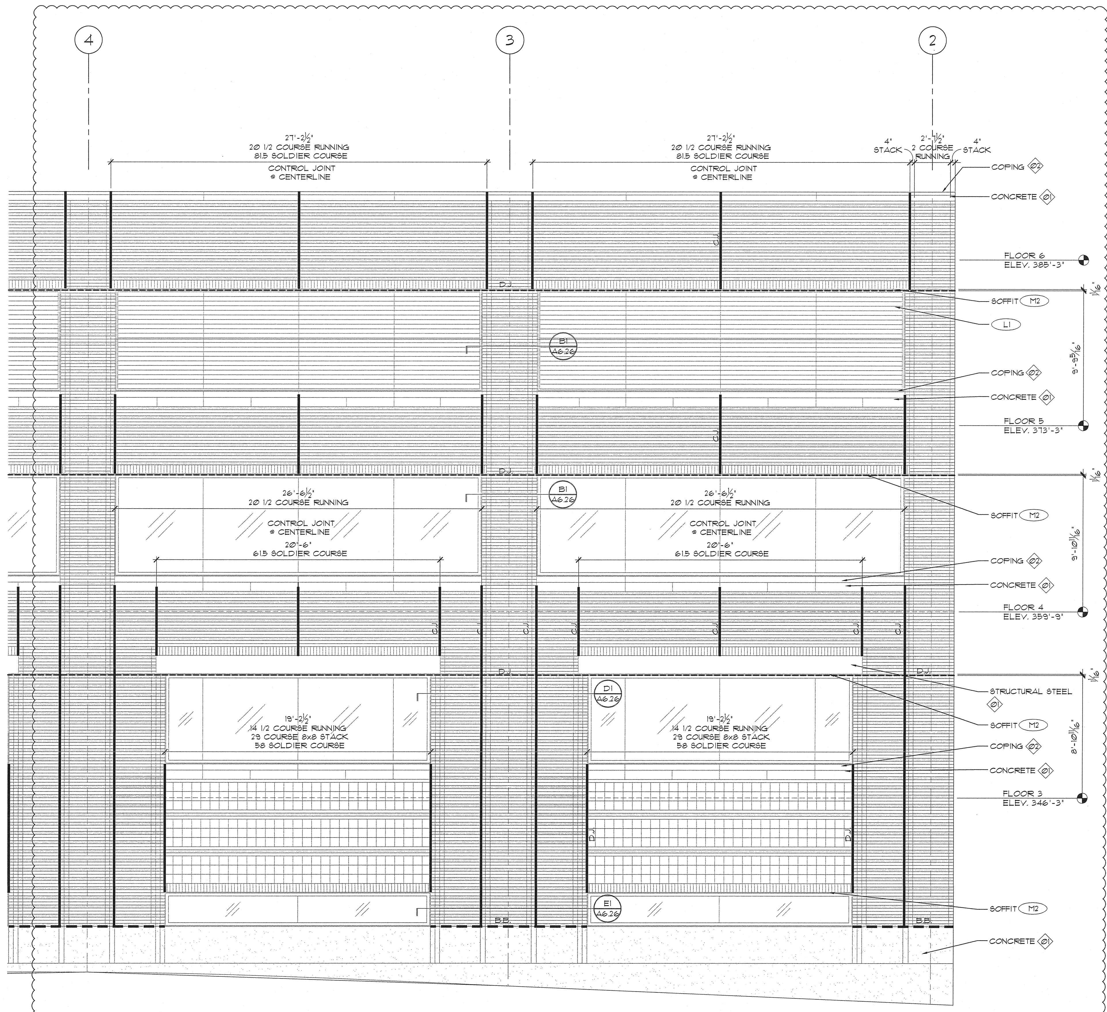
E1 PARTIAL EAST ELEVATION 1/4" = 1'-0"
