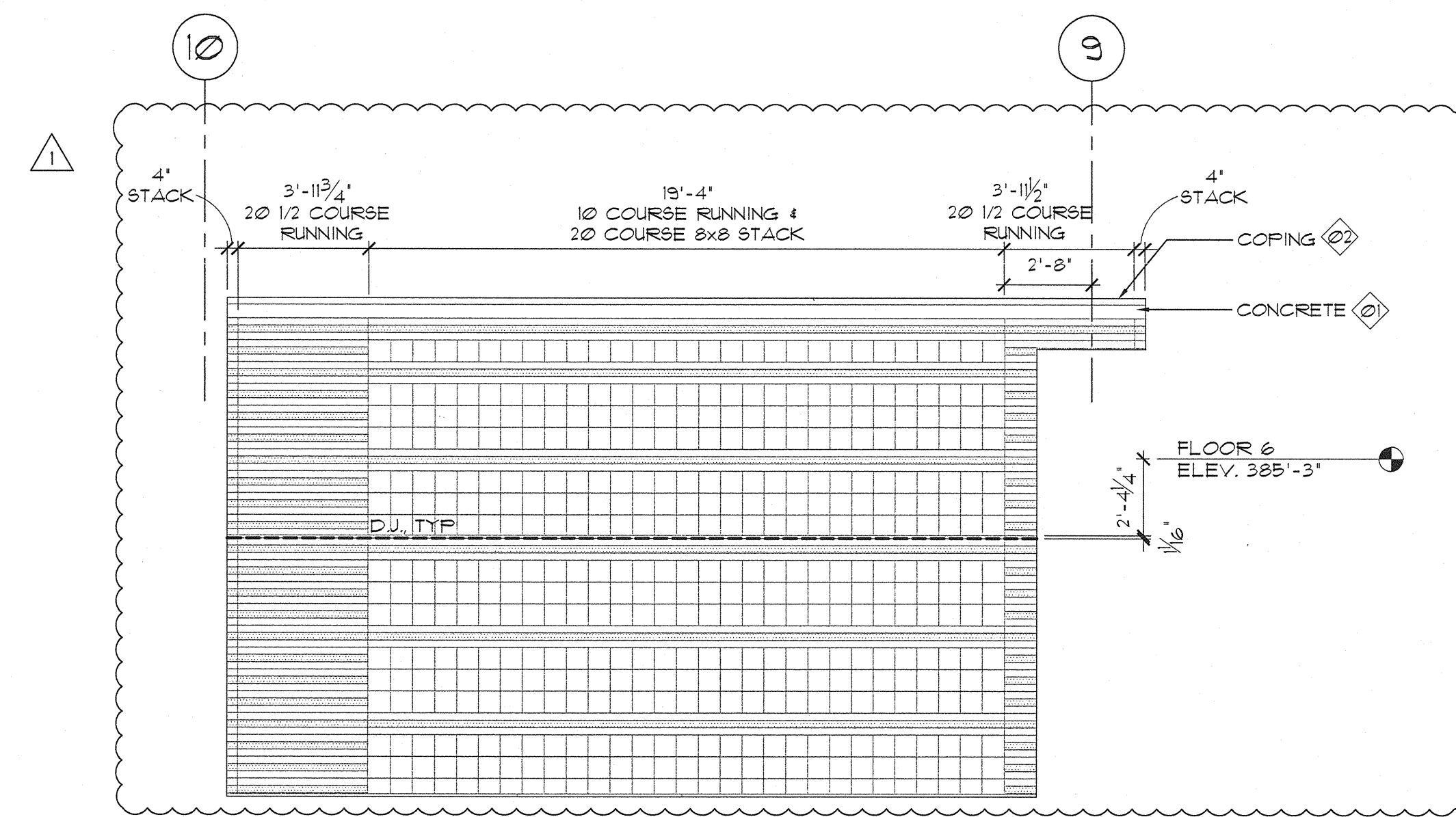
BI PARTIAL EAST ELEVATION 1/4" = 1'-0"
