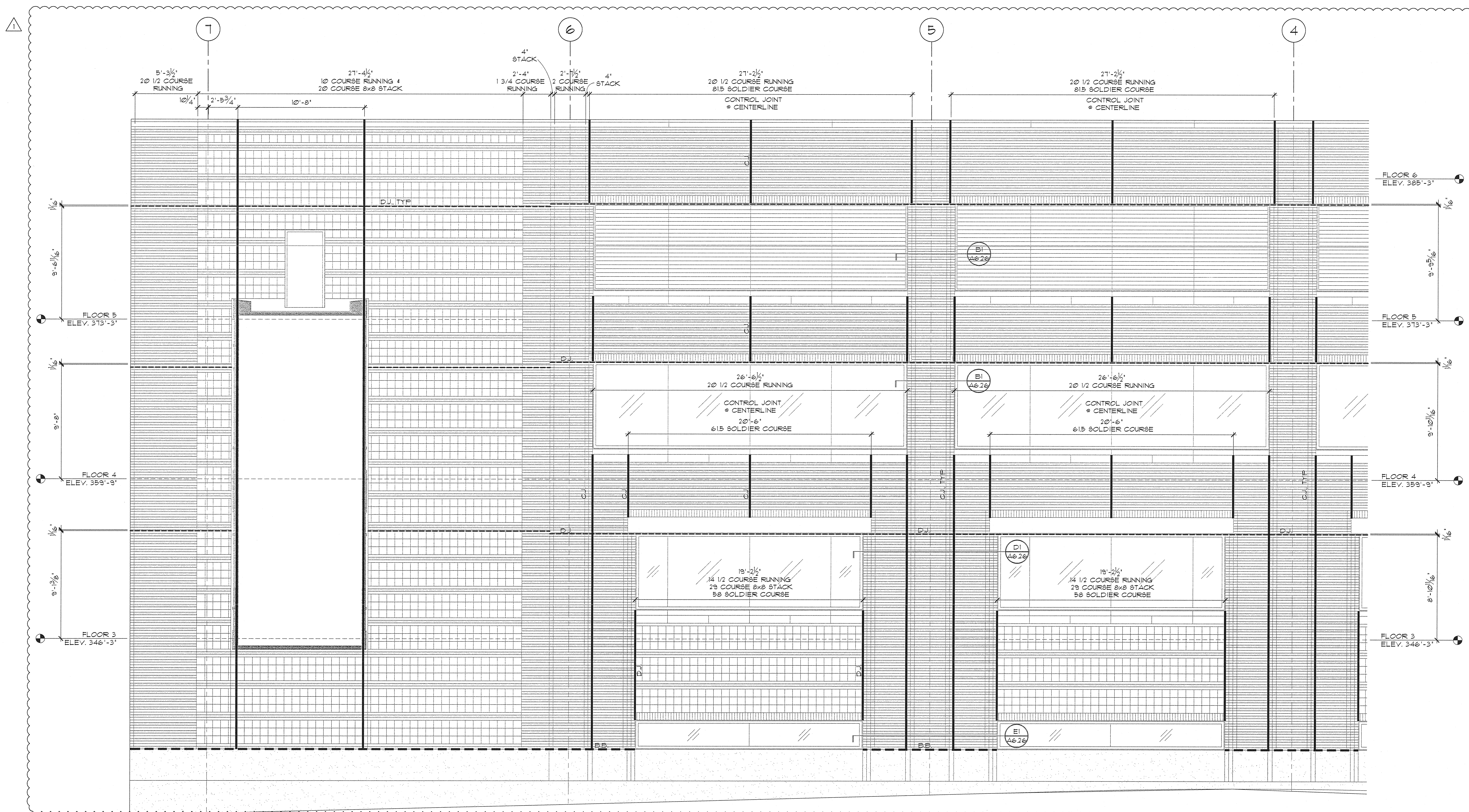
EI PARTIAL EAST ELEVATION 1/4" = 1'-0"
