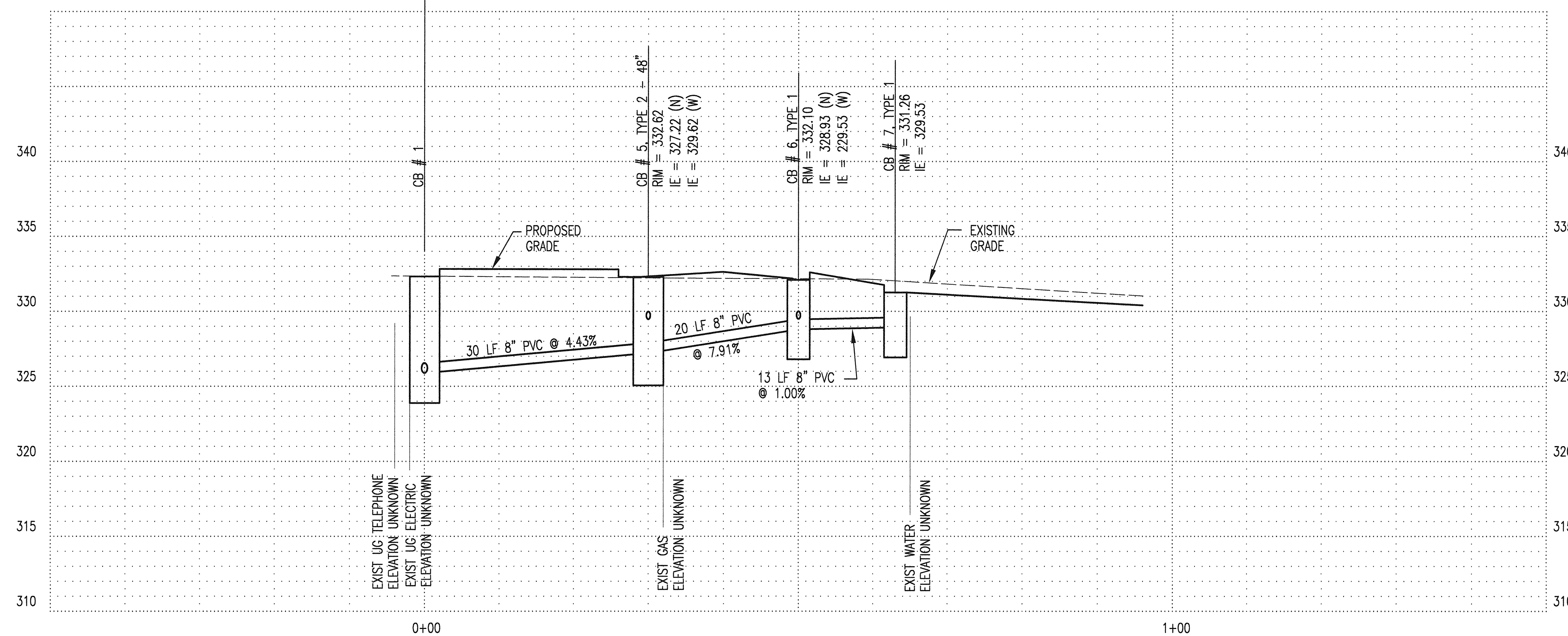
STORMDRAIN PROFILE 2
