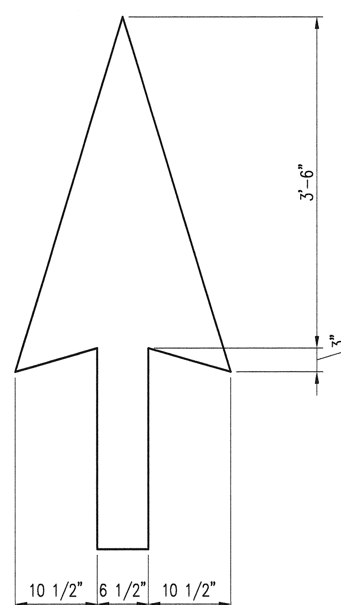
L-22 L-22T THROUGH ARROW NTS
