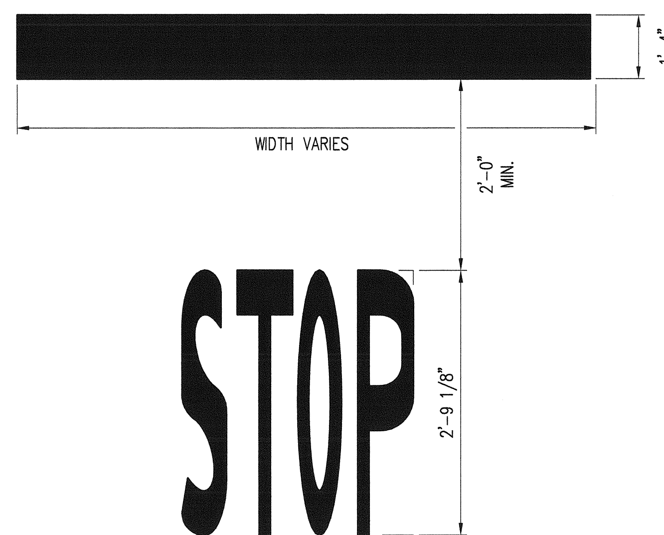
STOP BAR AND TEXT NTS
