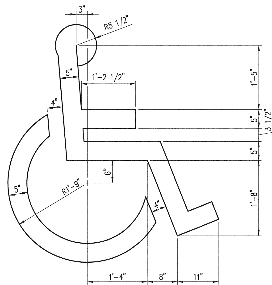
L-29 L-29T DISABLED PERSON SYMBOL NTS
