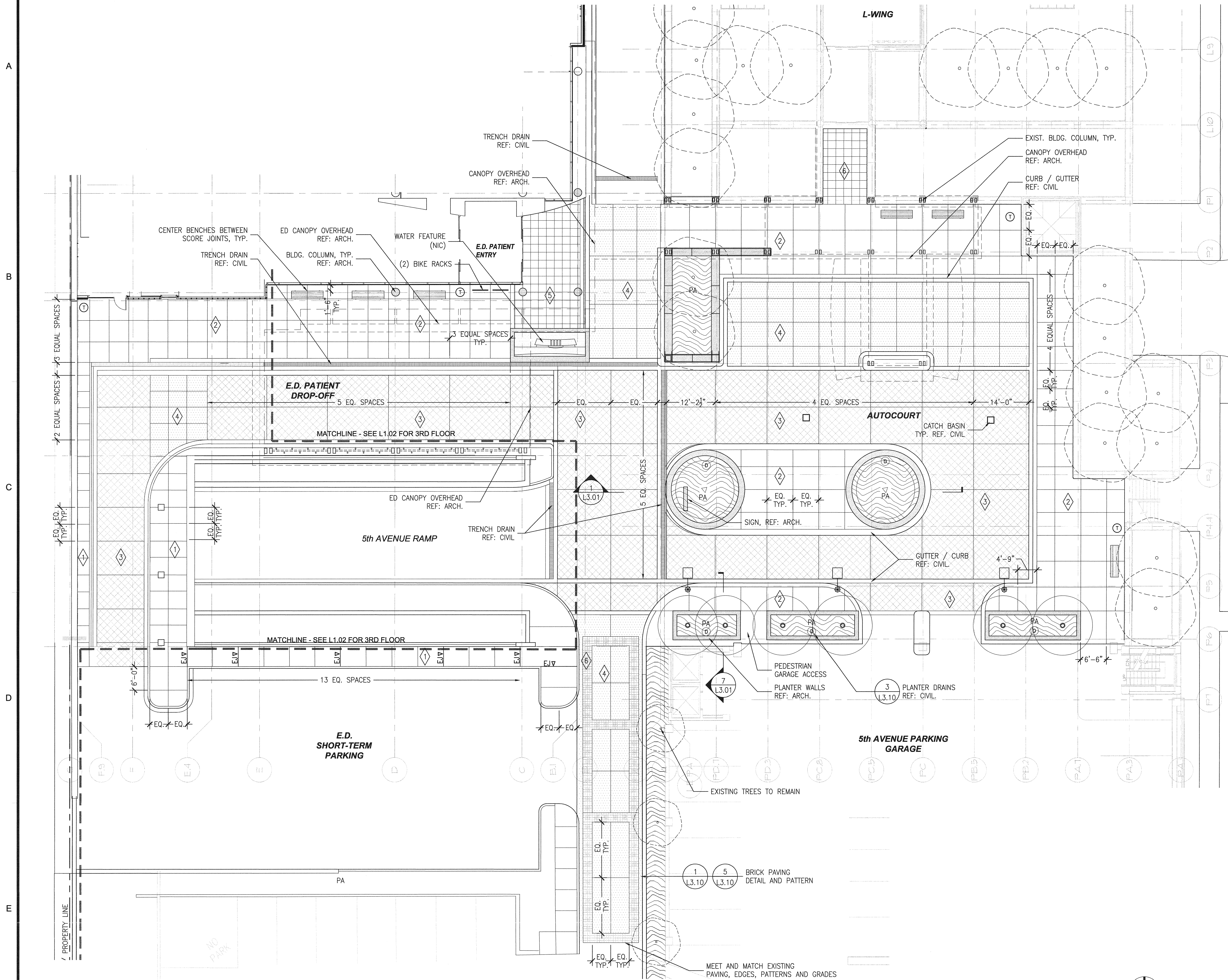
1 LANDSCAPE LAYOUT & MATERIALS PLAN SCALE: 1" = 10' - 0"
