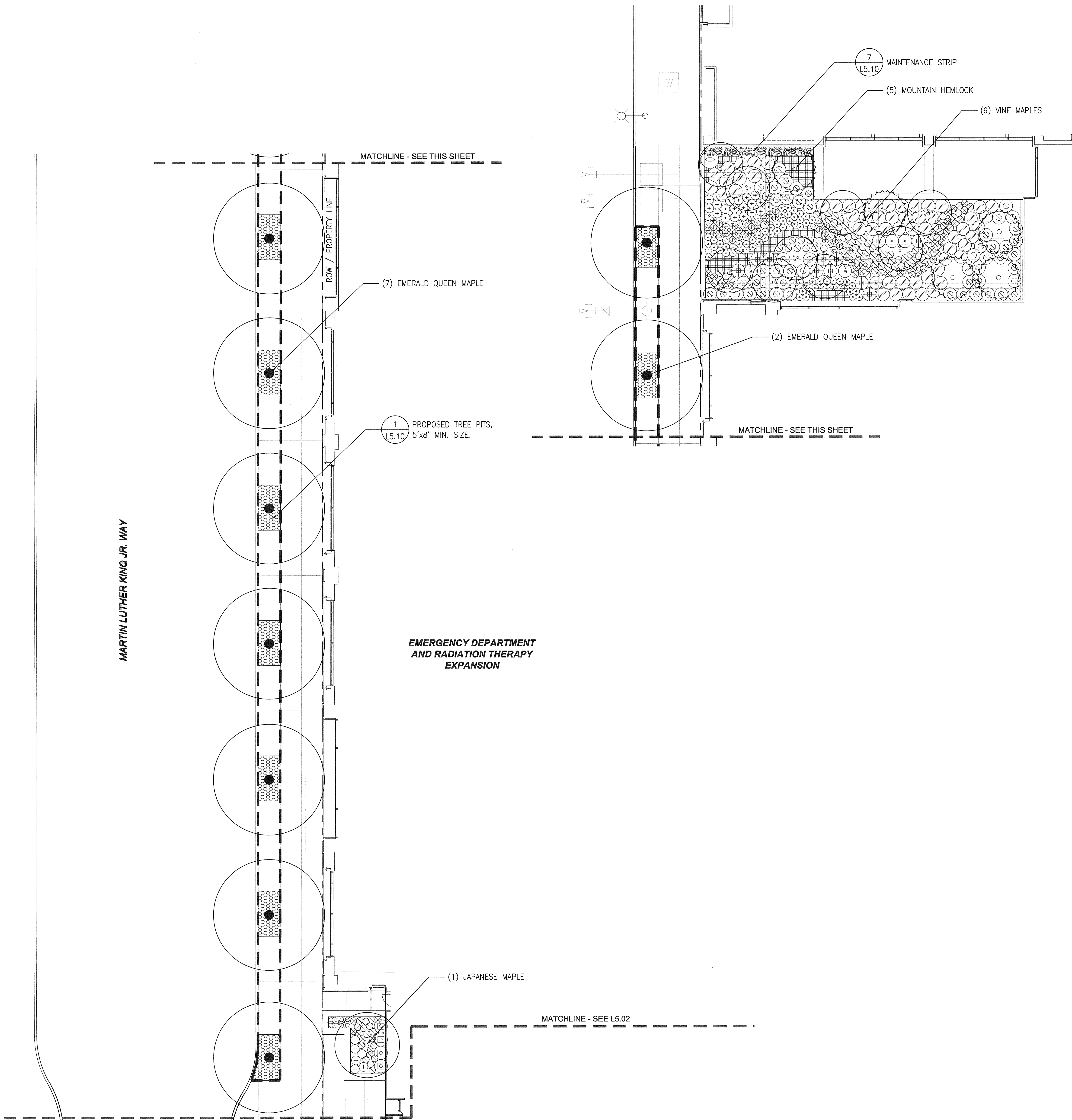
1 PLANTING PLAN SCALE: 1" = 10' - 0"
