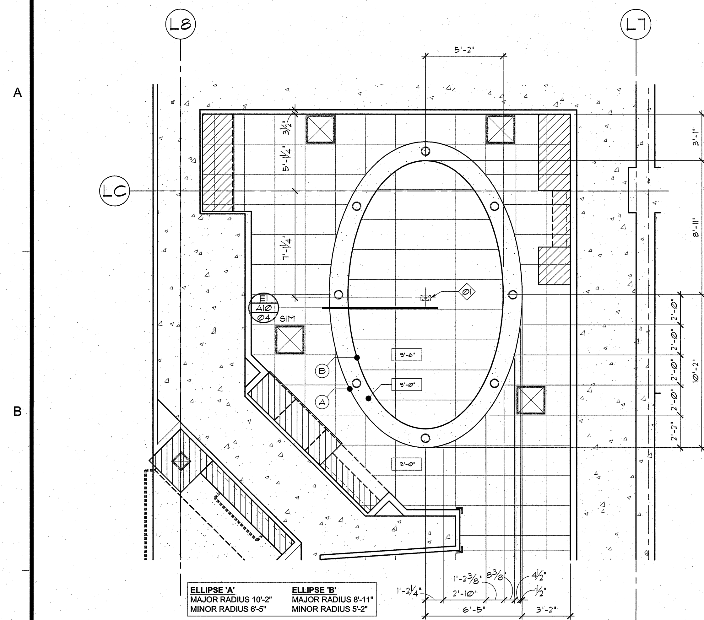
B1 RT-2 Ell28 1/4" = 1'-0"
