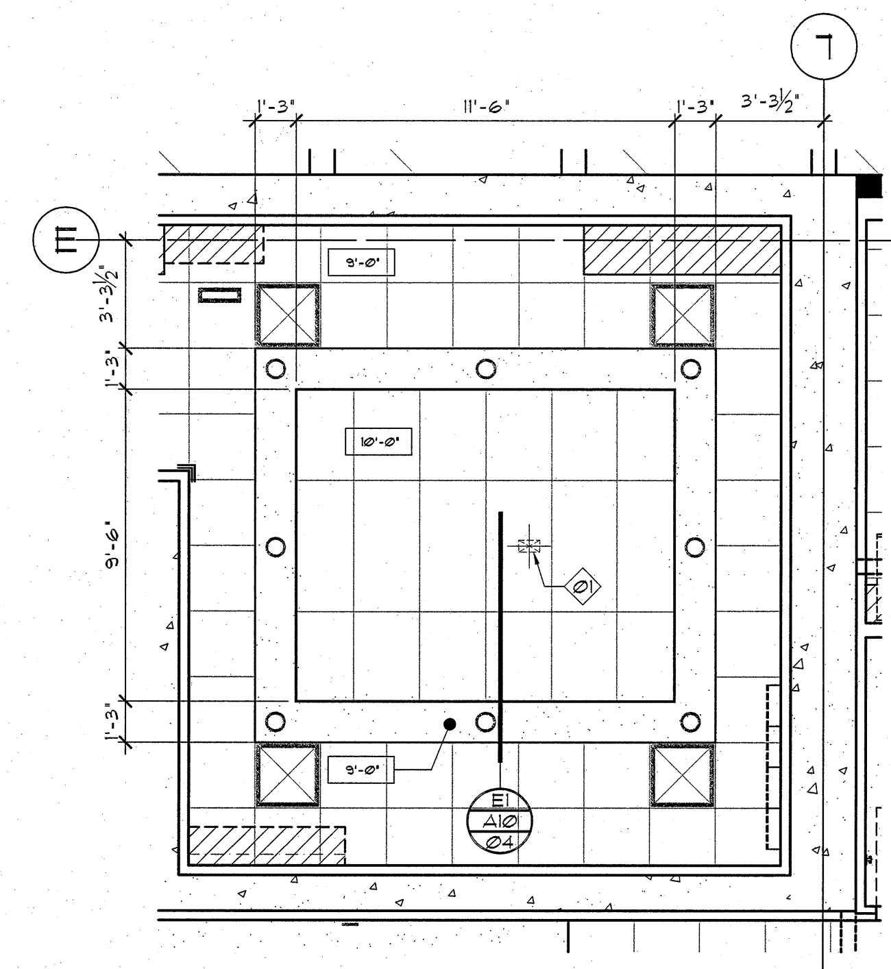
B5 SIMULATOR 2 - HDR ROOM 1062 1/4" = 1'-0"
