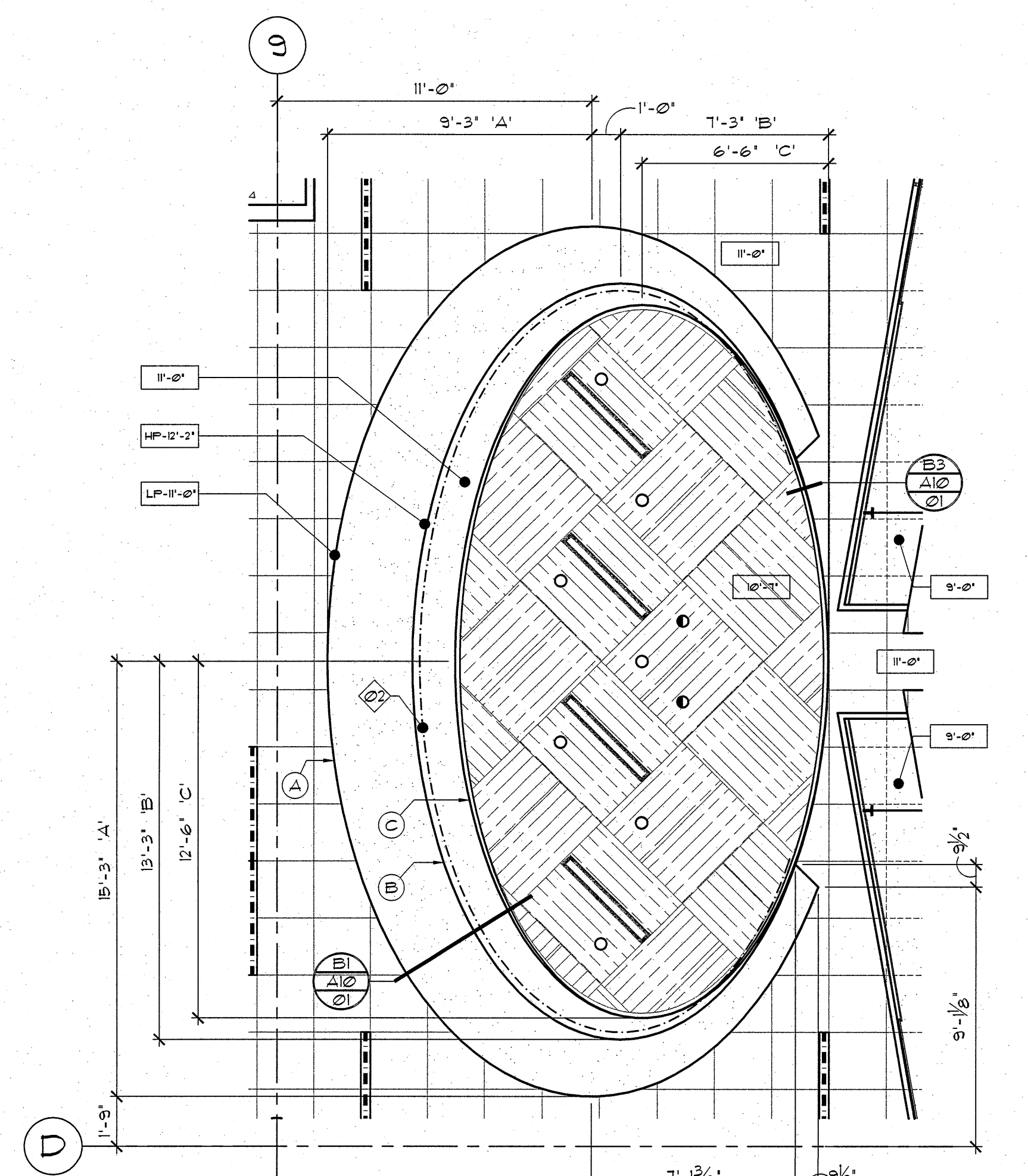
B3 RECEPTION 2006 1/4" = 1'-0"
