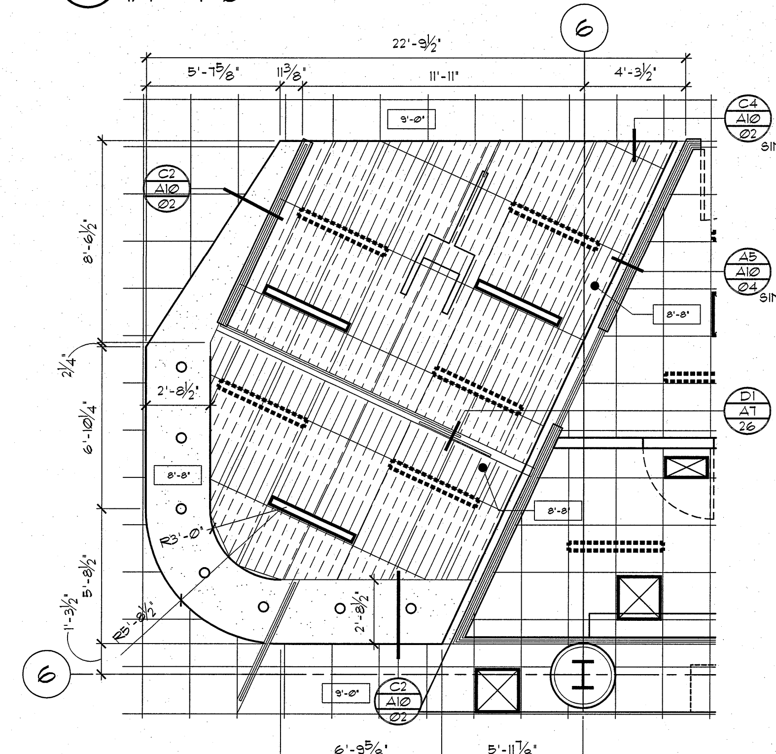
B5 SIMULATOR 2 - HDR ROOM 1062 1/4" = 1'-0"
