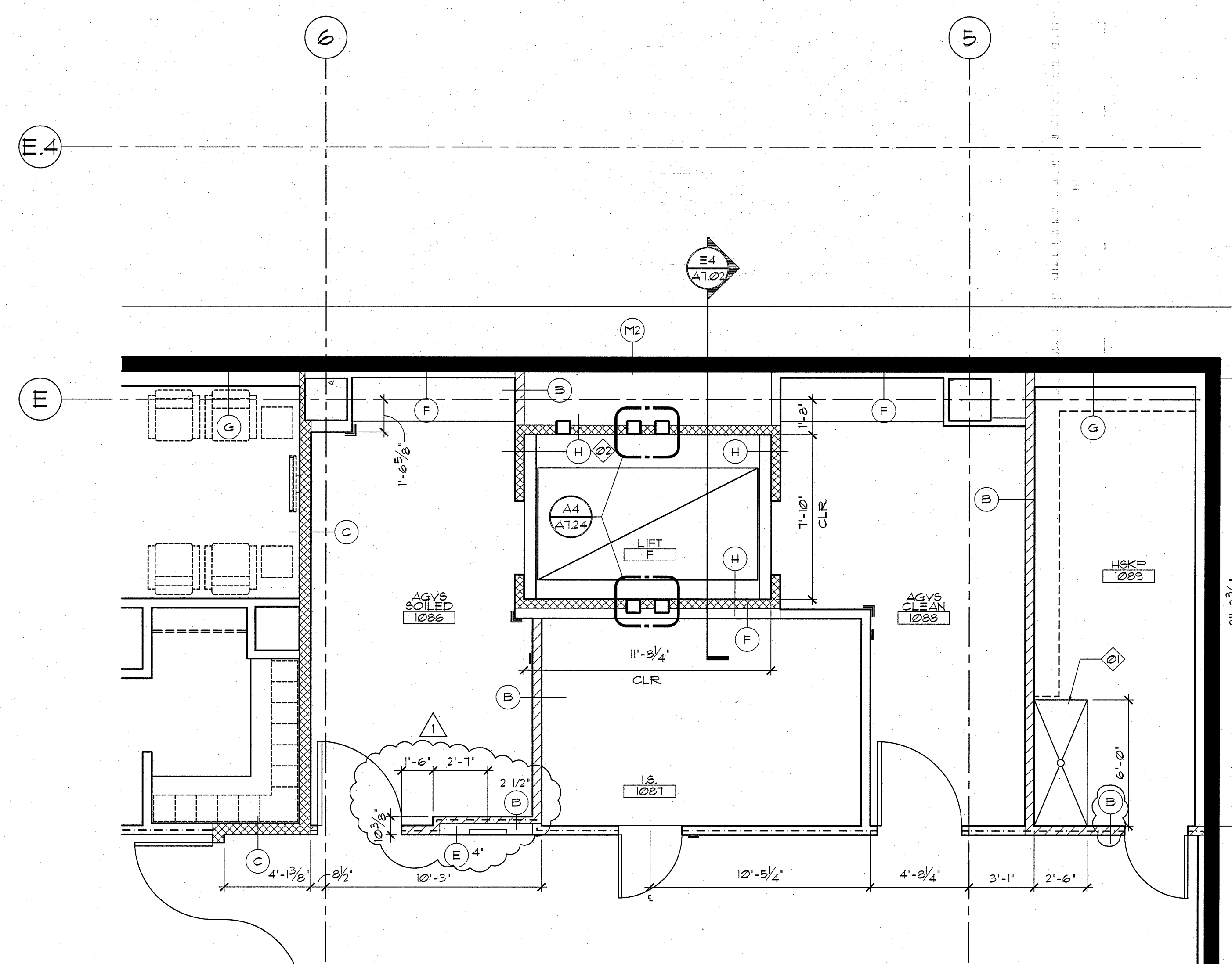
C4 LIFT F PLAN @ FIRST FLOOR 1/4" = 1'-0"
