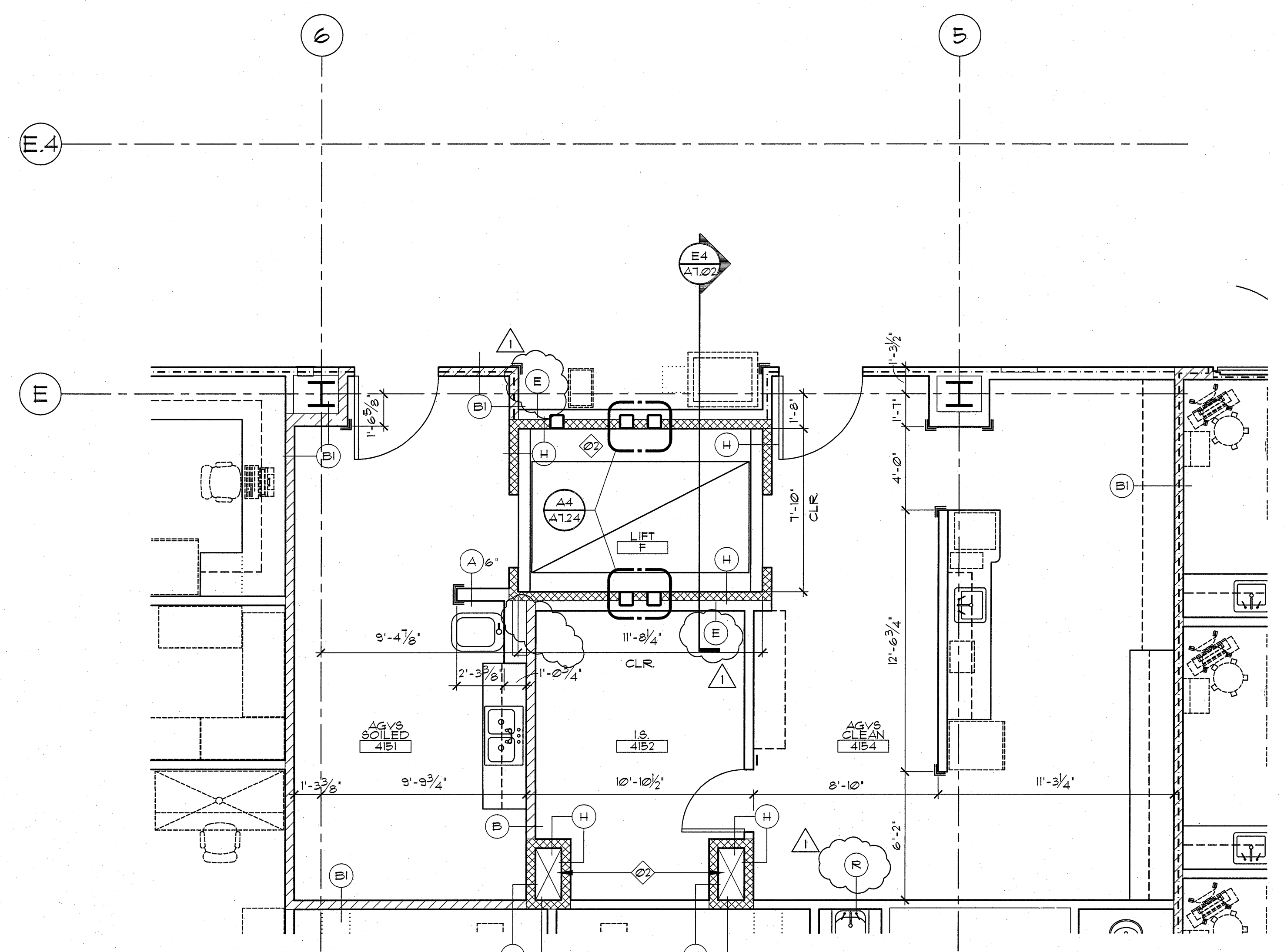
E1 LIFT F PLAN @ FOURTH FLOOR 1/4" = 1'-0"
