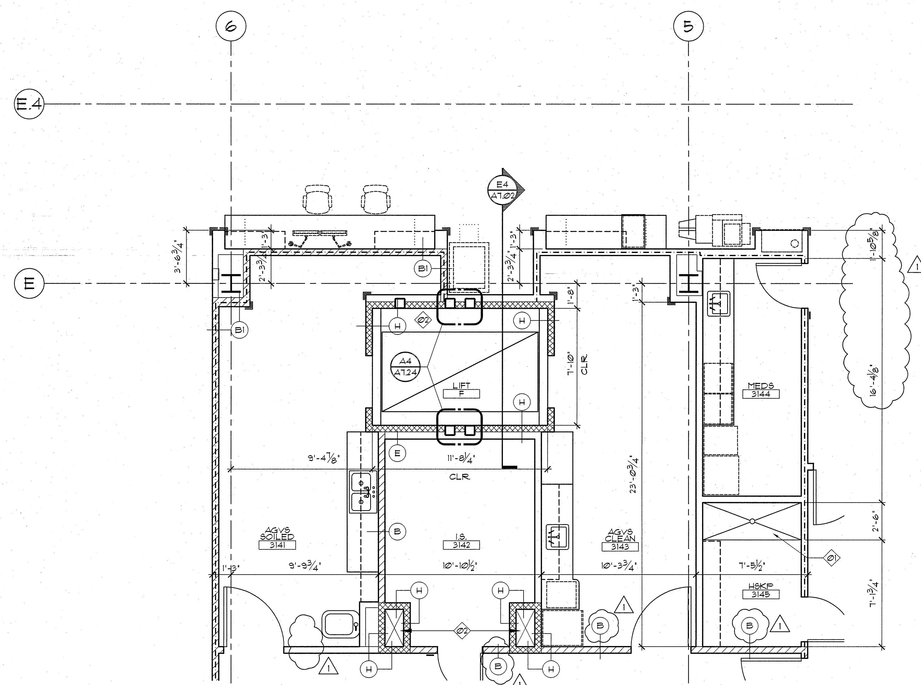
C1 LIFT F PLAN @ THIRD FLOOR 1/4" = 1'-0"
