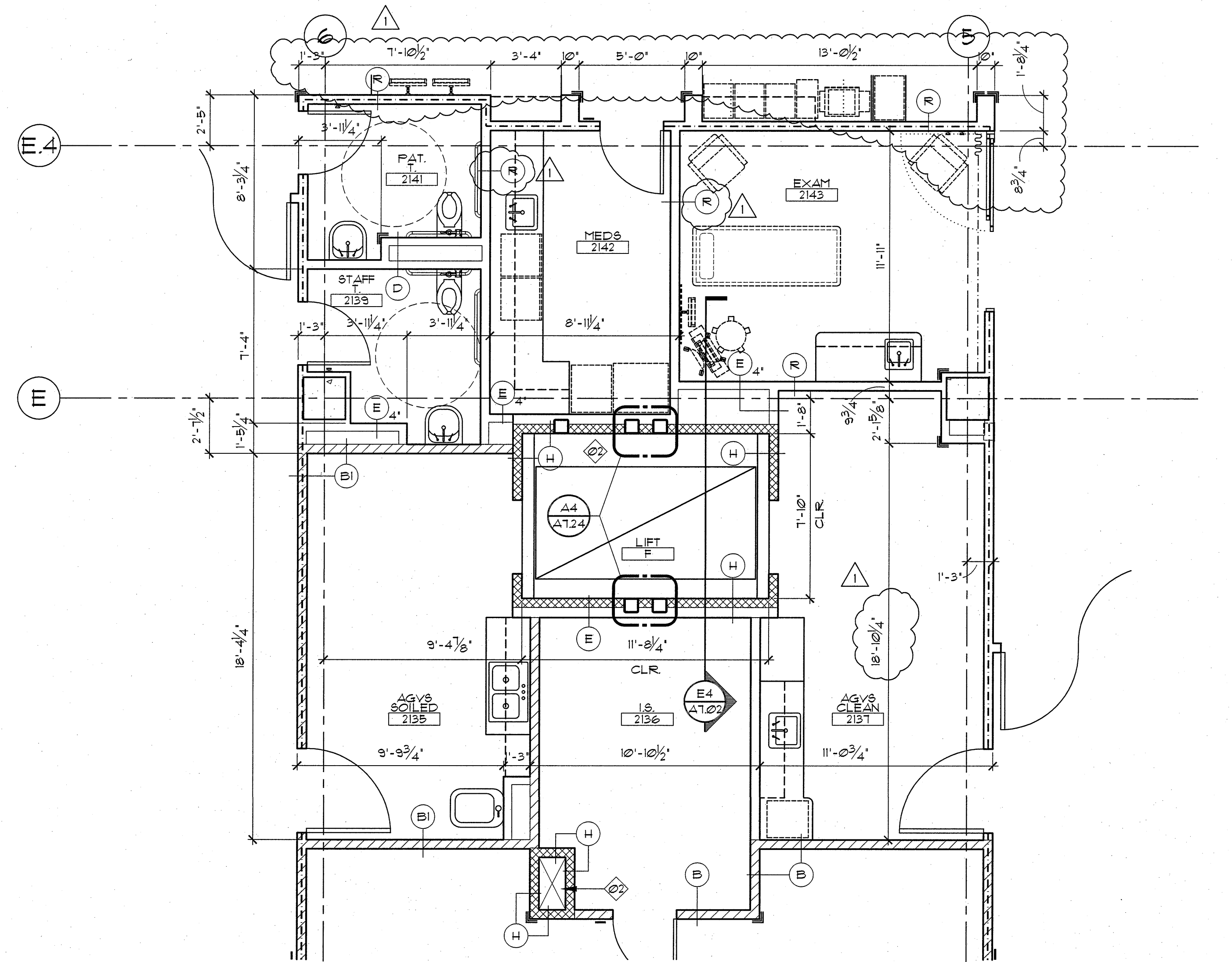
E4 LIFT F PLAN @ SECOND FLOOR 1/4" = 1'-0"
