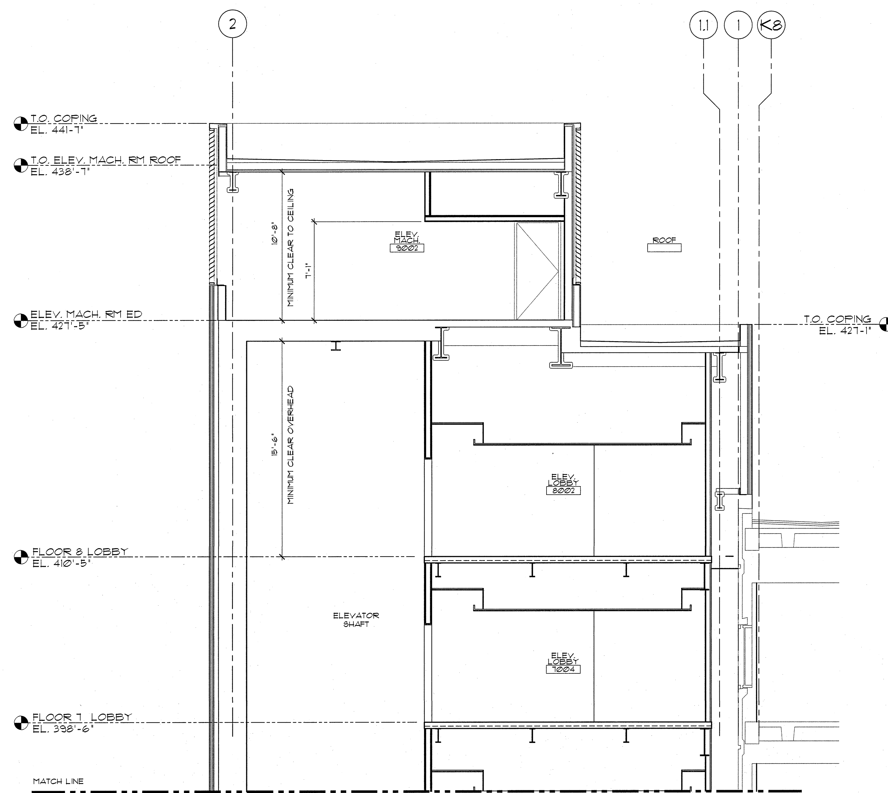
B1 ELEVATOR 19 & 20 SECTION - NOT USED 1/4" = 1'-0"
