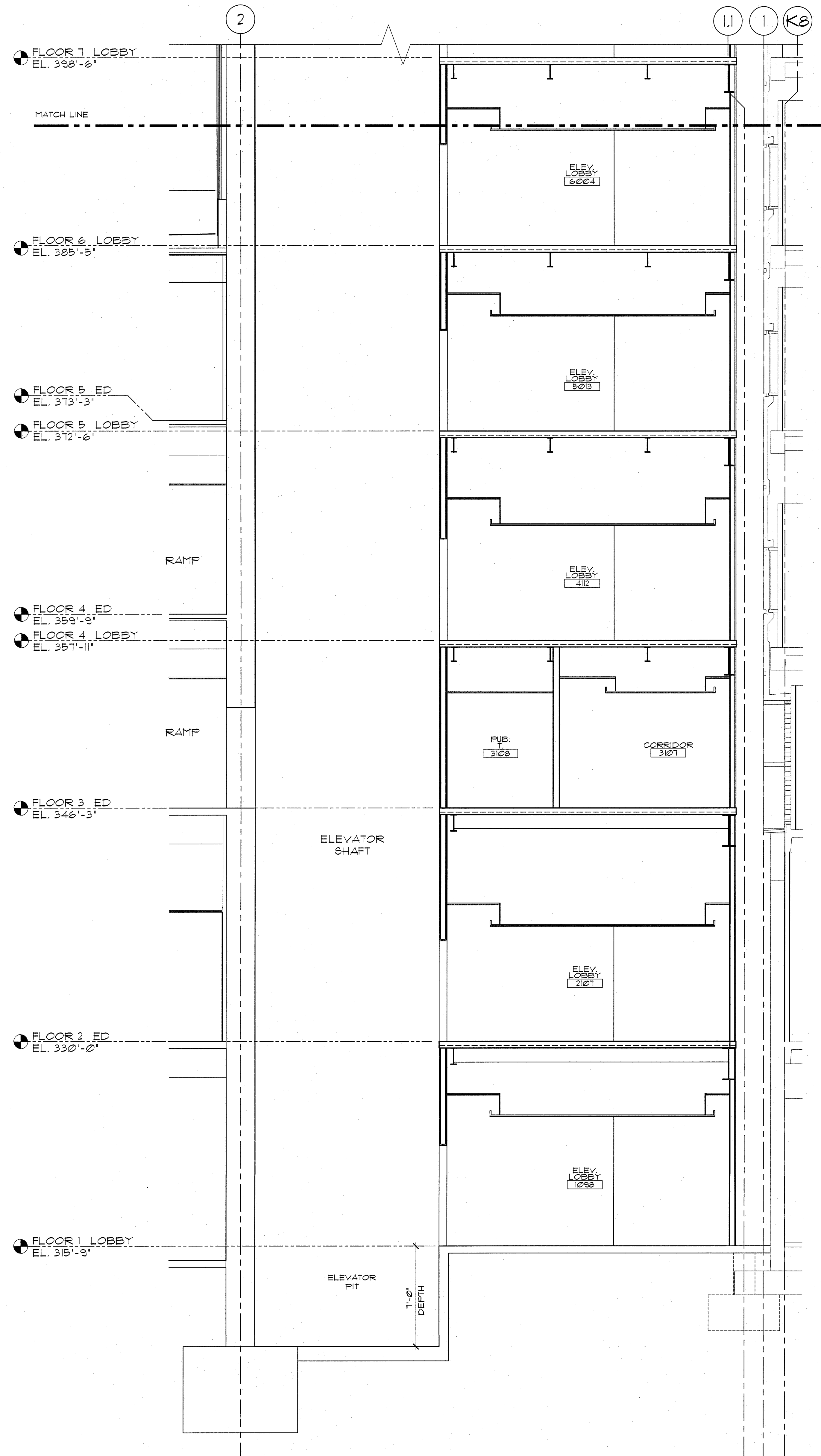
E4 ELEVATOR 19 & 20 SECTION 1/4" = 1'-0"
