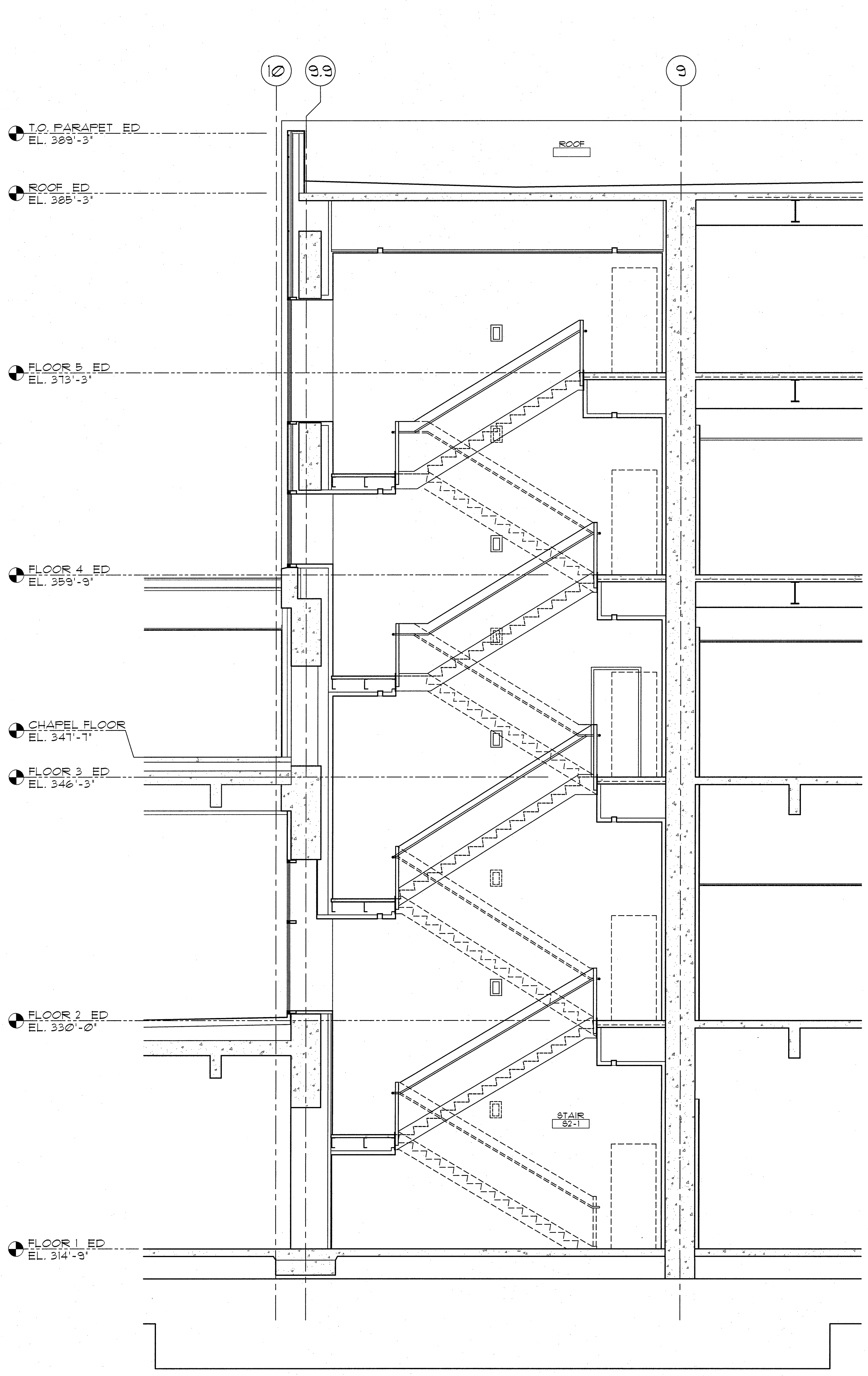
E4 STAIR #2 SECTION 1/4" = 1'-0"
