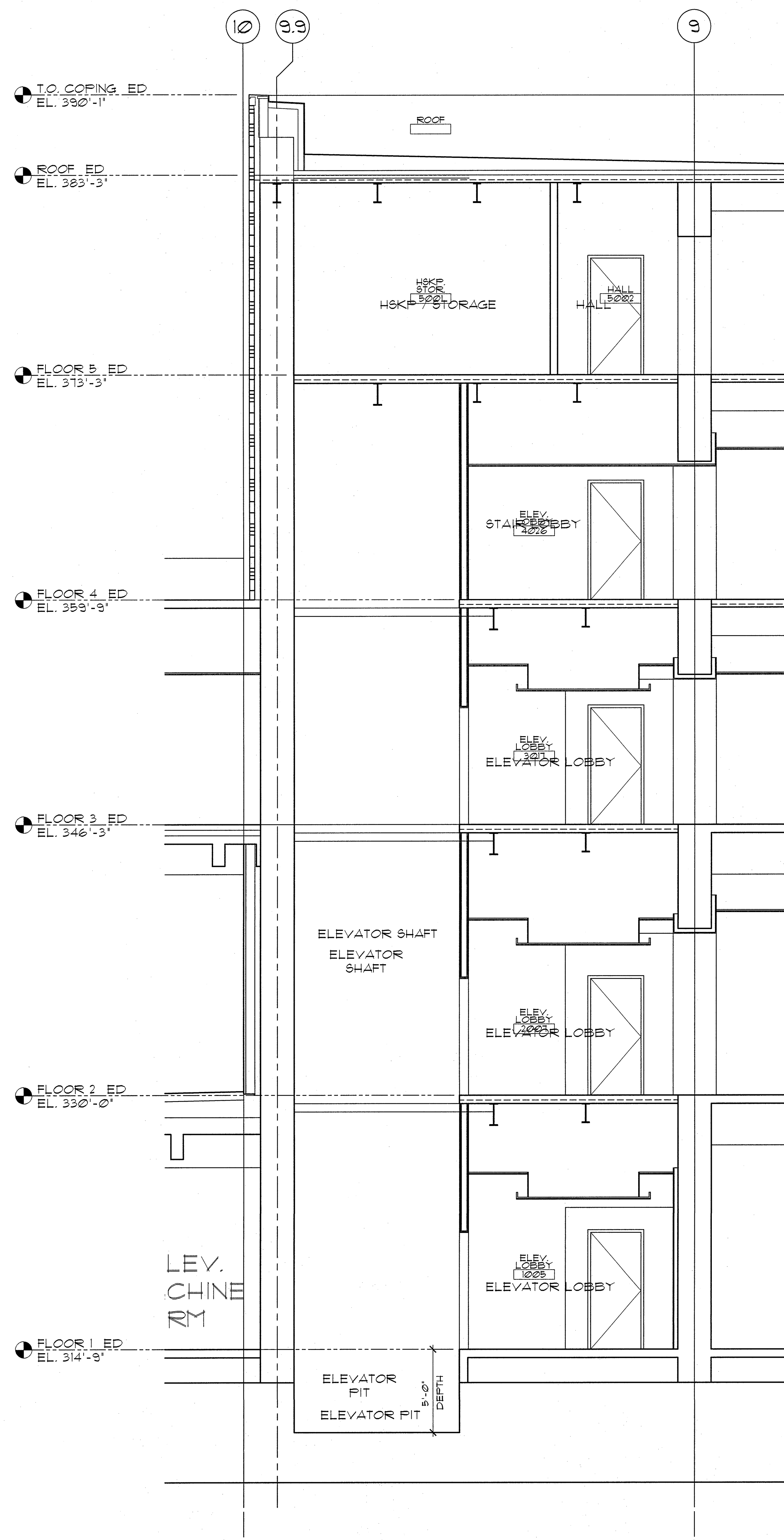
E1 ELEVATOR 21 & 22 SECTION 1/4" = 1'-0"
