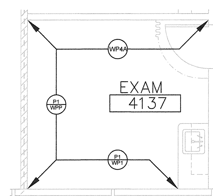
EXAM ROOM TYPICAL SCALE: 1/8" = 1'-0"
