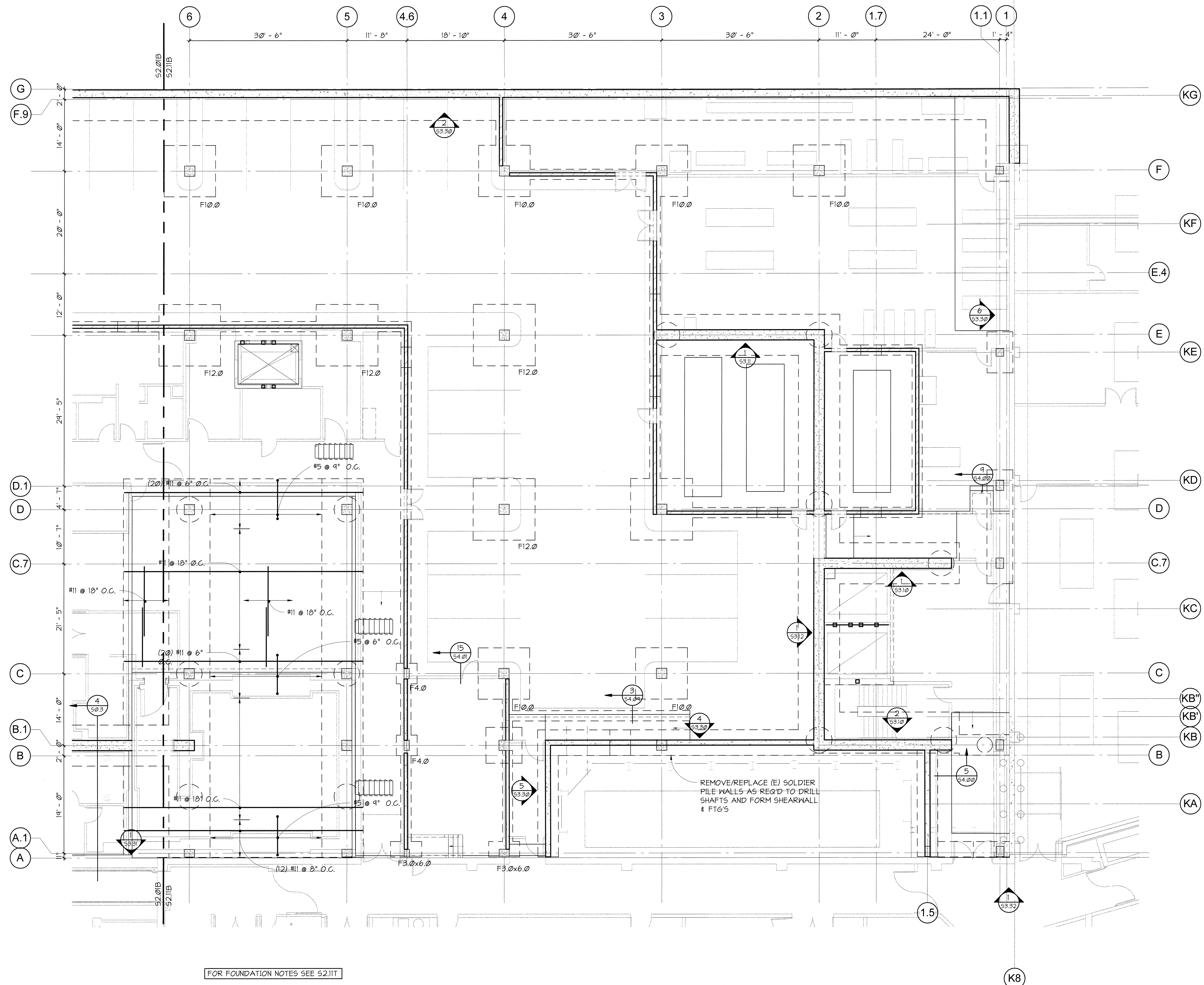
1 FOUNDATION BOTTOM REINFORCING PLAN - NORTH S2.11B 1/8" = 1'-0"
