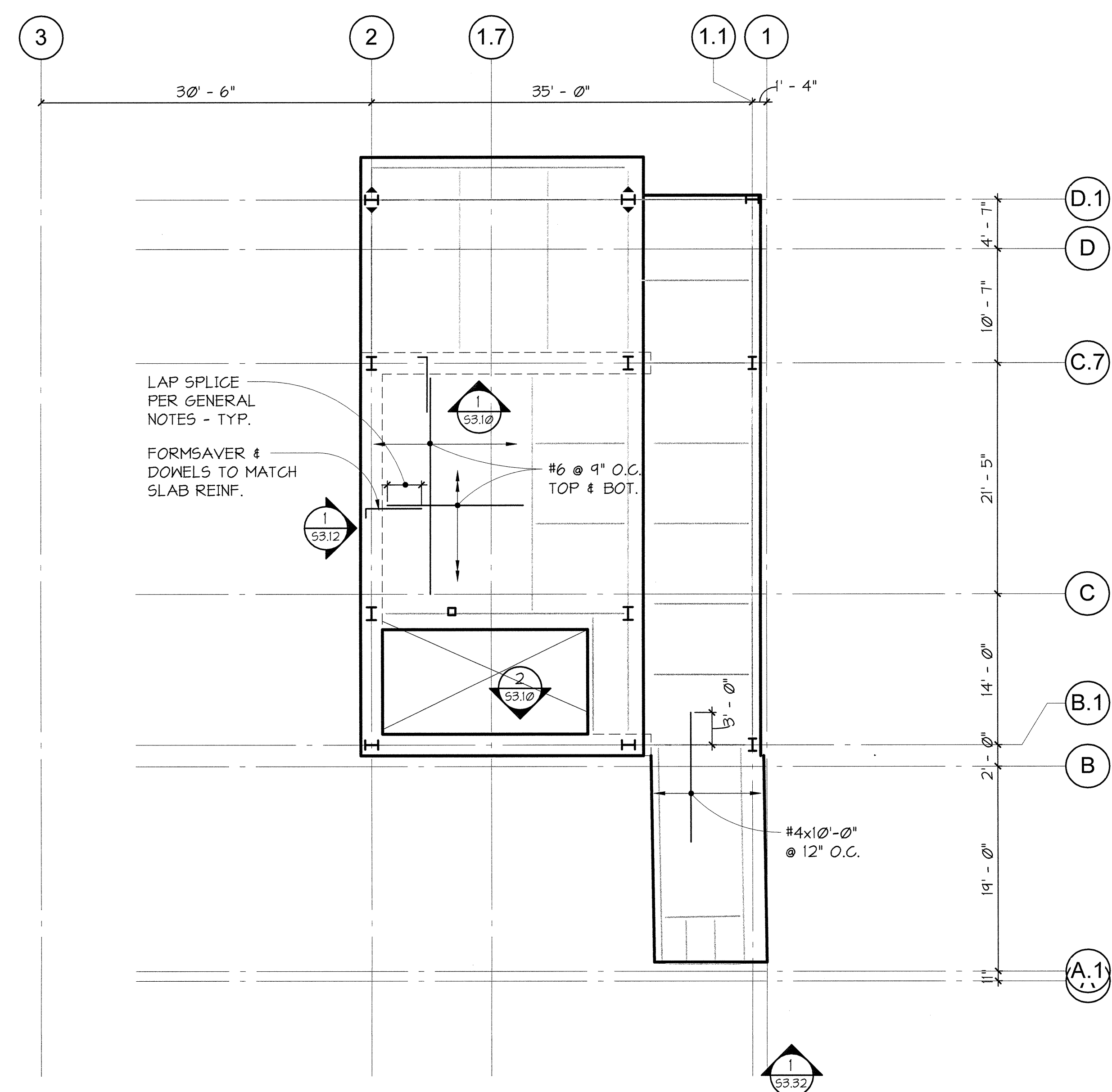
1 NINTH FLOOR SLAB PLAN - NORTH 52.146 1/8" = 1'-0"
