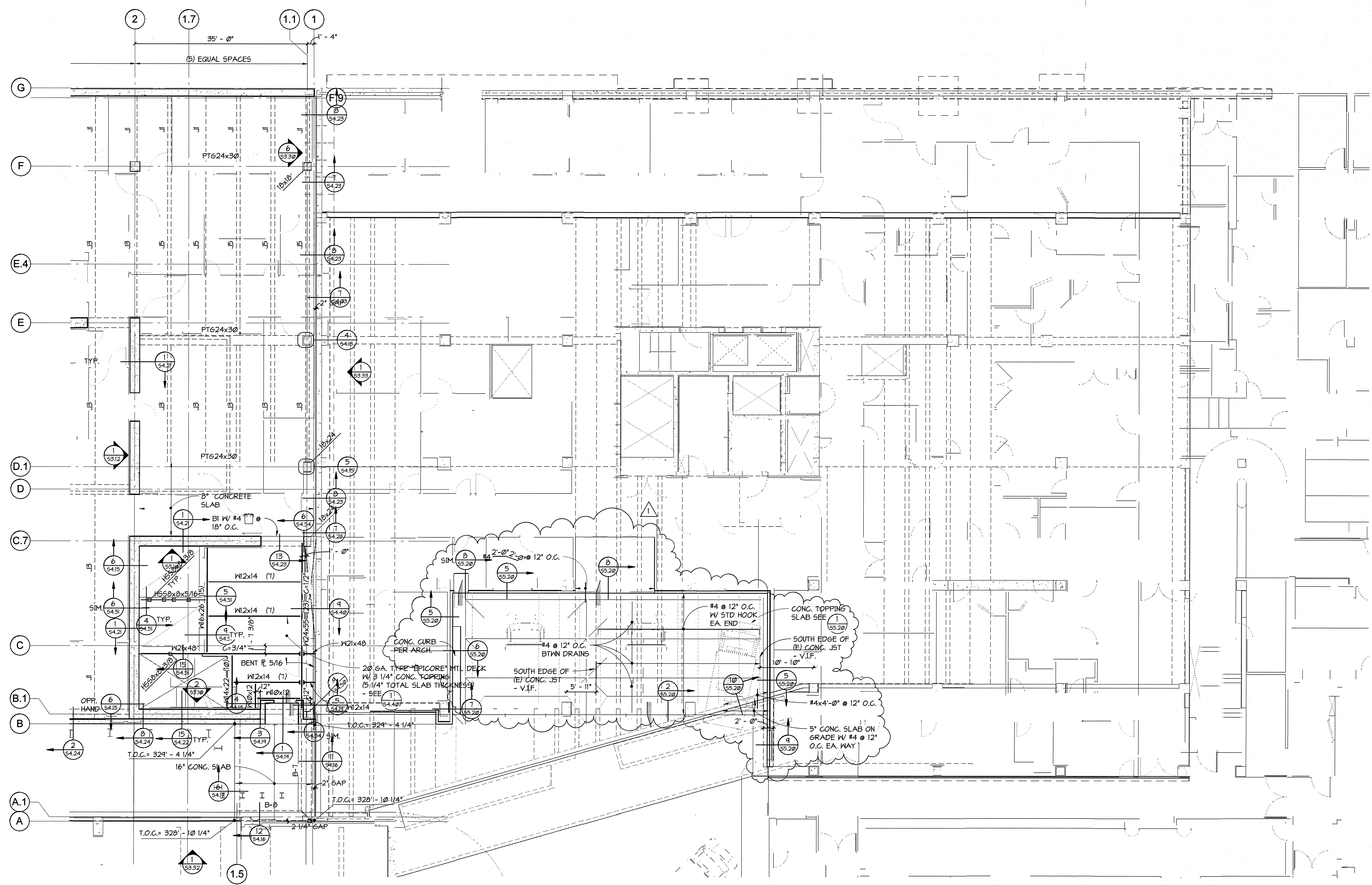
1 SECOND FLOOR FRAMING PLAN 52.22 1/8" = 1'-0"
