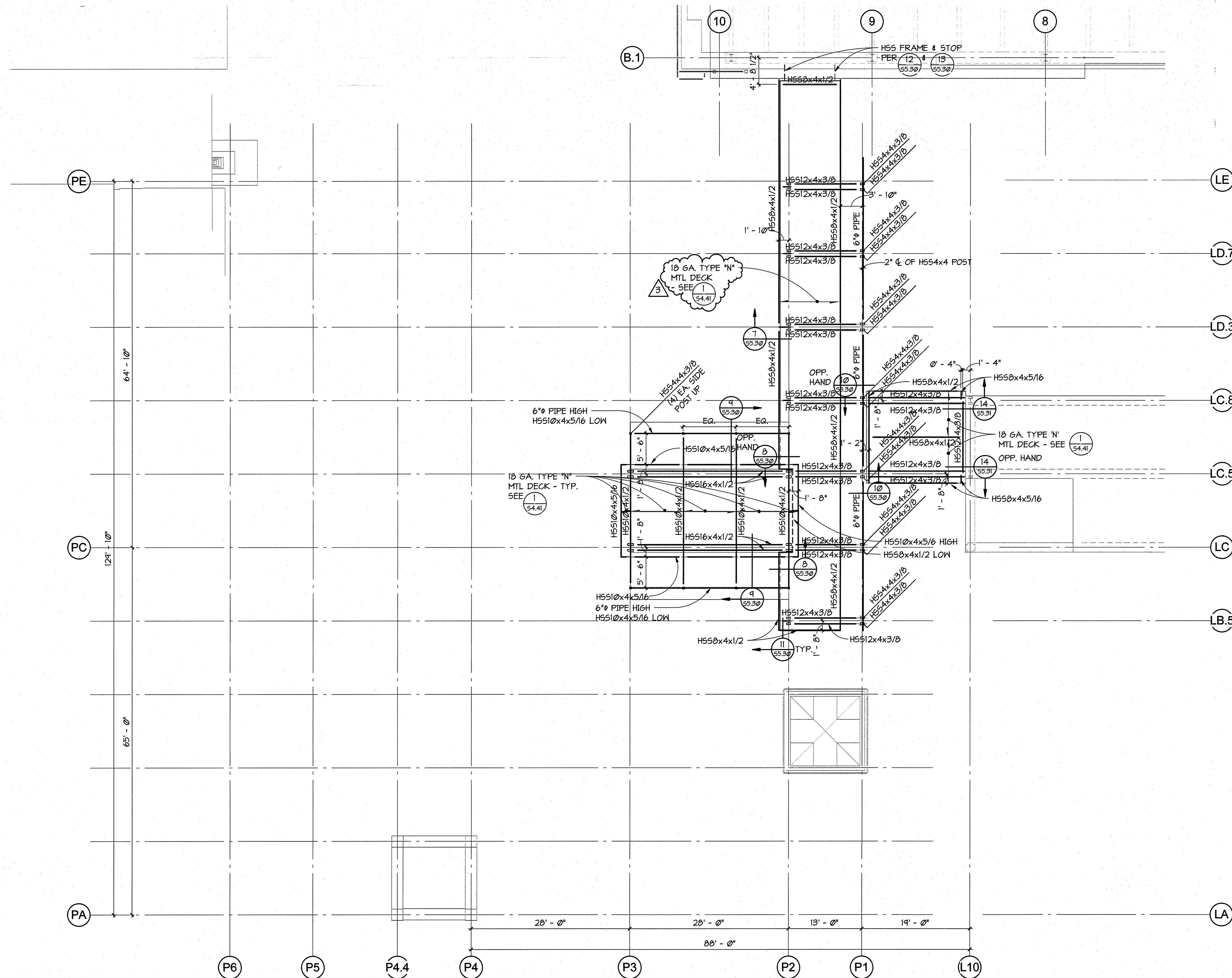
1 L-WING PLAZA CANOPY FRAMING 1/8" = 1'-0"
