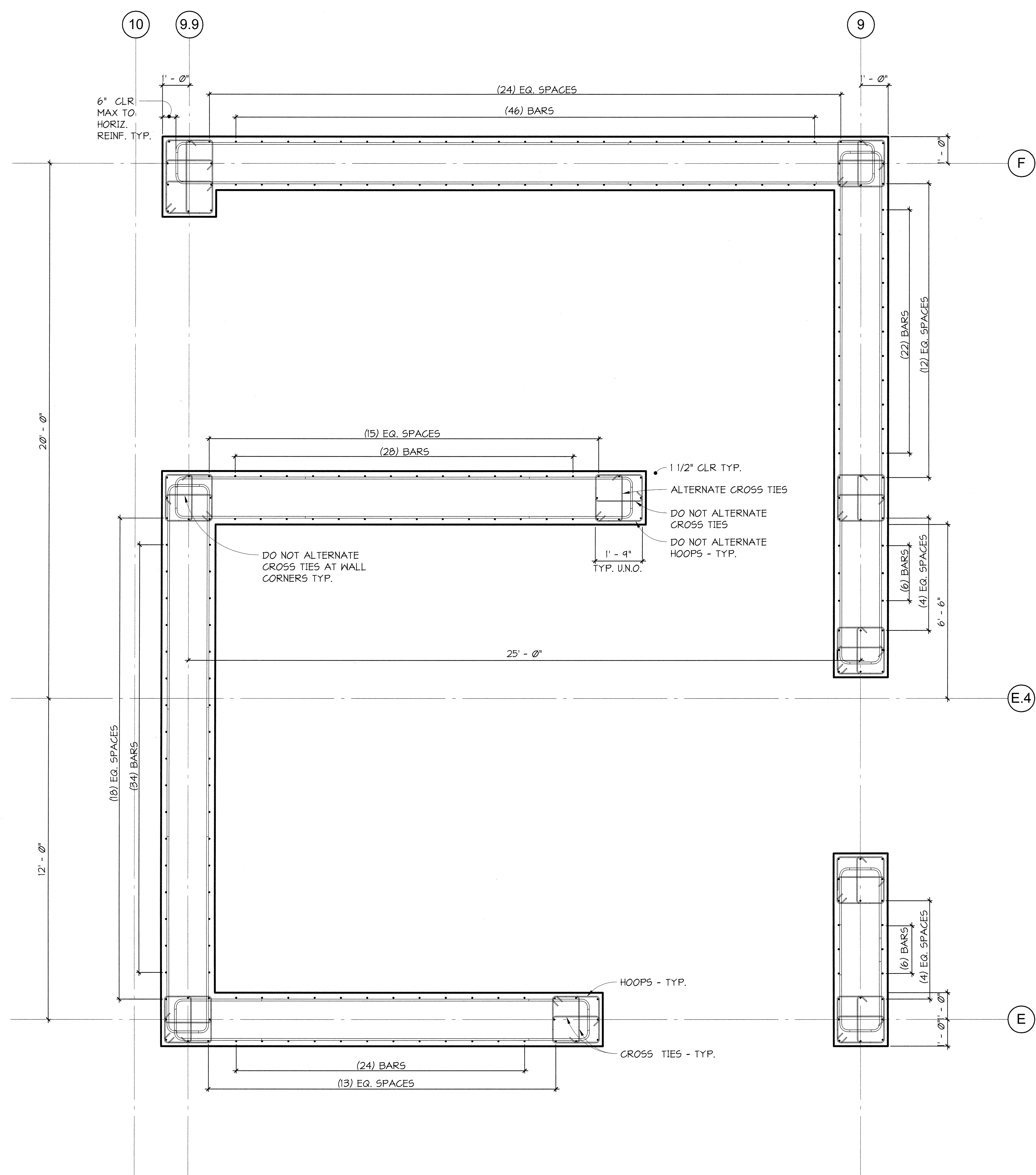
1 PLAN SECTION 1/2" = 1'-0"
