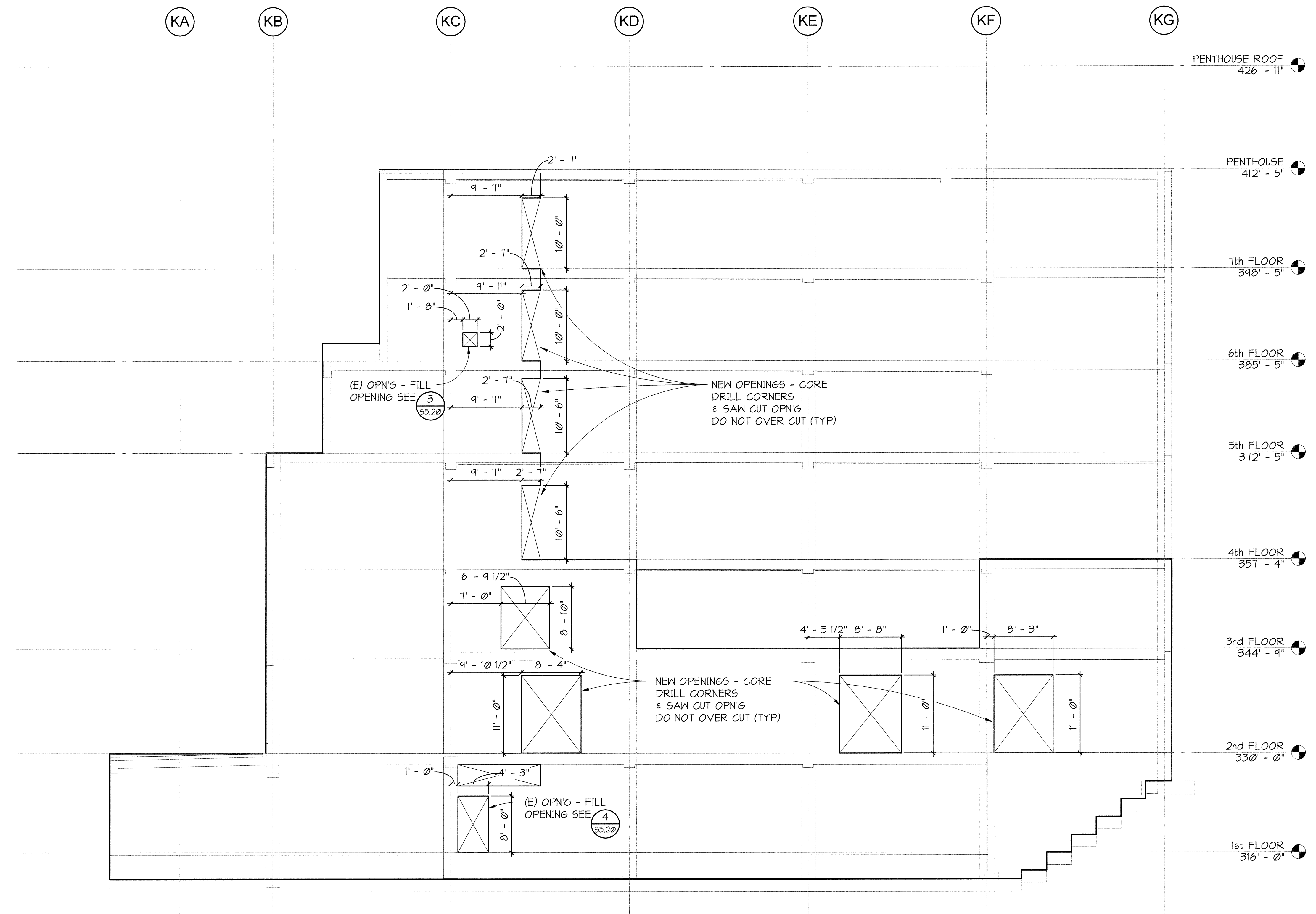
1 WALL ELEVATION K-WING 55.33 1/8" = 1'-0"
