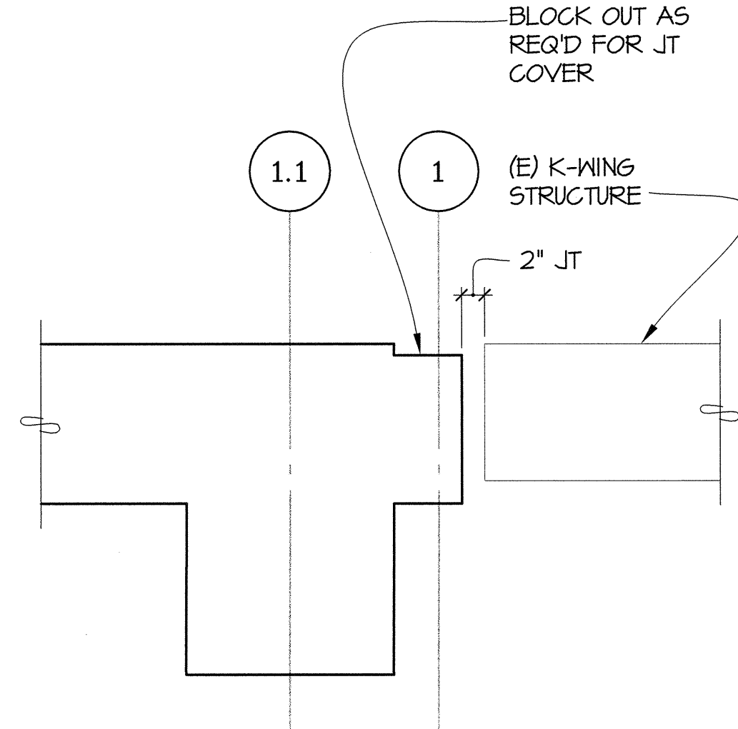
11 SECTION S4.16 1"=1'-0"
