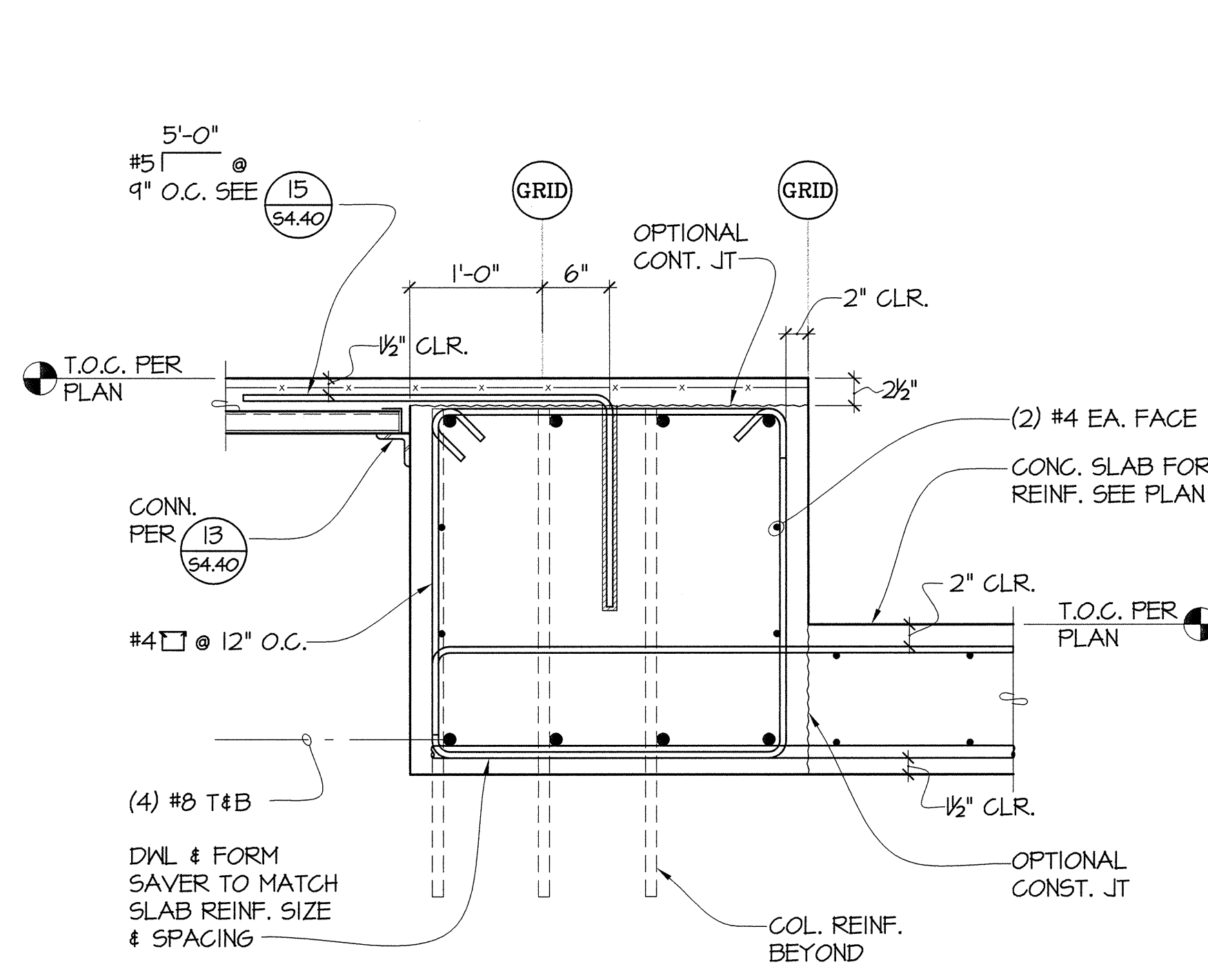
2 SECTION S4.16 1"=1'-0"
