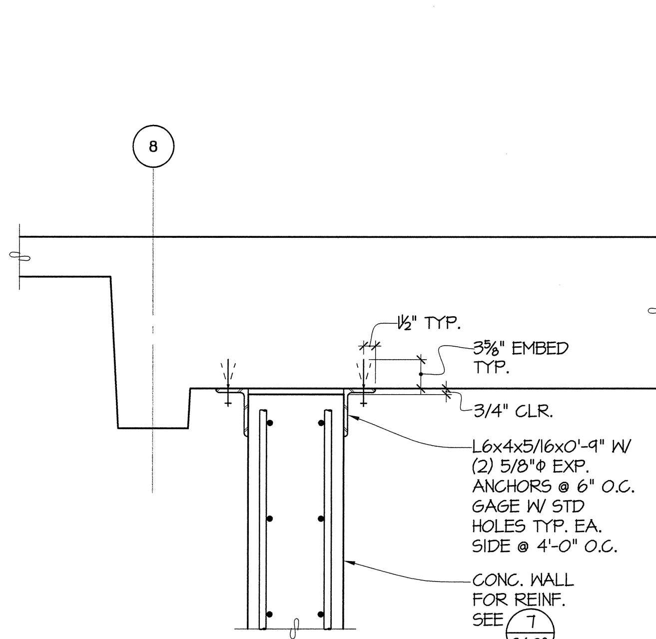
5 SECTION S4.16 1"=1'-0"
