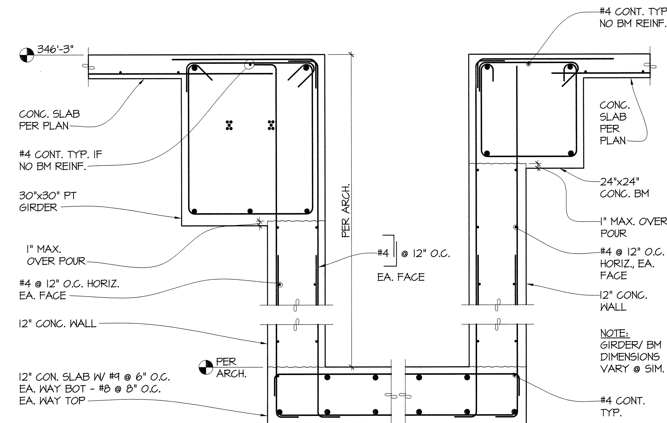
3 SECTION S4.16 1"=1'-0"
