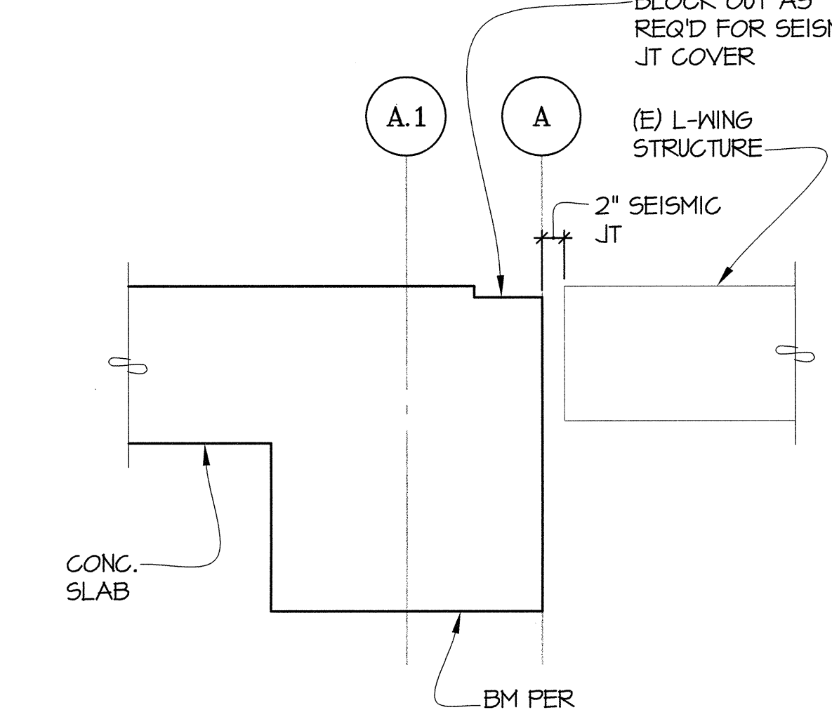
12 SECTION S4.16 1"=1'-0"
