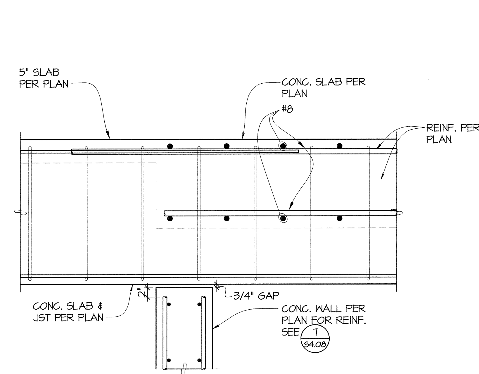
8 SECTION S4.16 1"=1'-0"
