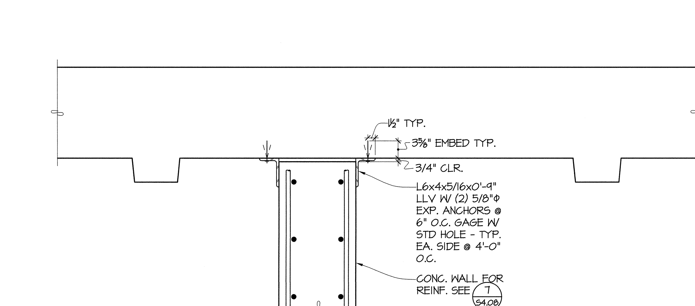
10 SECTION S4.16 1"=1'-0"
