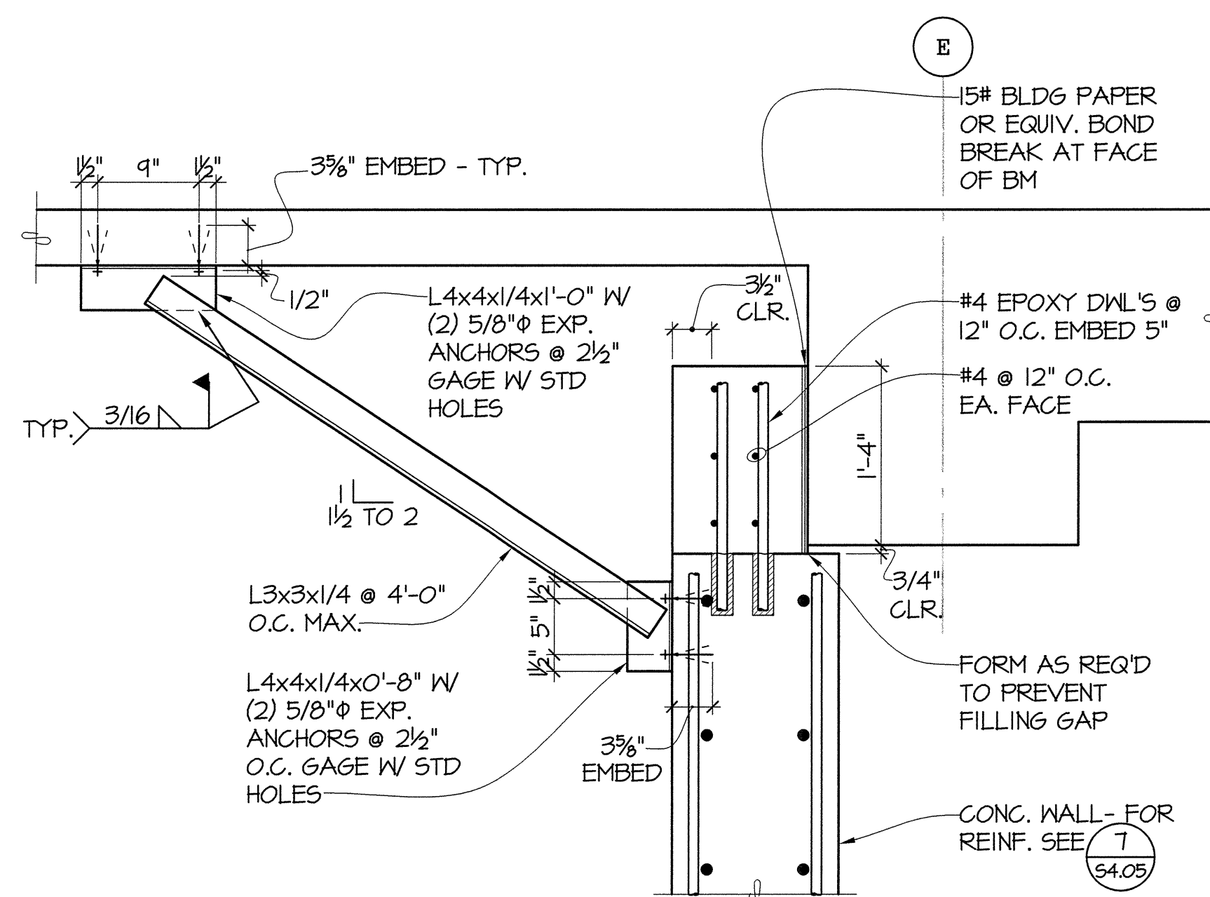
6 SECTION S4.16 1"=1'-0"
