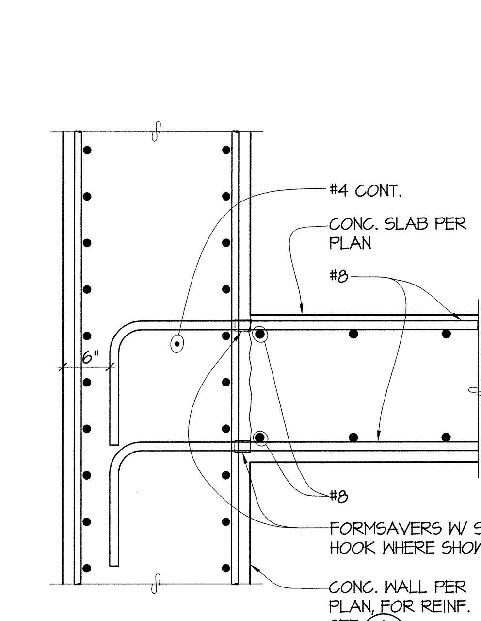
7 SECTION S4.16 1"=1'-0"
