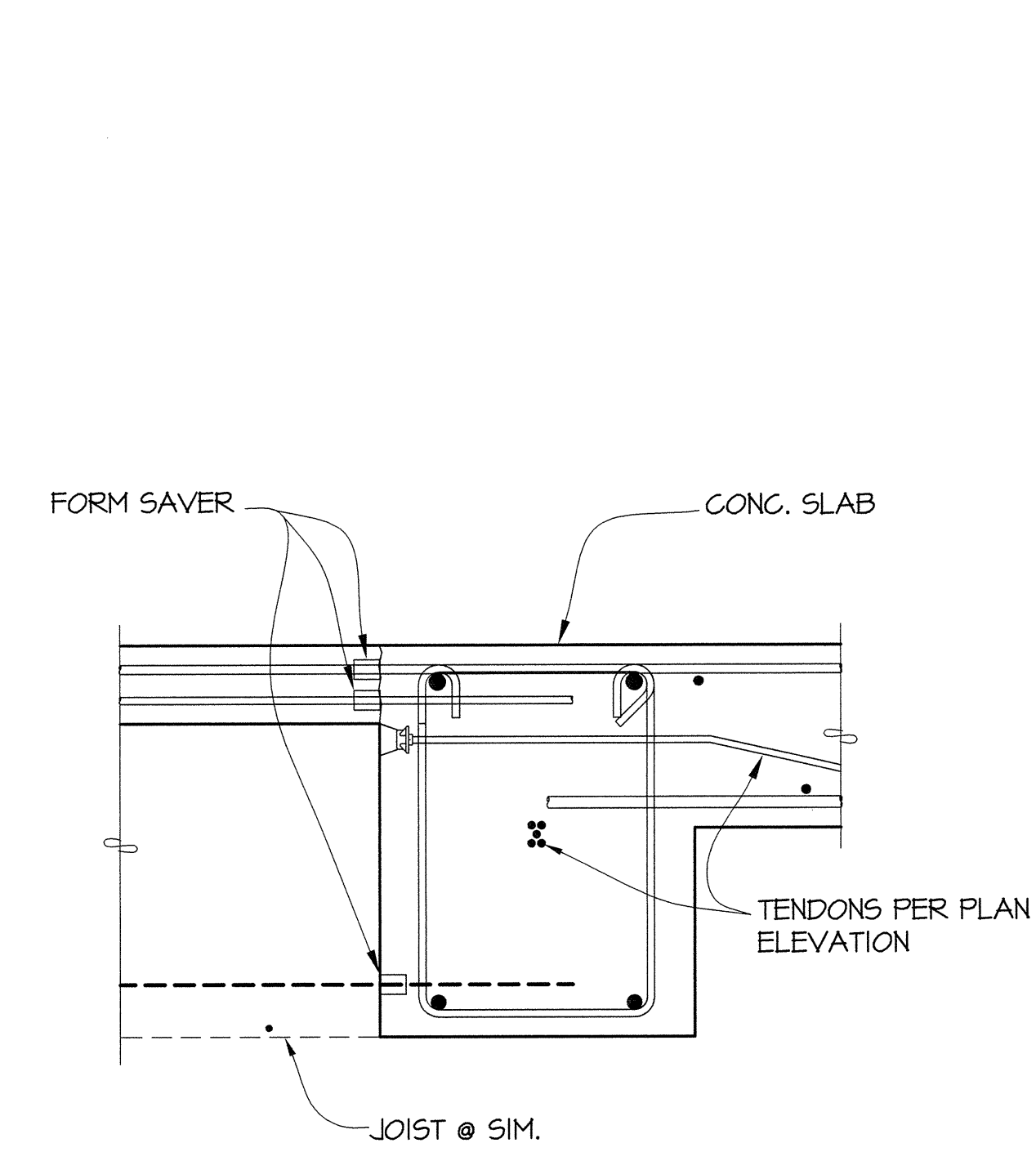
4 SECTION S4.16 1"=1'-0"
