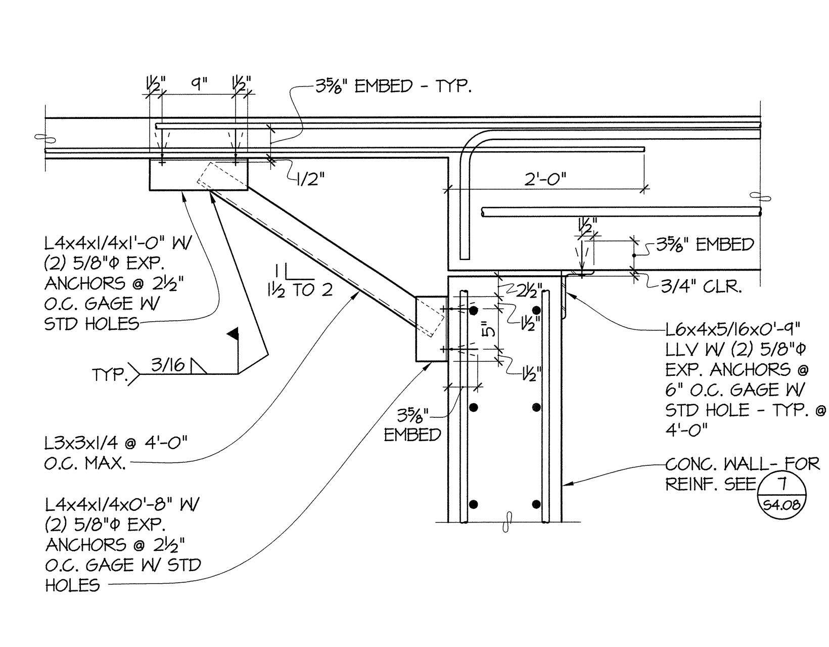
9 SECTION S4.16 1"=1'-0"
