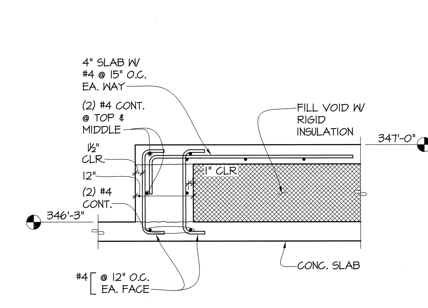
13 SECTION S4.16 1"=1'-0"
