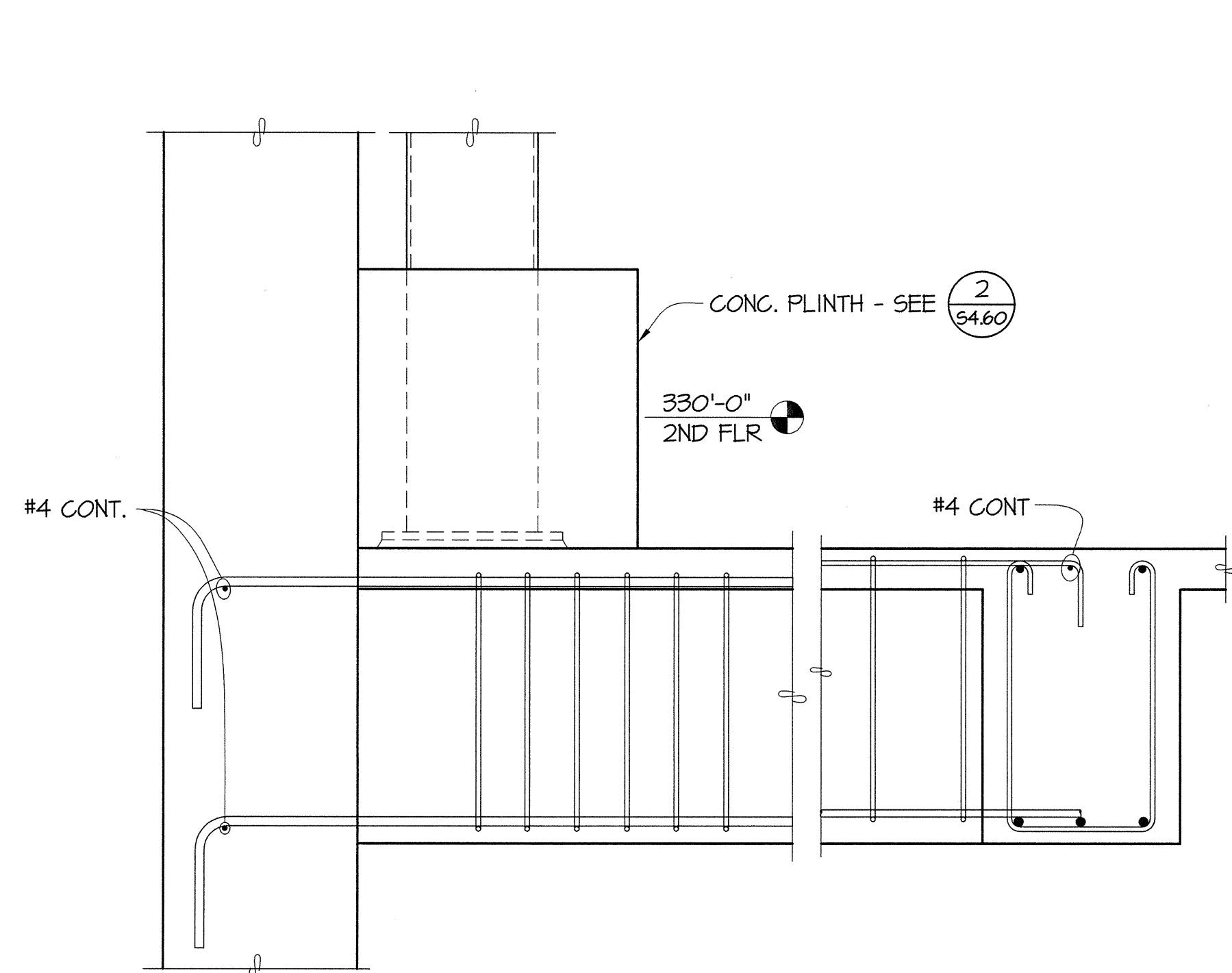
1 SECTION S4.16 3/4"=1'-0"
