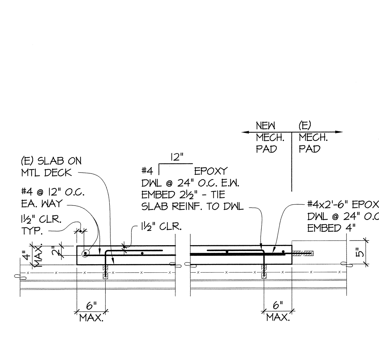
8 SECTION 55.40 1"=1'-0"
