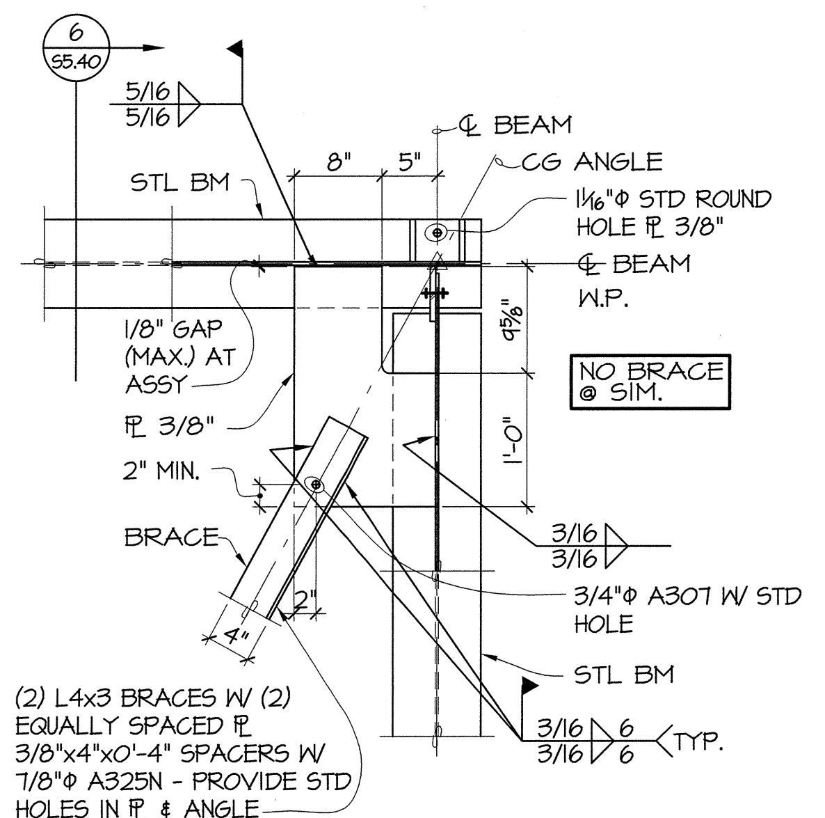
5 DETAIL 55.40 1"=1'-0"
