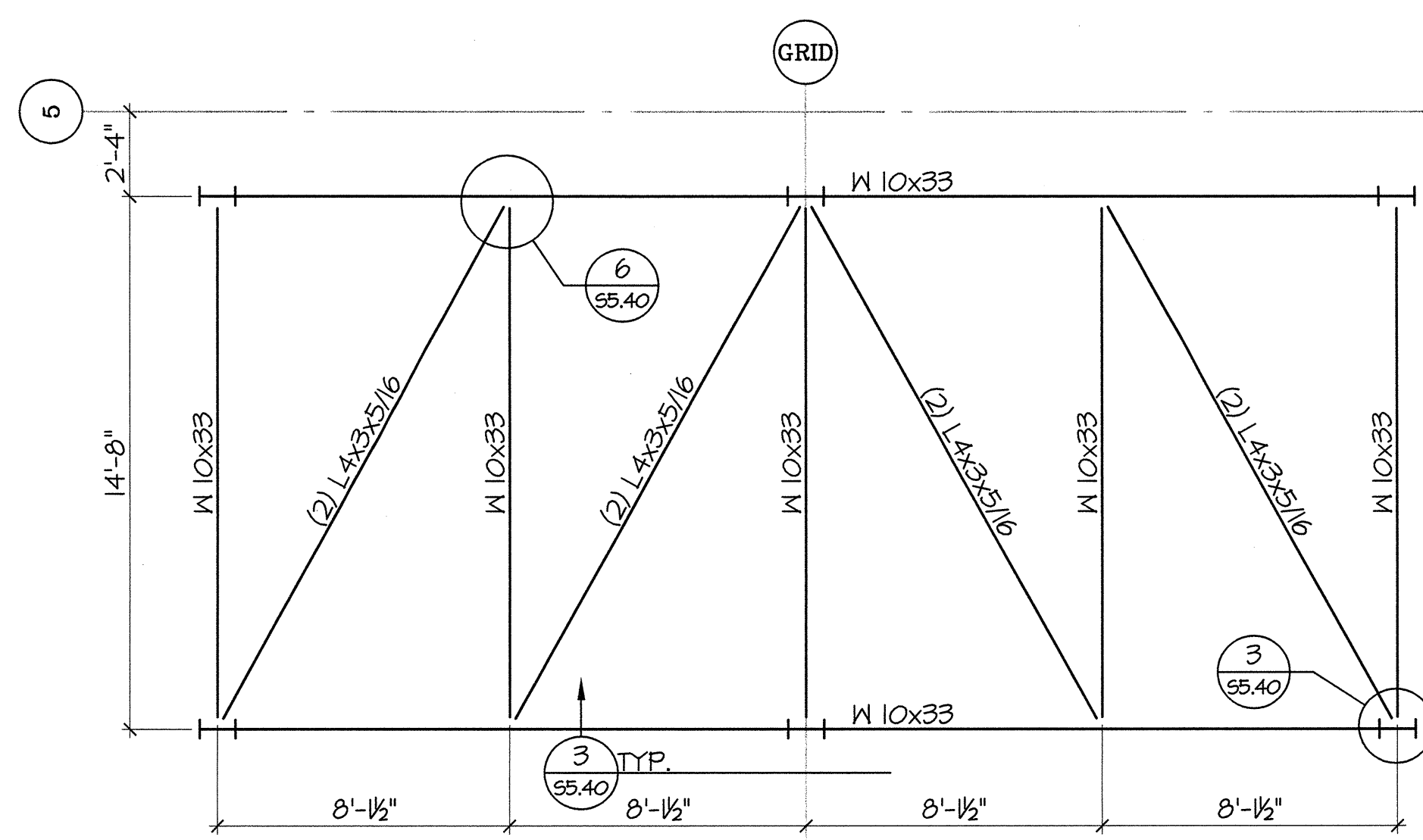
1 PLAN 55.40 1/4"=1'-0"
