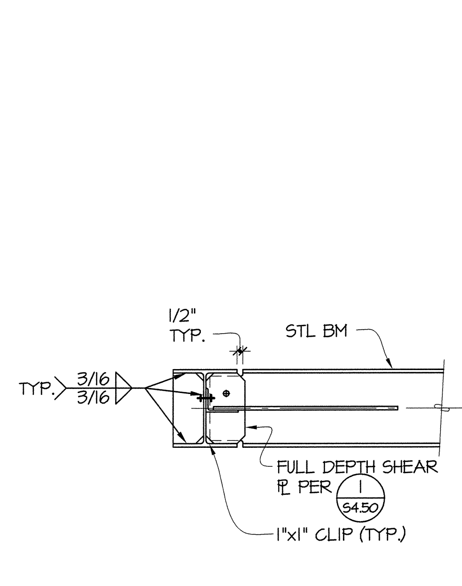
6 DETAIL 55.40 1"=1'-0"
