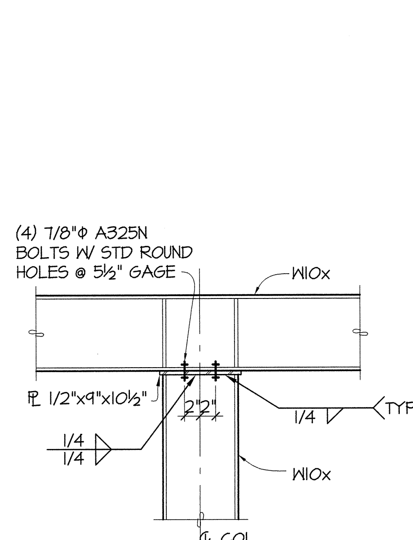
3 SECTION 55.40 1"=1'-0"
