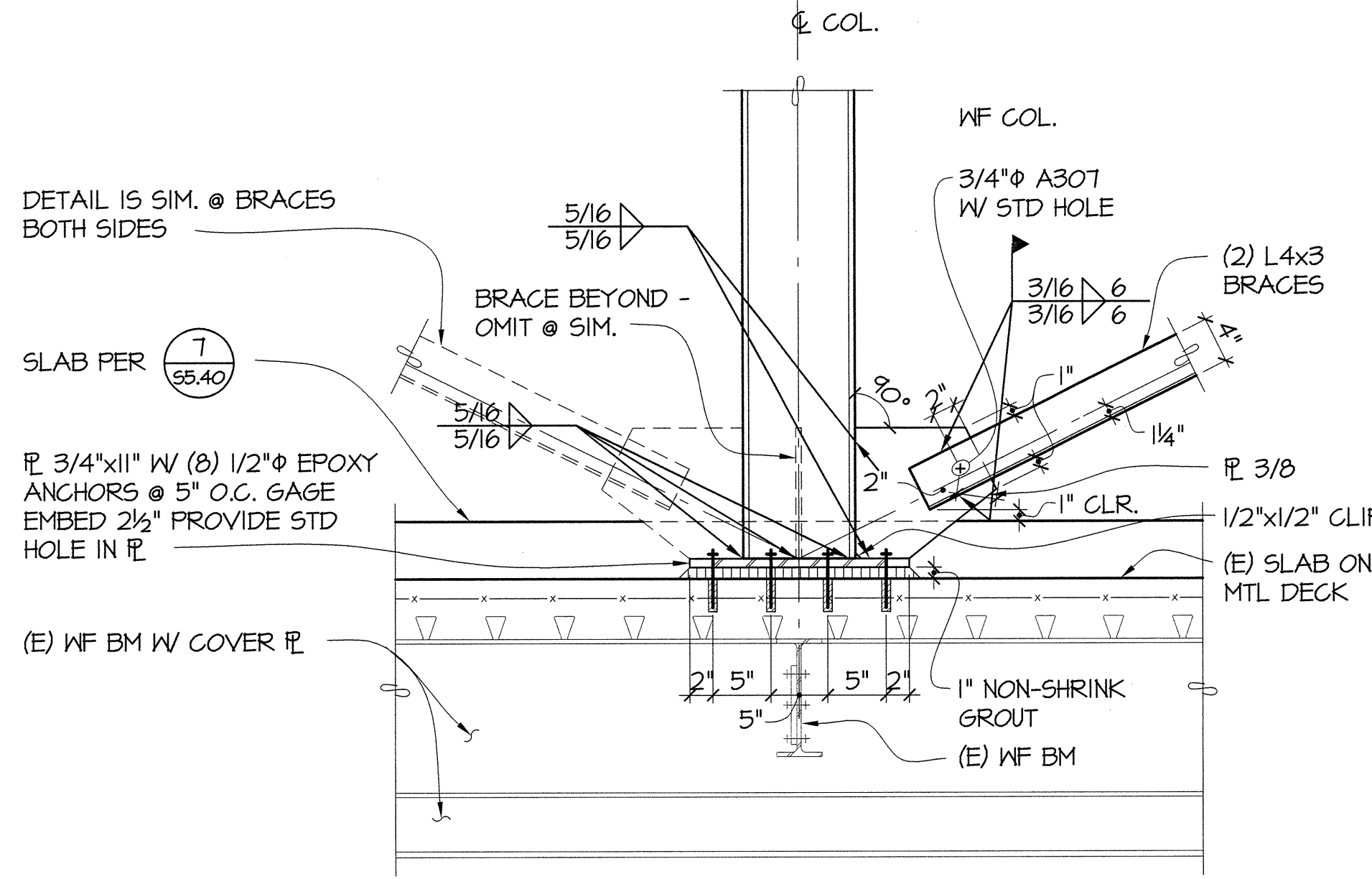
2 SECTION 55.40 1"=1'-0"
