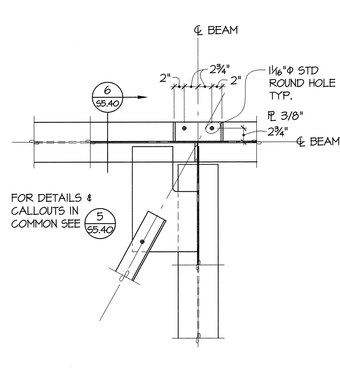
7 DETAIL 55.40 1"=1'-0"
