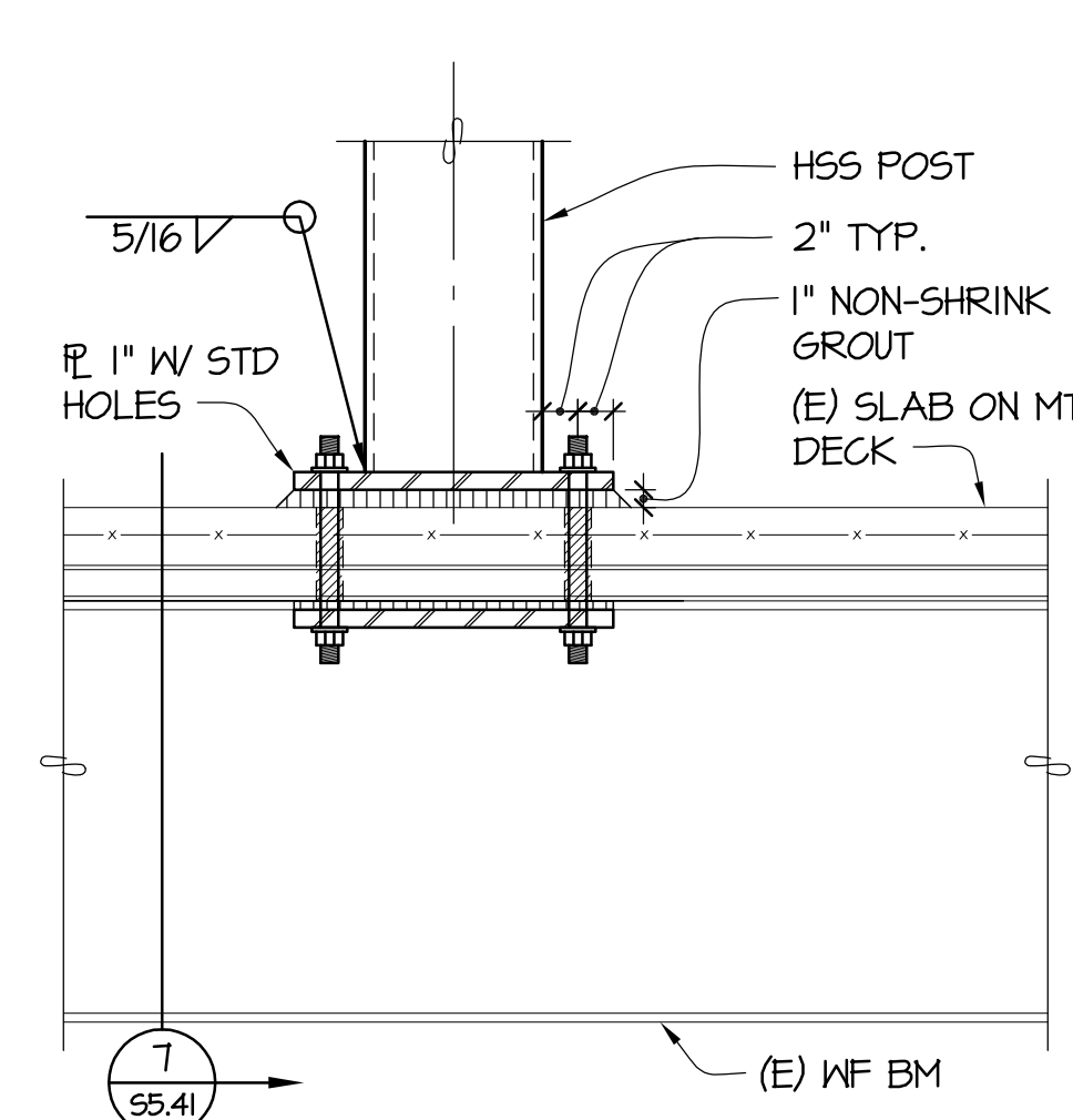
8 SECTION 55.41 1"=1'-0"
