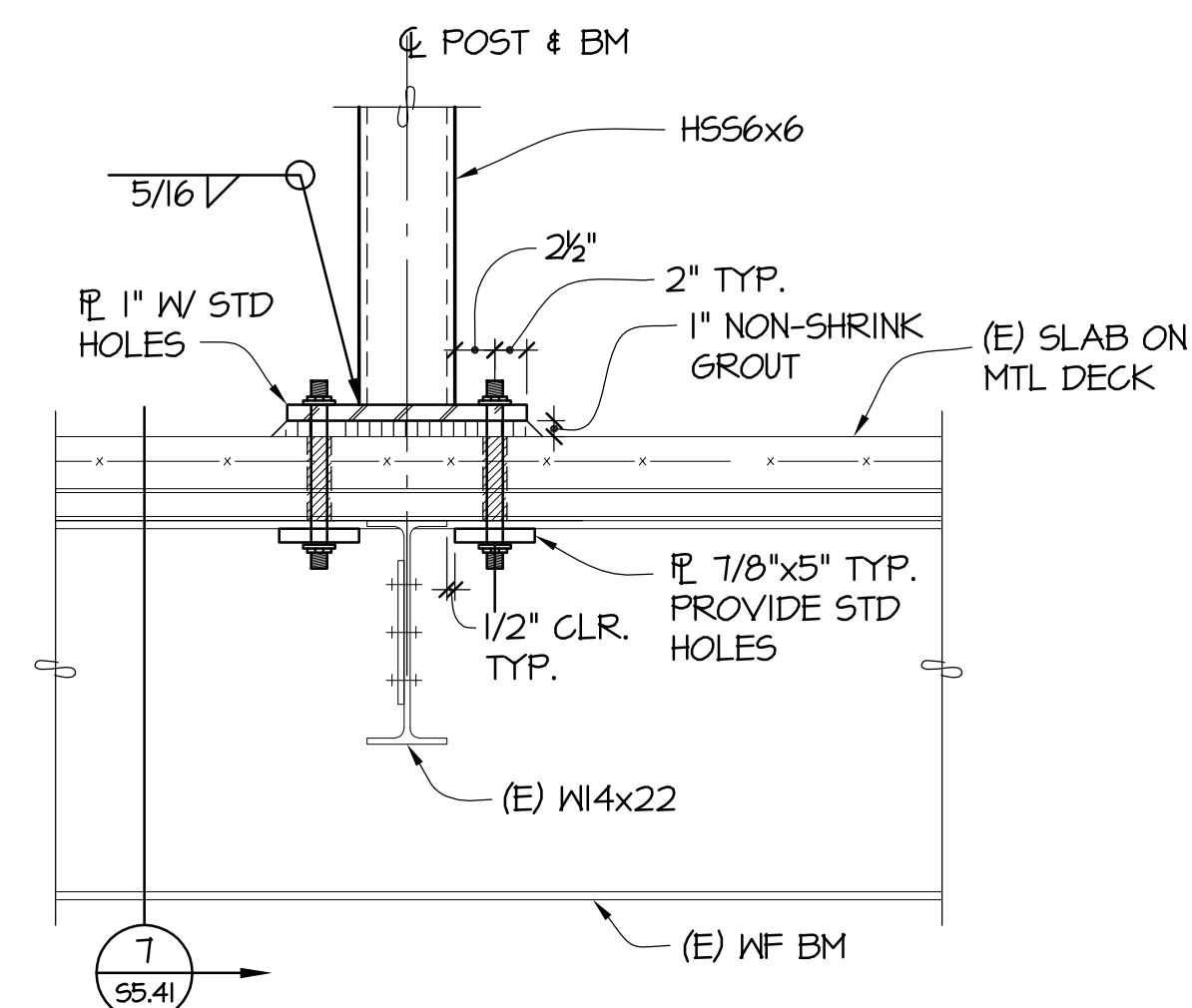
5 SECTION 55.41 1"=1'-0"
