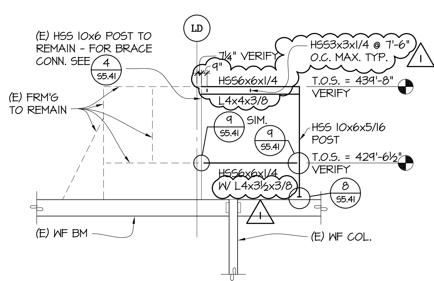
2 ELEVATION 55.41 1/8"=1'-0"
