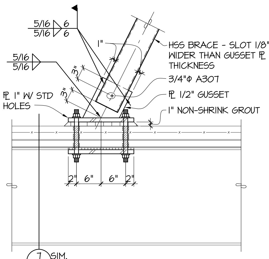
6 SECTION 55.41 1"=1'-0"
