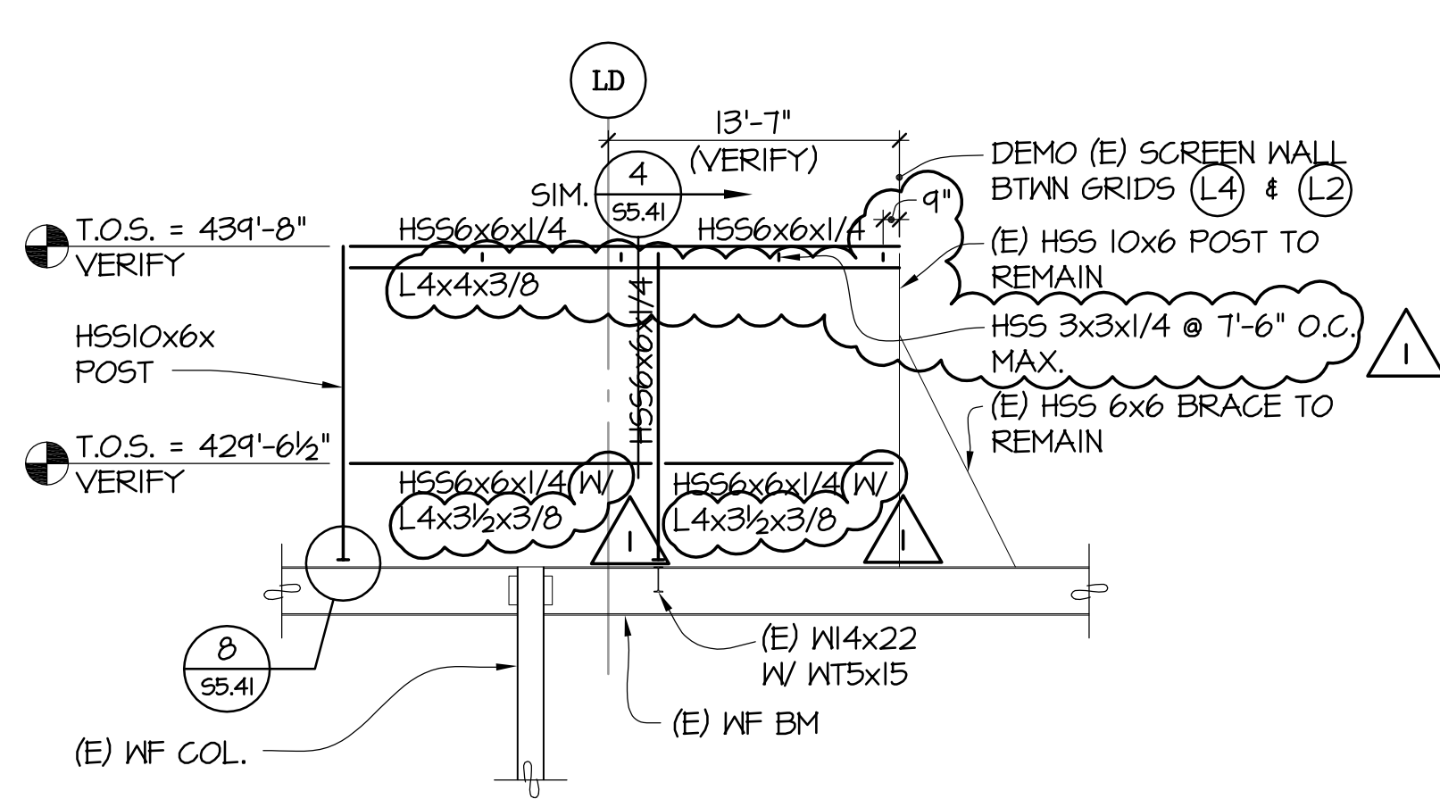
3 ELEVATION 55.41 1/8"=1'-0"
