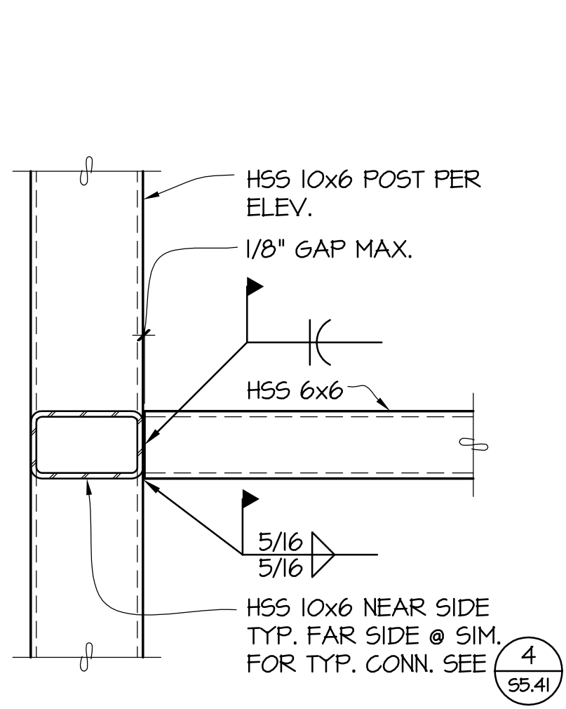
9 SECTION 55.41 1"=1'-0"
