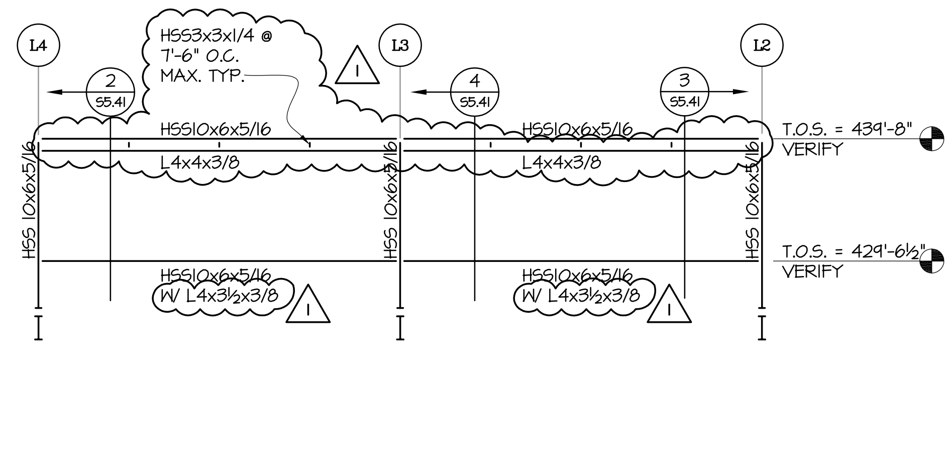
1 ELEVATION 55.41 1/8"=1'-0"
