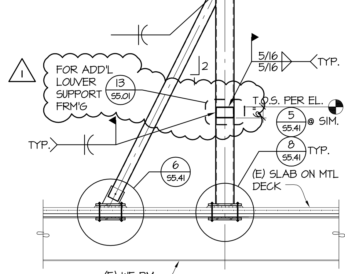
4 DETAIL 55.41 3/8"=1'-0"
