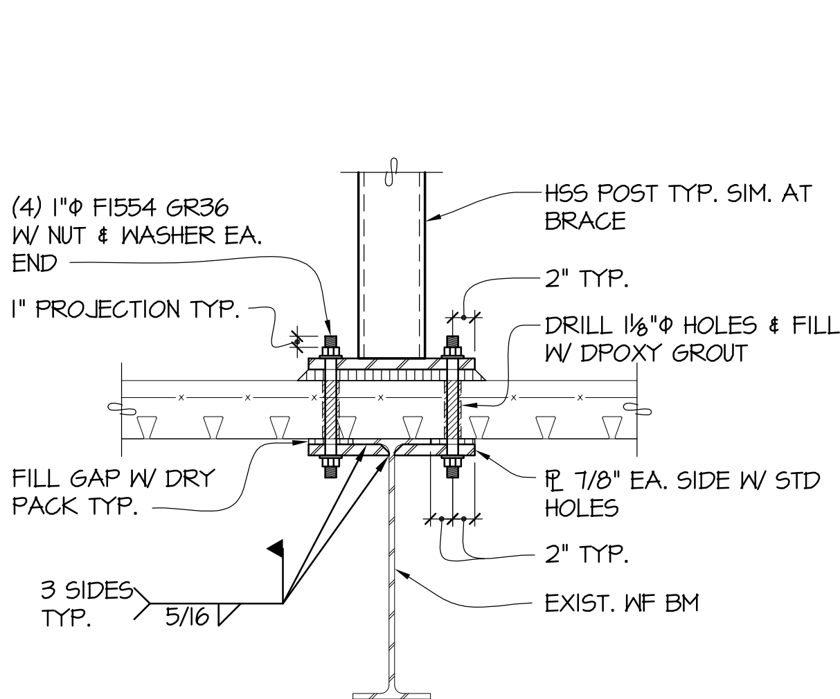
7 SECTION 55.41 1"=1'-0"
