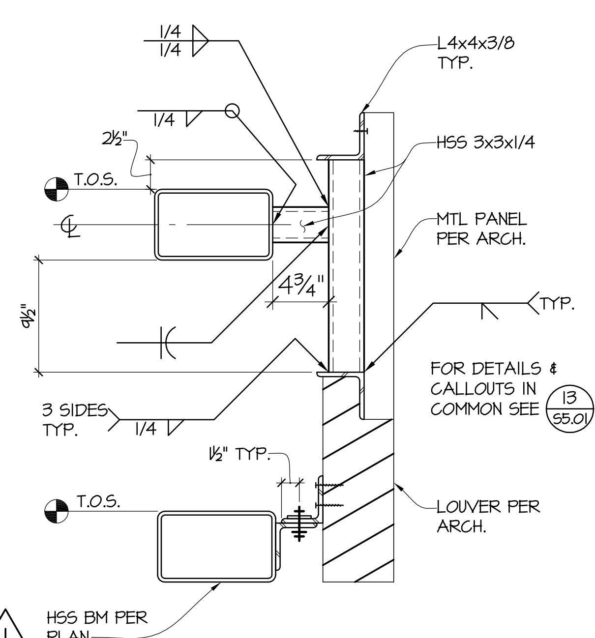
10 SECTION 55.41 1 1/2"=1'-0"
