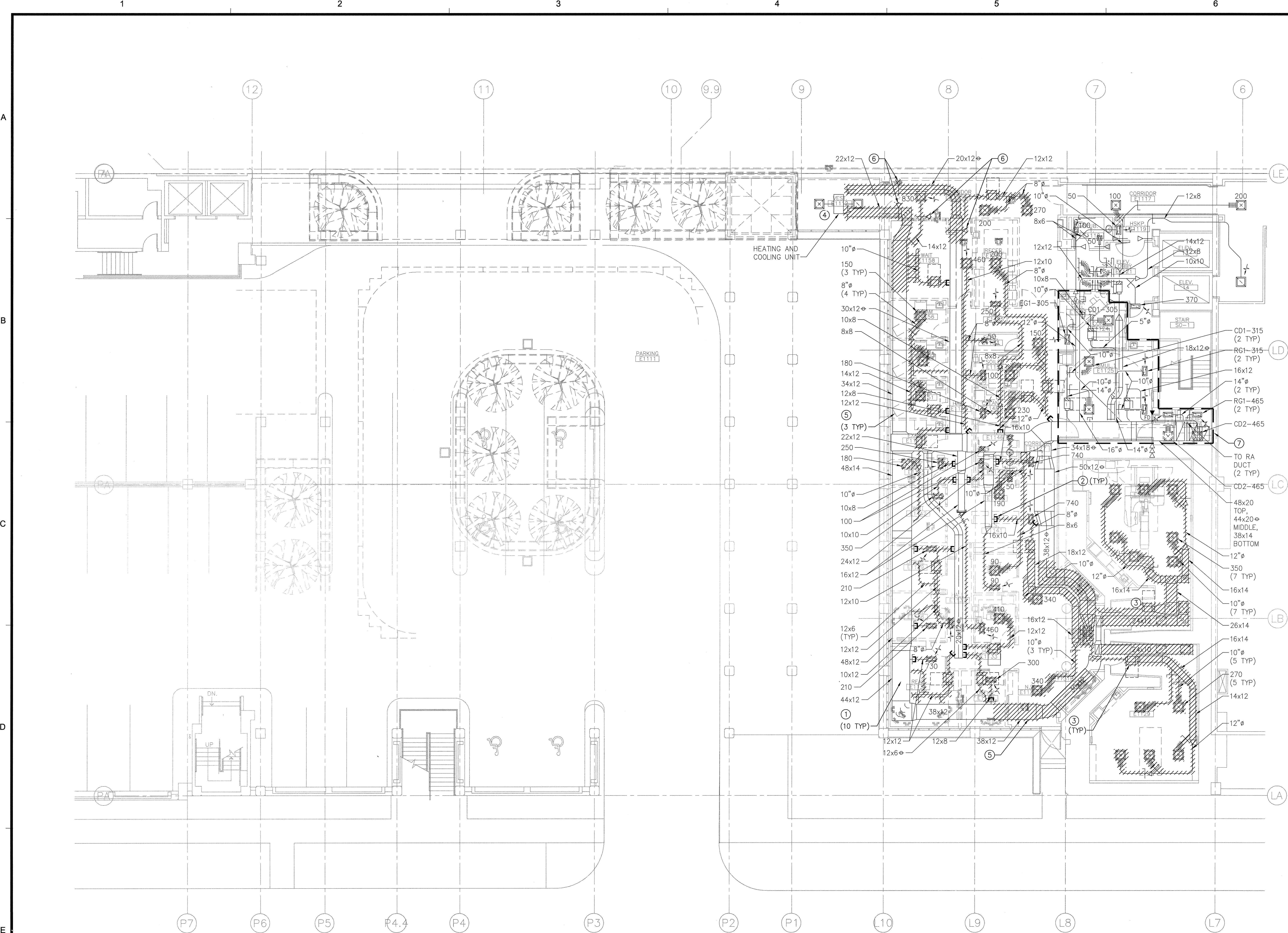
1ST FLOOR PLAN - L WING & PLAZA REMODEL - HVAC DEMOLITION SCALE: 1/8"=1'-0"
