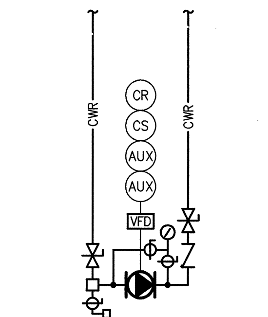
TYPICAL CHILLED WATER PUMP P-4, P-5 AND P-6 CONTROL DIAGRAM SCALE: NONE
