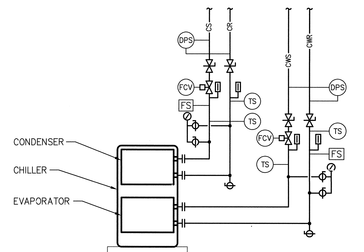
TYPICAL CHILLER CH-1, CH-2 AND CH-3 CONTROL DIAGRAM
