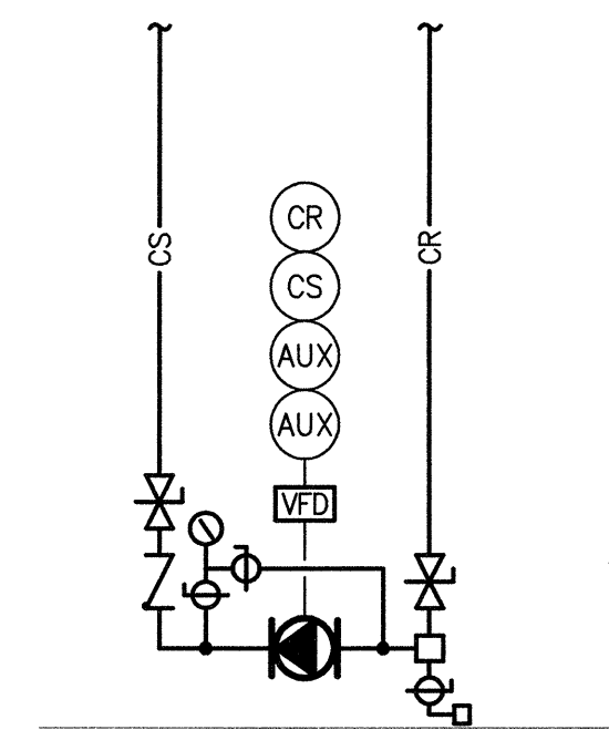
TYPICAL CONDENSER WATER PUMP P-8, P-9 AND P-10 CONTROL DIAGRAM
