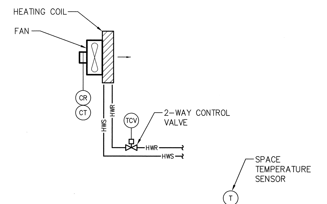
TYPICAL UNIT HEATER CONTROL DIAGRAM
