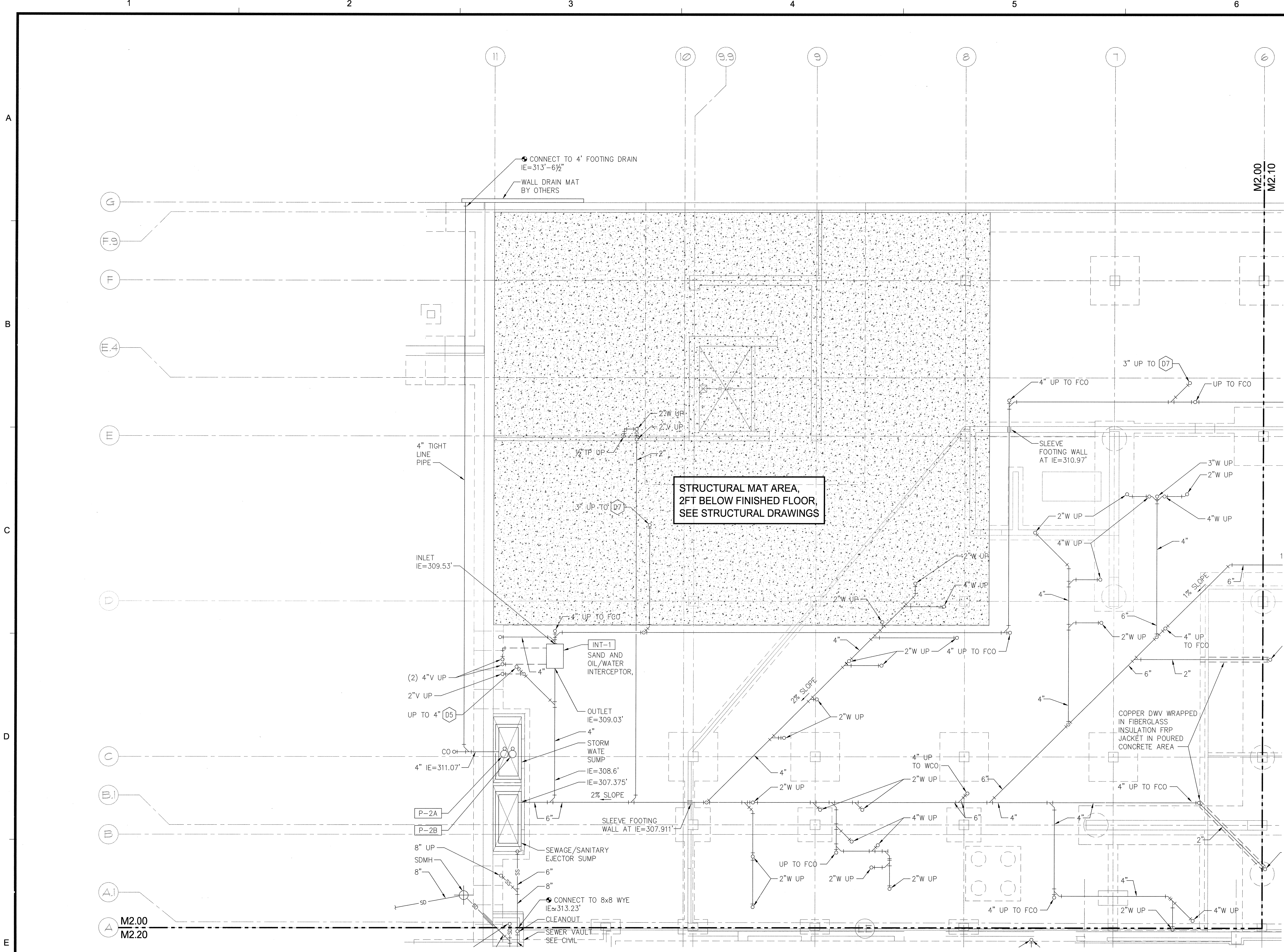
FOUNDATION PLAN - SOUTH - PLUMBING SCALE: 1/8"=1'-0"
