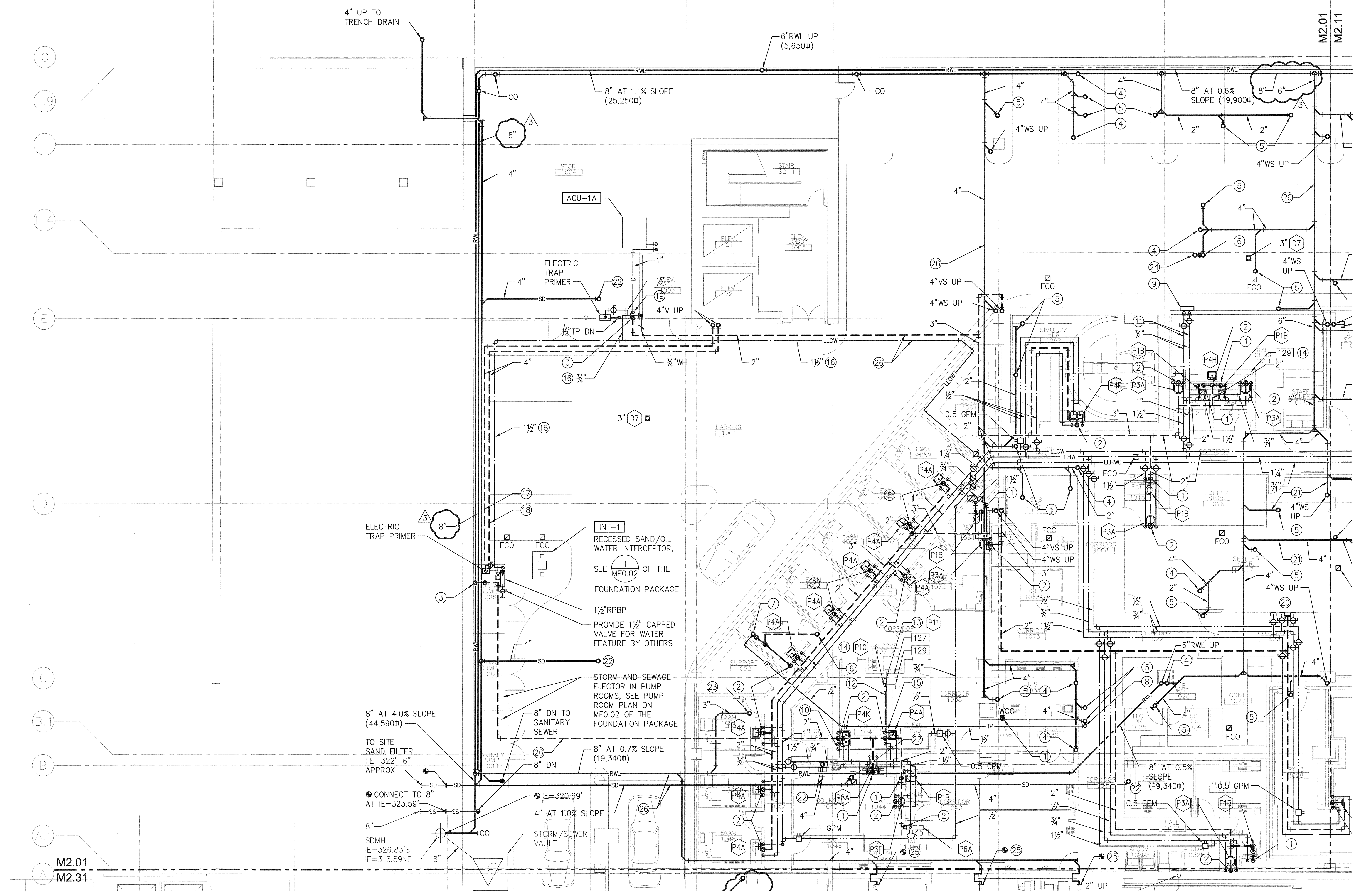
1ST FLOOR PLAN - SOUTH - PLUMBING SCALE: 1/8"=1'-0"
