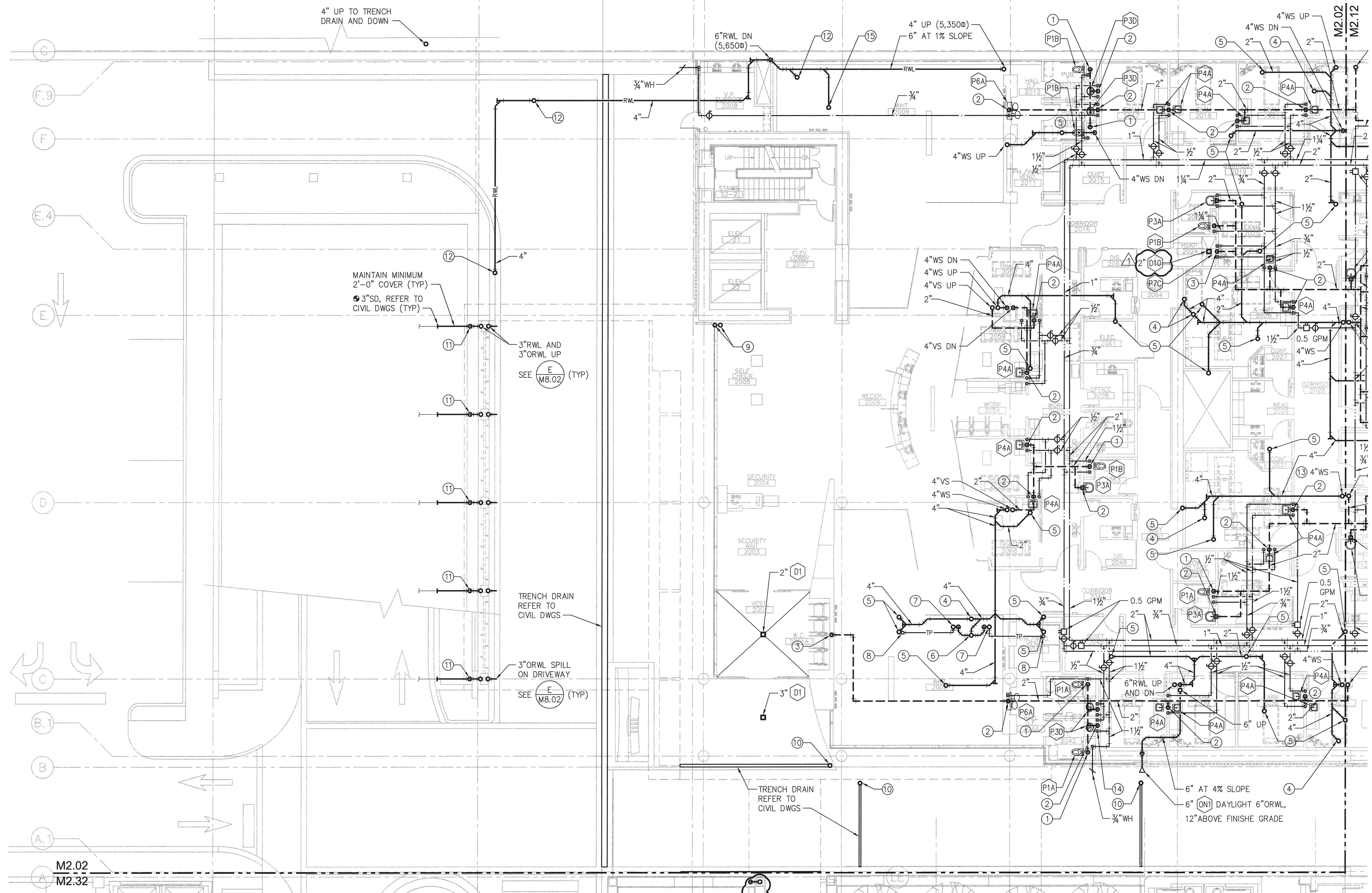
2ND FLOOR PLAN - SOUTH - PLUMBING SCALE: 1/8"=1'-0"
