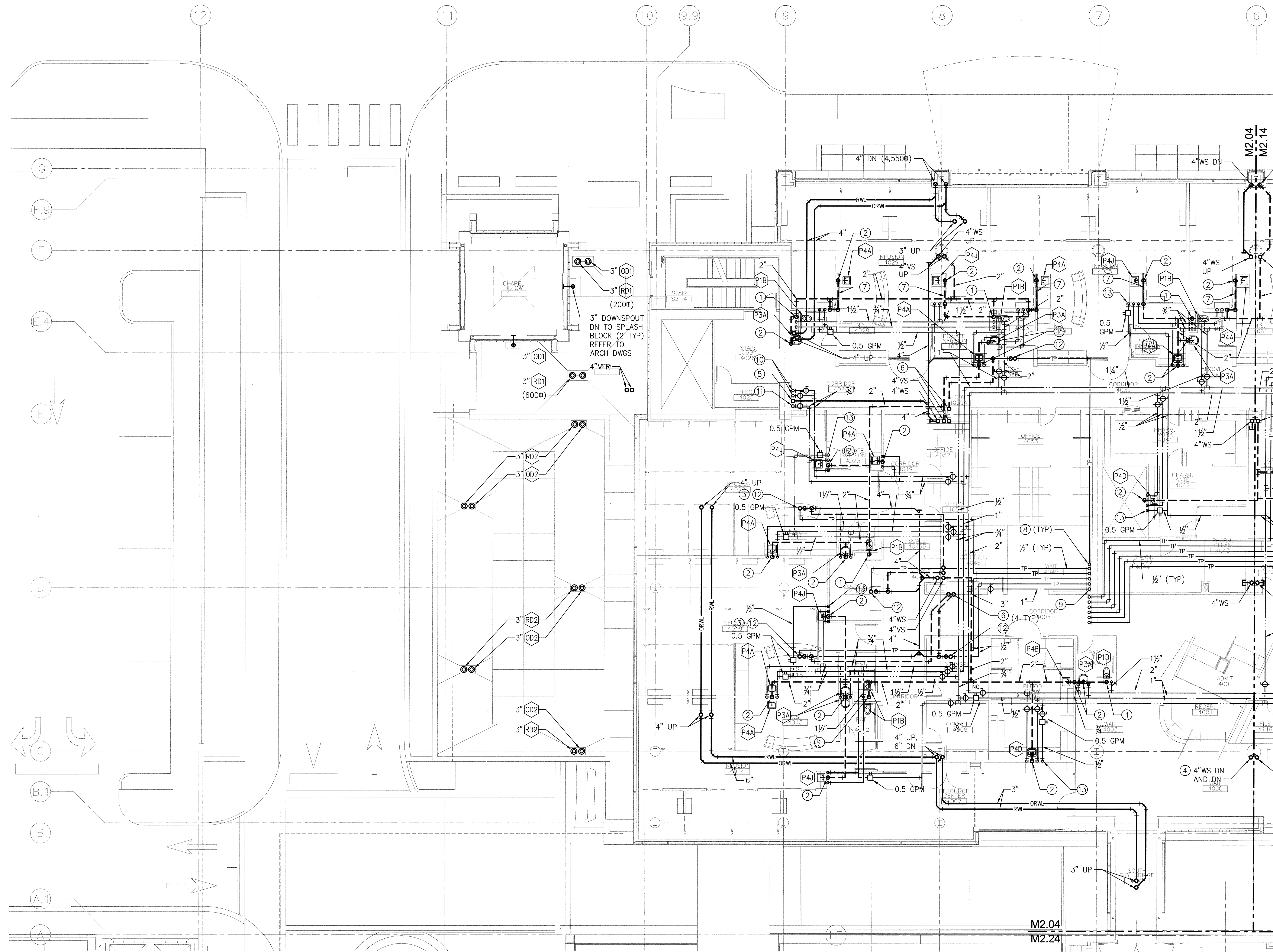
4TH FLOOR PLAN - SOUTH - PLUMBING SCALE: 1/8"=1'-0"
