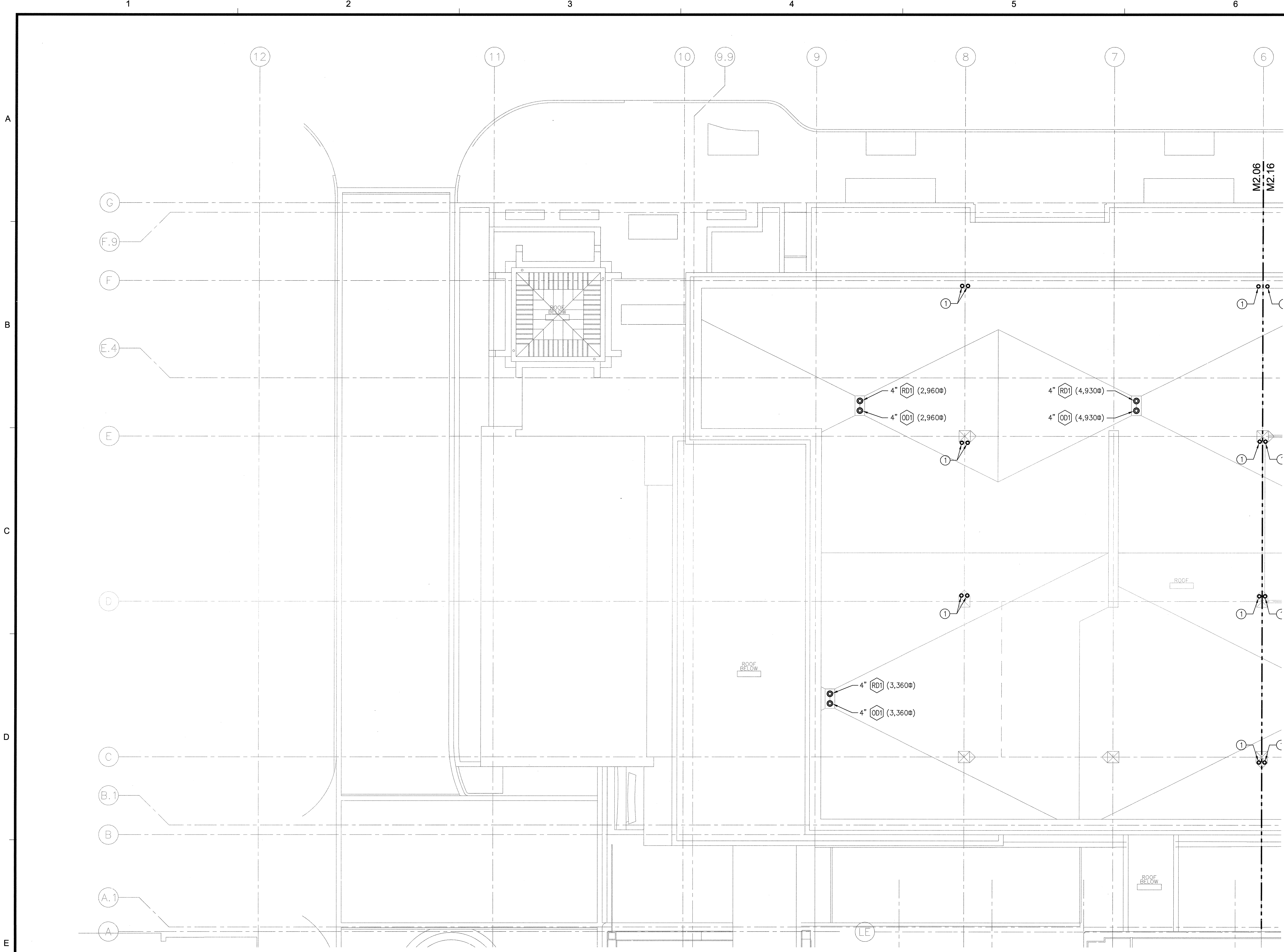
6TH FLOOR PLAN - SOUTH - PLUMBING SCALE: 1/8"=1'-0"
