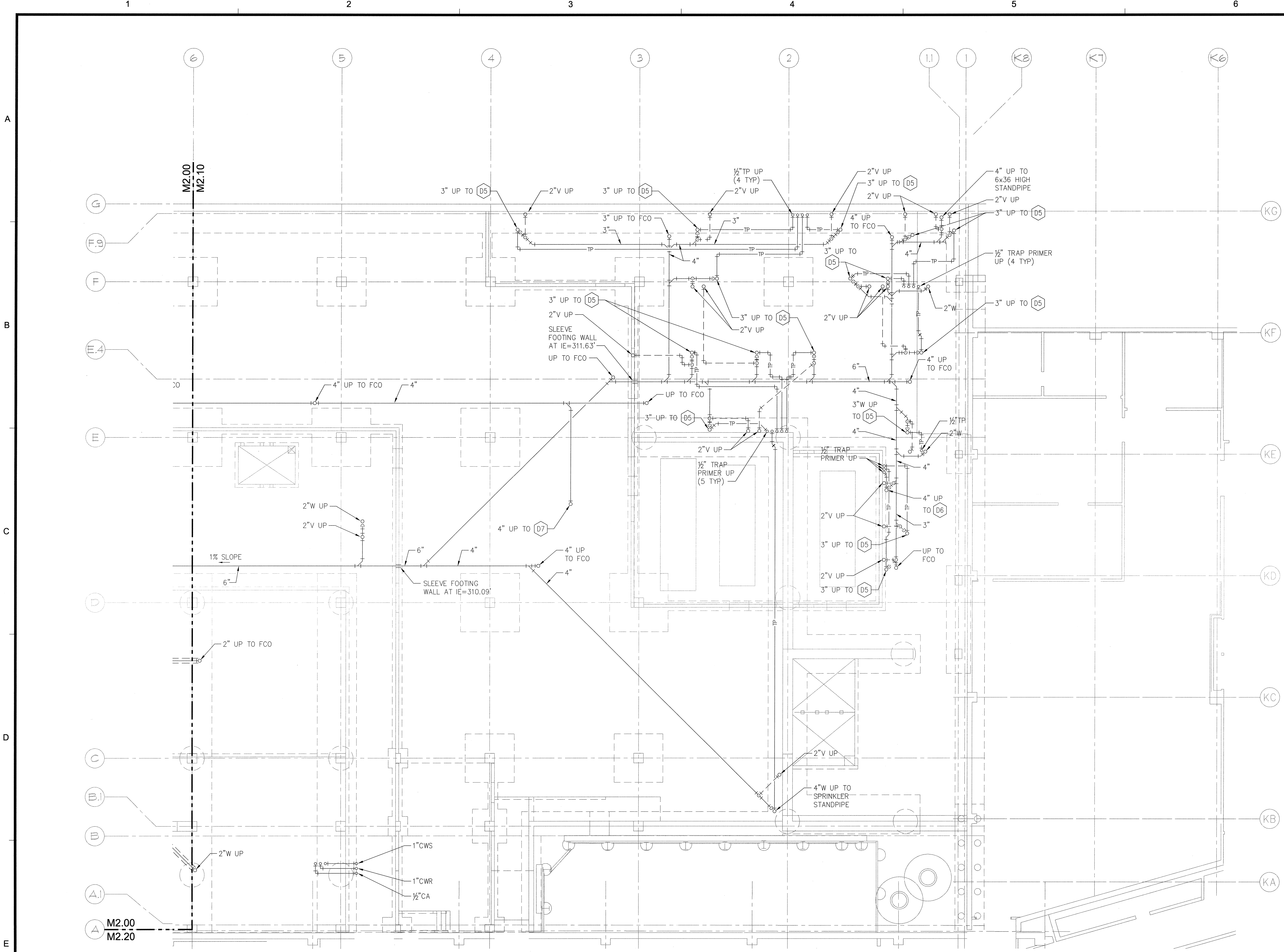
FOUNDATION PLAN - NORTH - PLUMBING SCALE: 1/8"=1'-0"
