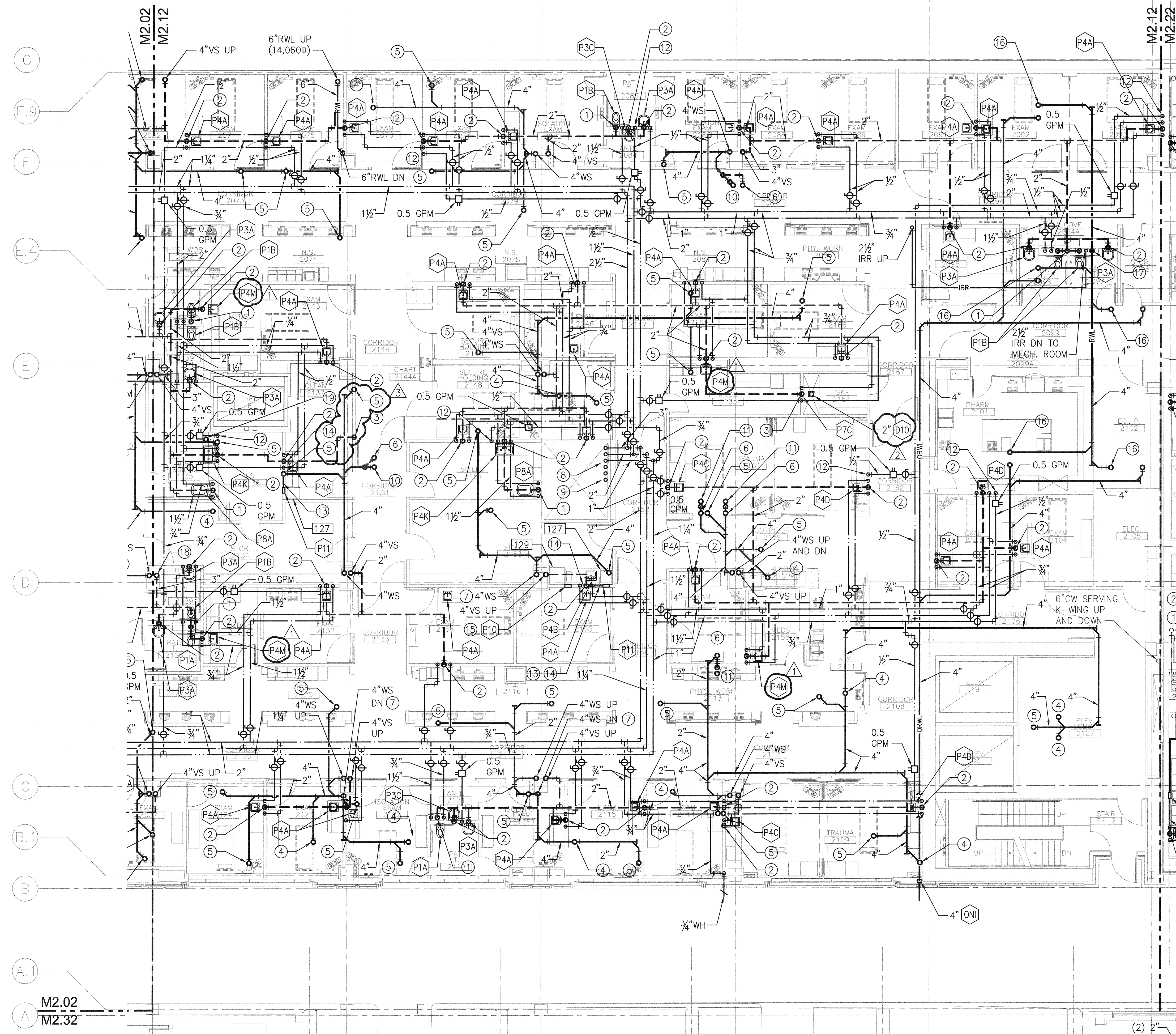
2ND FLOOR PLAN - NORTH - PLUMBING
