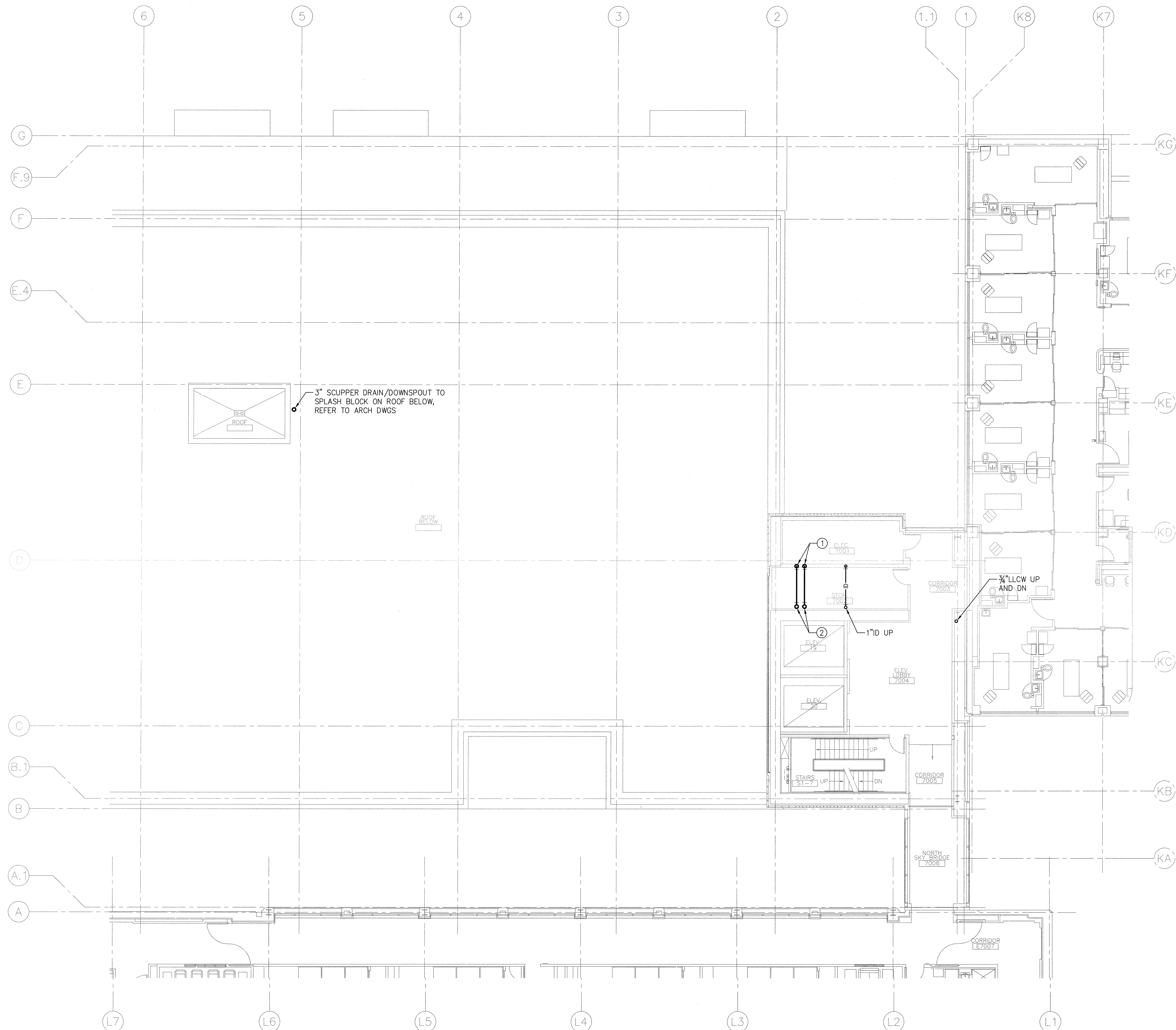
7TH FLOOR PLAN - NORTH - PLUMBING SCALE: 1/8"=1'-0"
