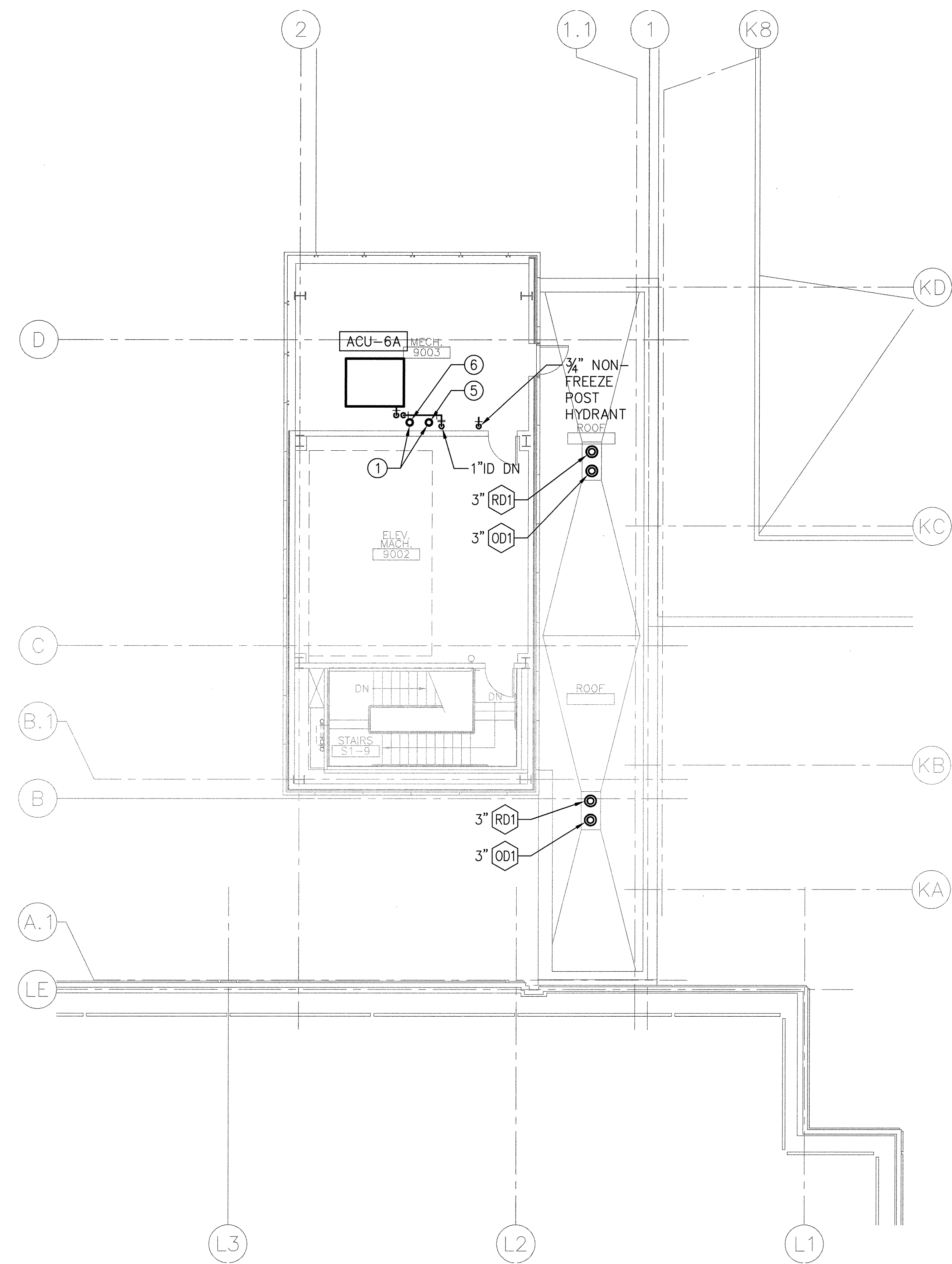
PARTIAL 9TH FLOOR PLAN - PLUMBING SCALE: 1/8"=1'-0"
