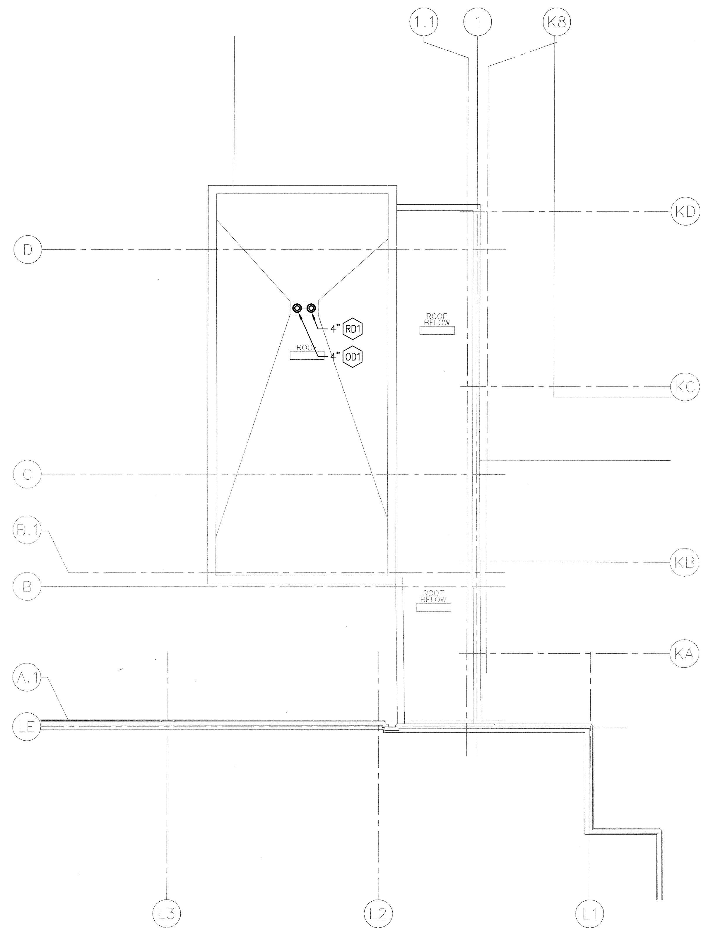
PARTIAL ROOF PLAN - PLUMBING SCALE: 1/8"=1'-0"
