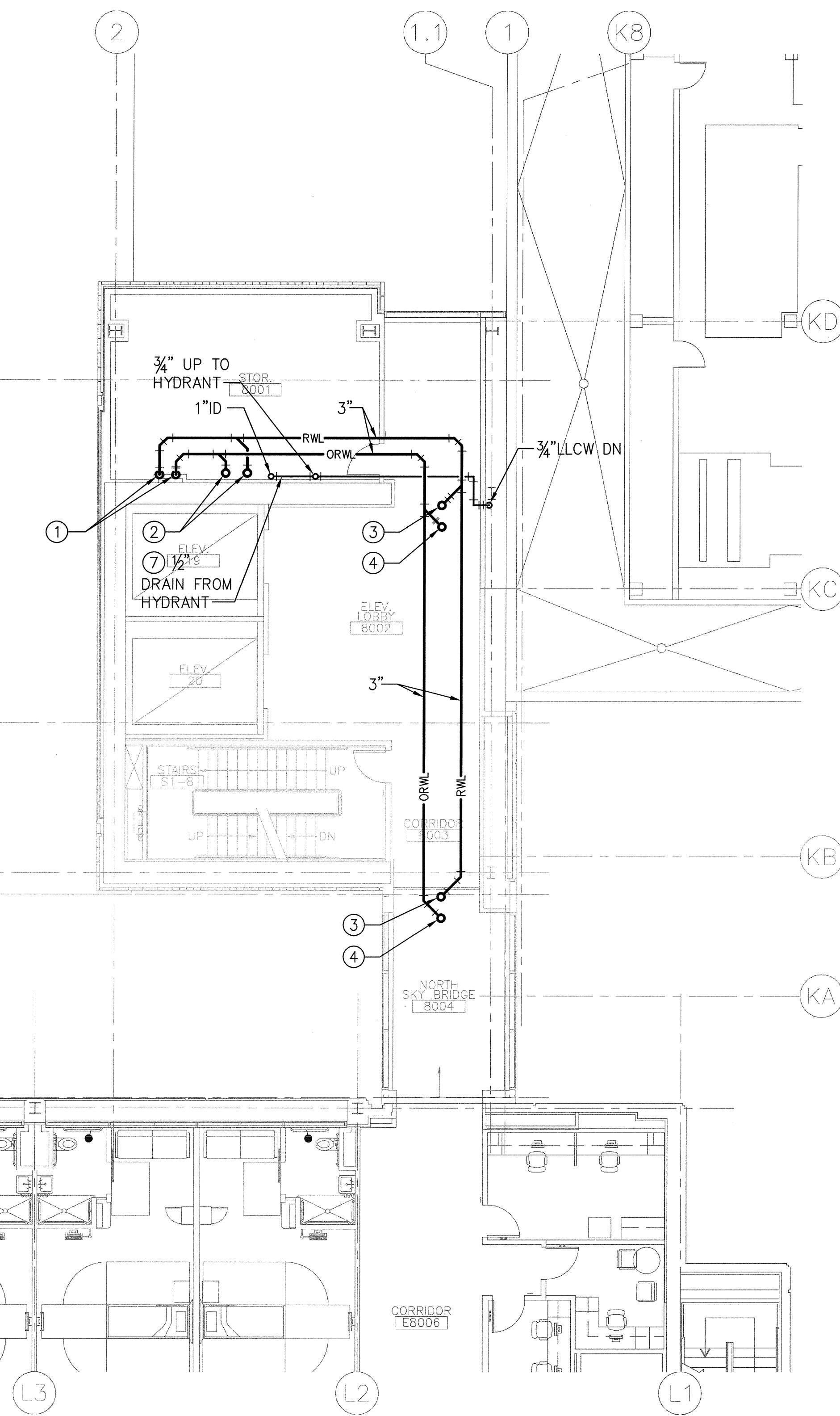
PARTIAL 8TH FLOOR PLAN - PLUMBING SCALE: 1/8"=1'-0"
