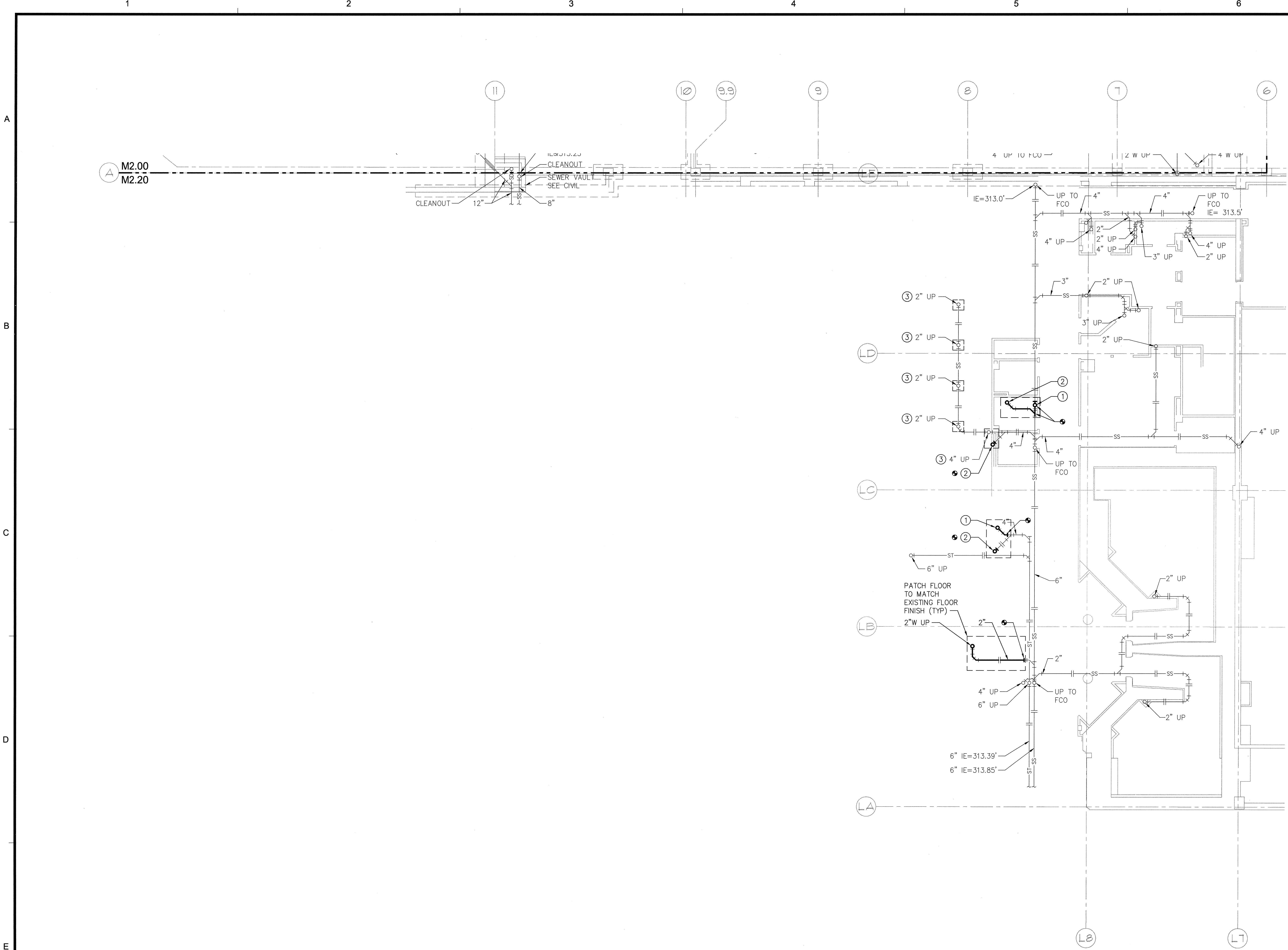
FOUNDATION PLAN - L WING & PLAZA REMODEL - PLUMBING SCALE: 1/8"=1'-0"
