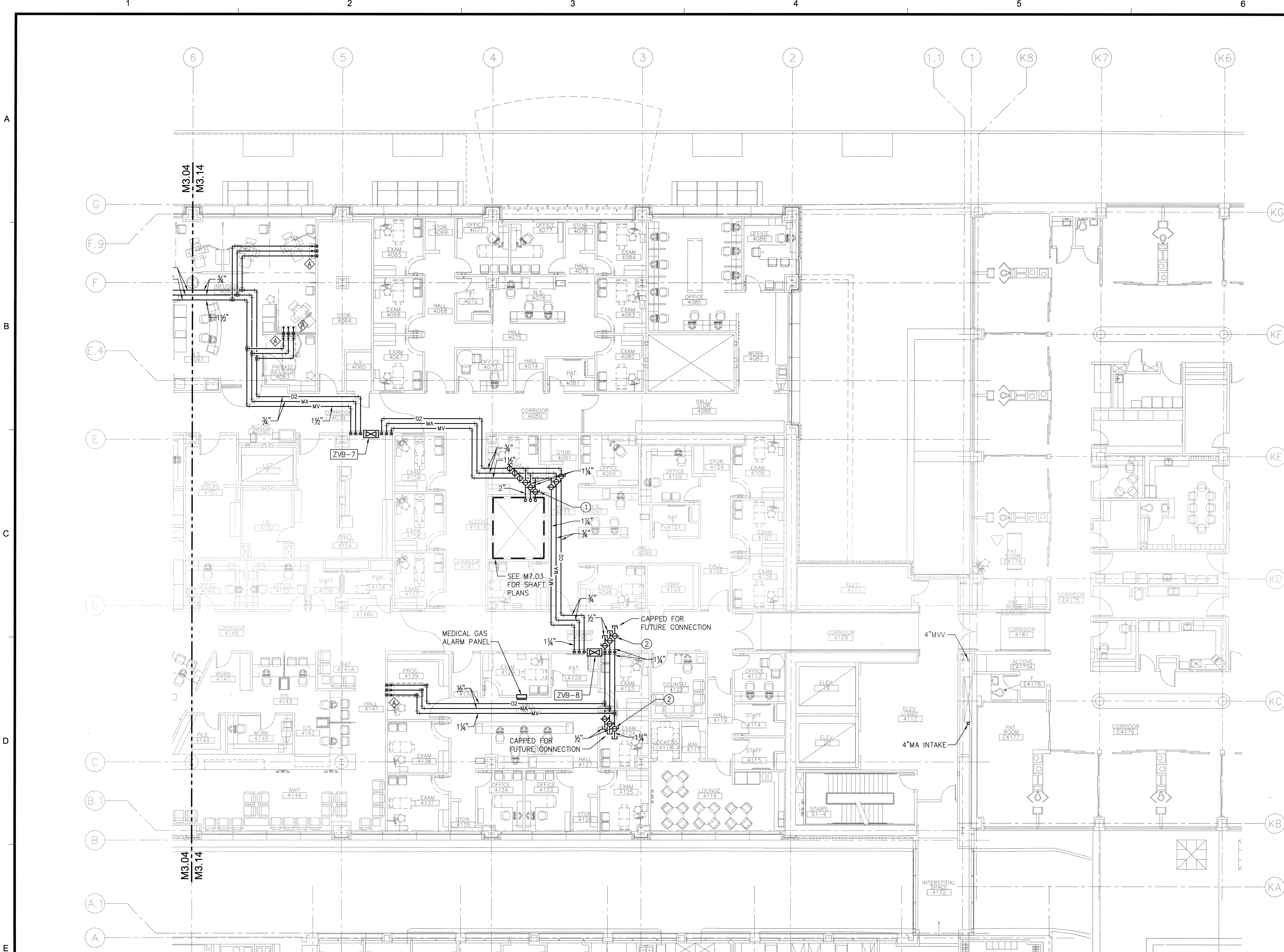
4TH FLOOR PLAN - NORTH - MEDICAL GAS PIPING SCALE: 1/8"=1'-0"
