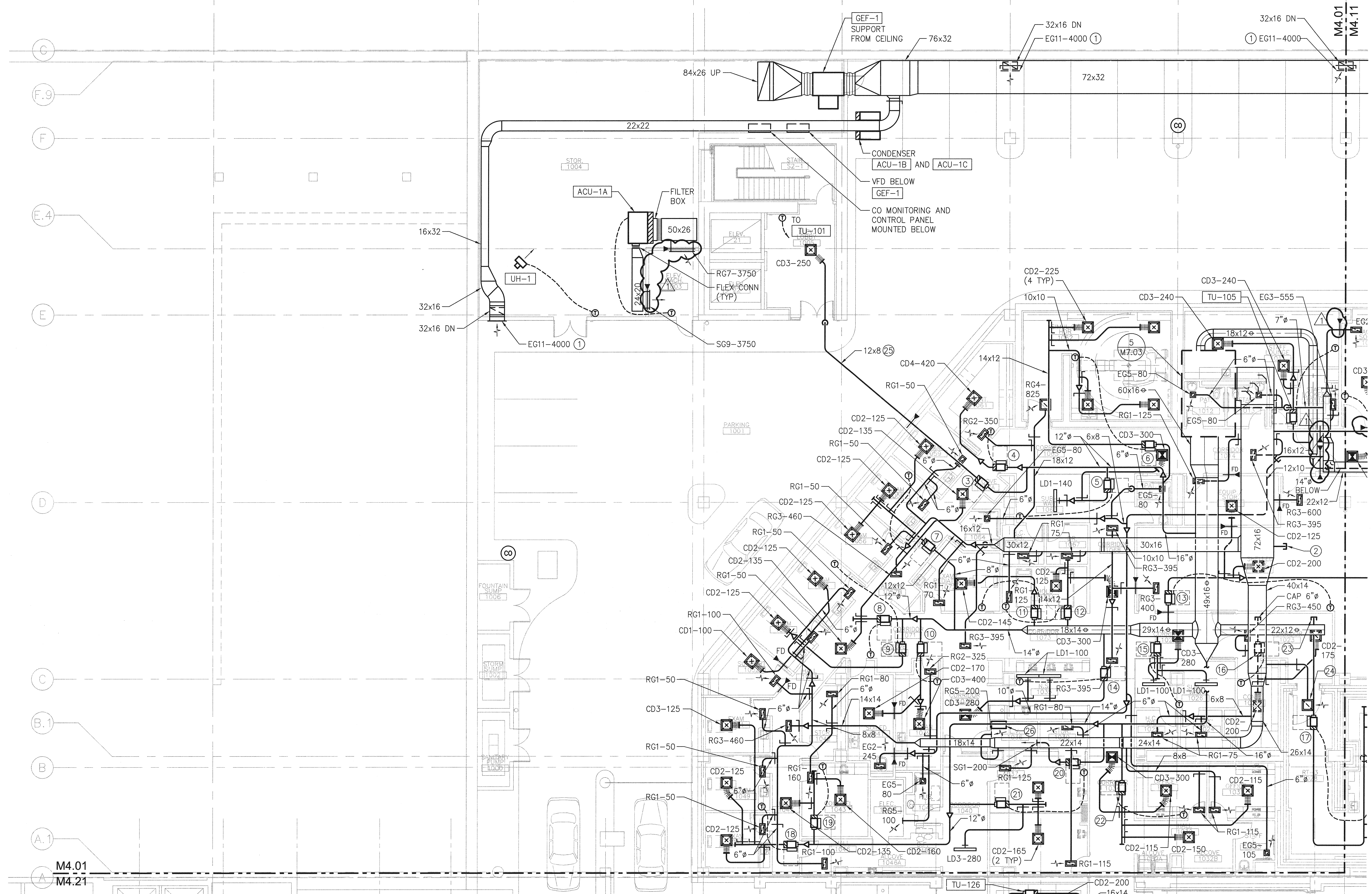
1ST FLOOR PLAN - SOUTH - HVAC SCALE: 1/8"=1'-0"
