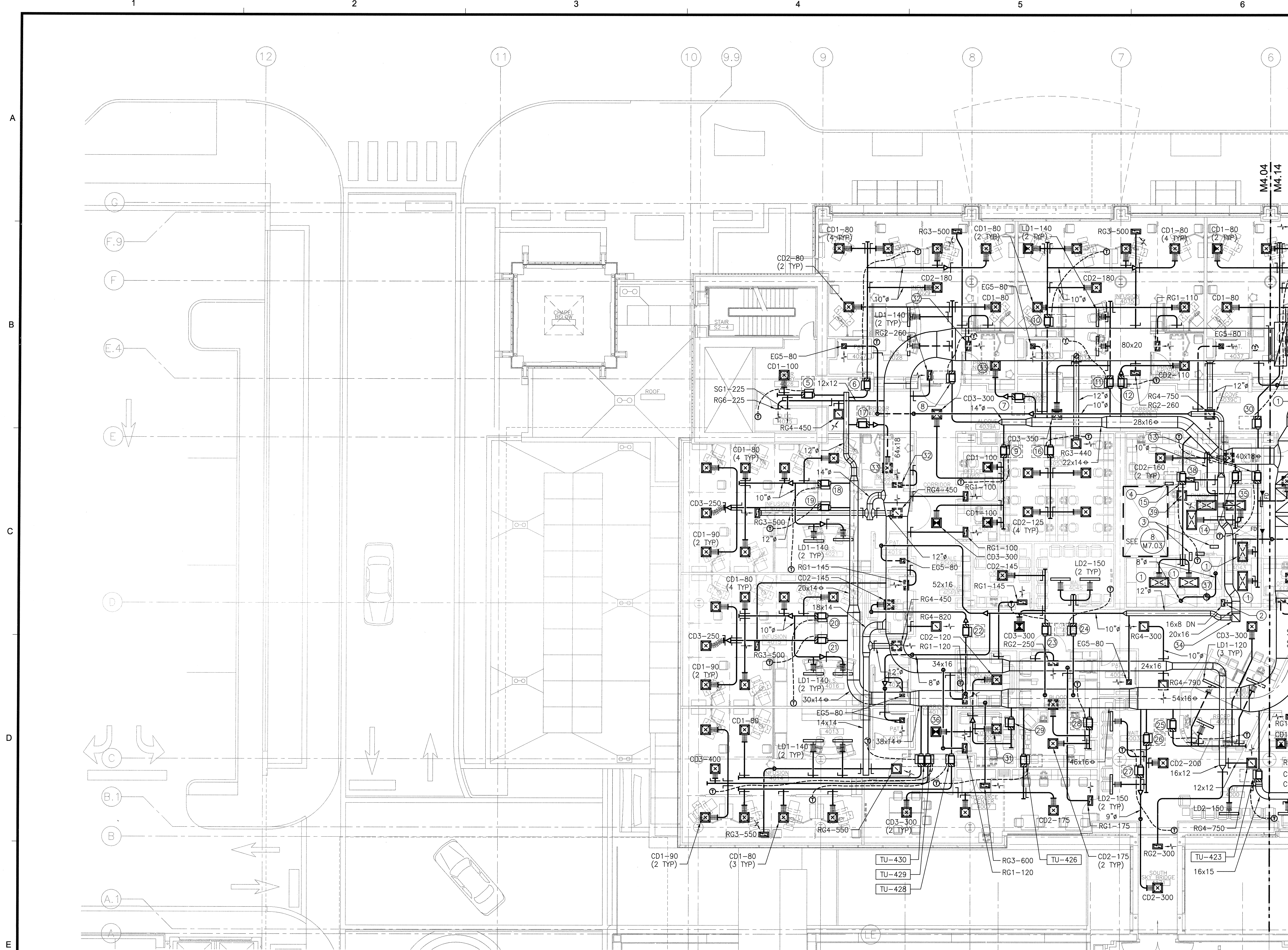
4TH FLOOR PLAN - SOUTH - HVAC SCALE: 1/8"=1'-0"
