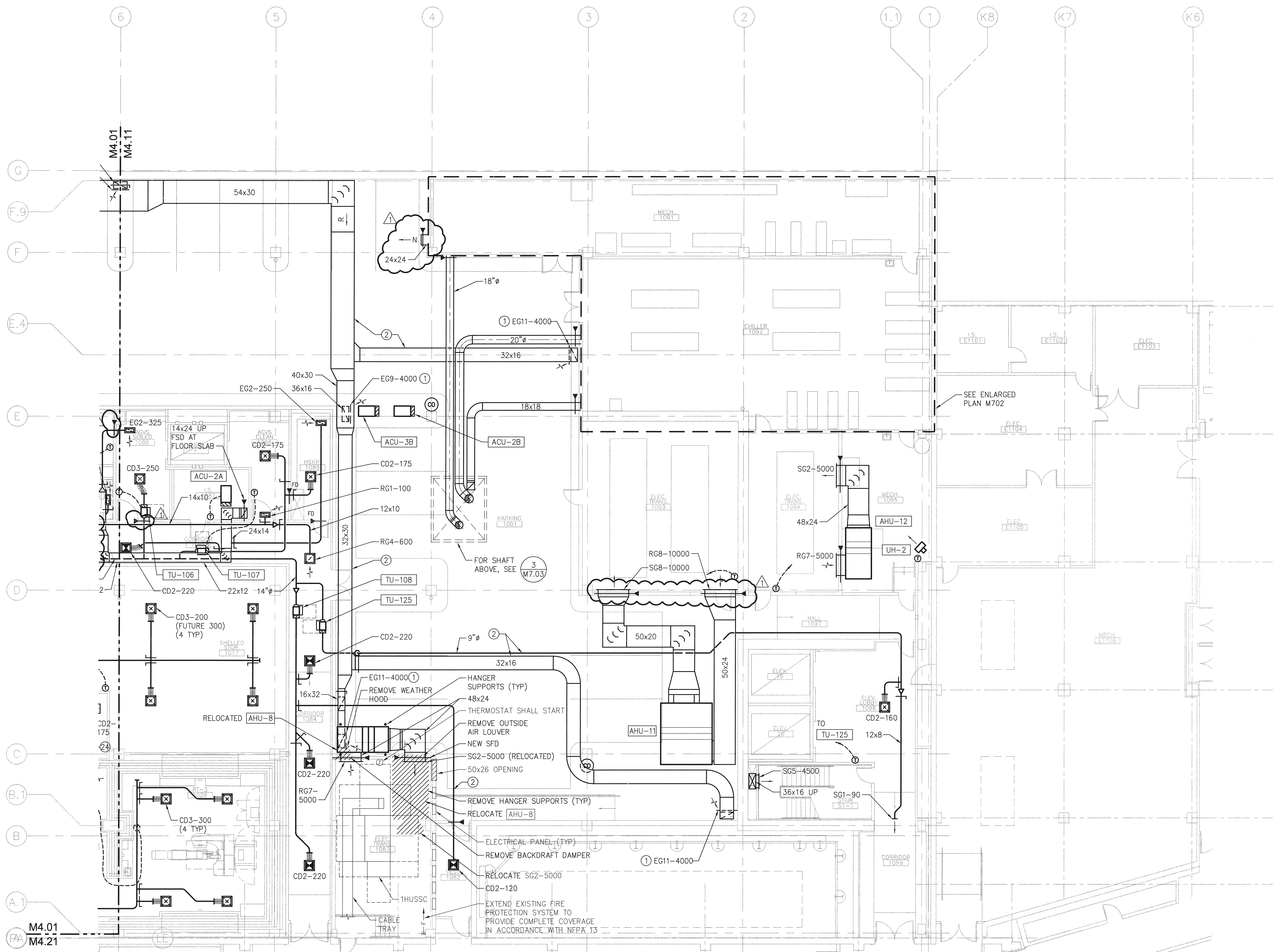
1ST FLOOR PLAN - NORTH - HVAC SCALE: 1/8"=1'-0"
