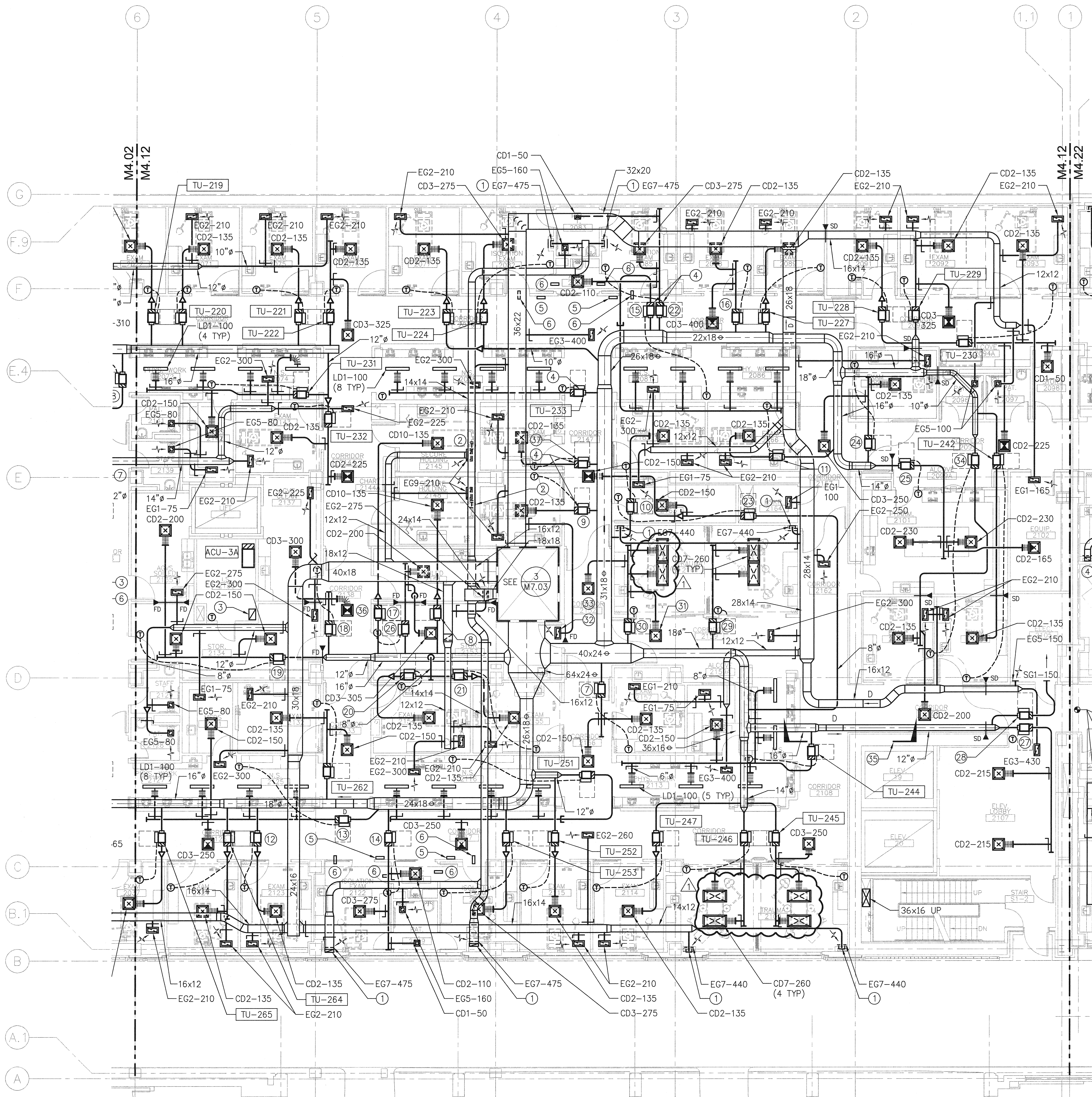
2ND FLOOR PLAN - NORTH - HVAC
