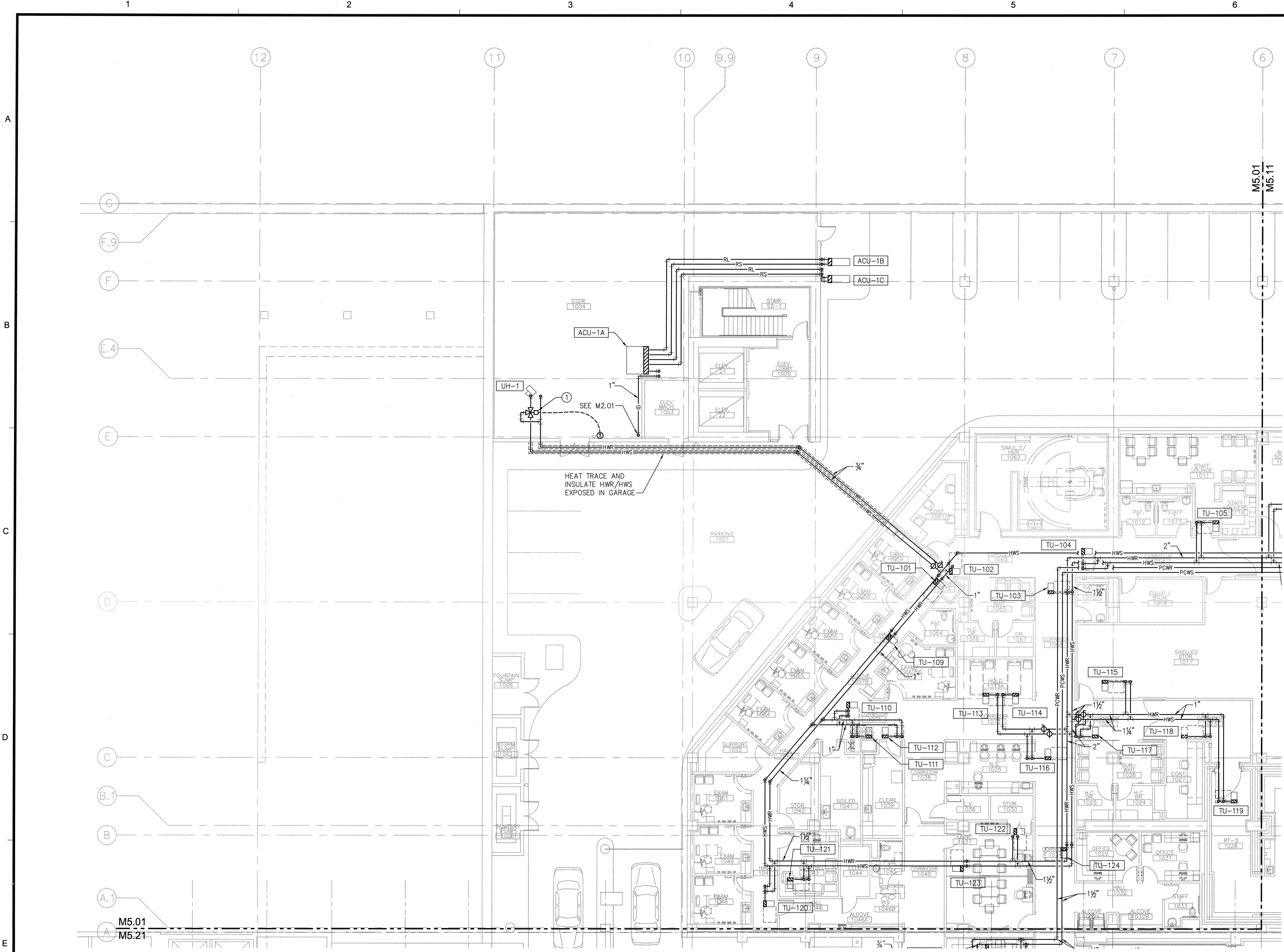
1ST FLOOR PLAN - SOUTH - HVAC PIPING SCALE: 1/8"=1'-0"
