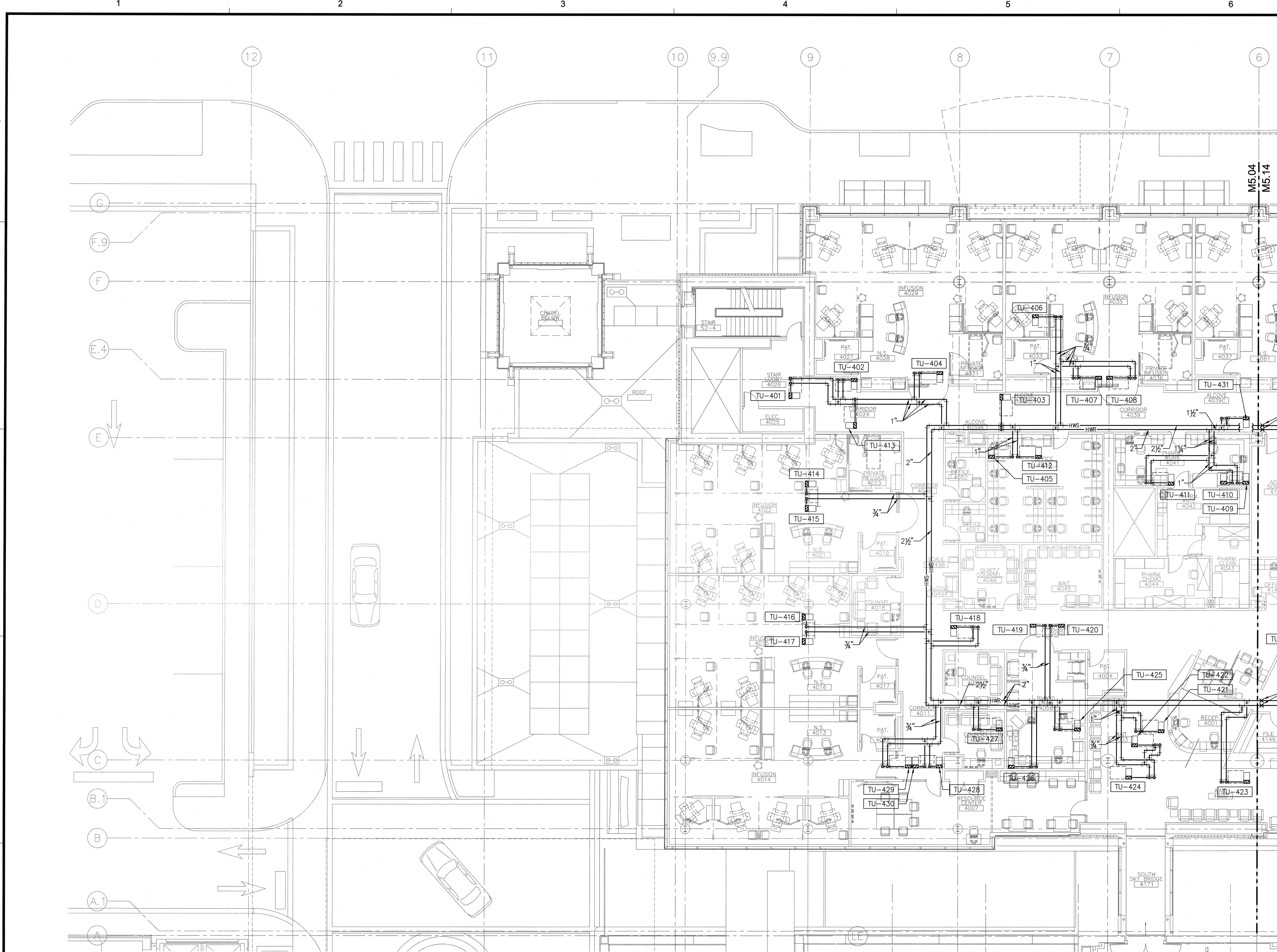
4TH FLOOR PLAN - SOUTH - HVAC PIPING SCALE: 1/8"=1'-0"
