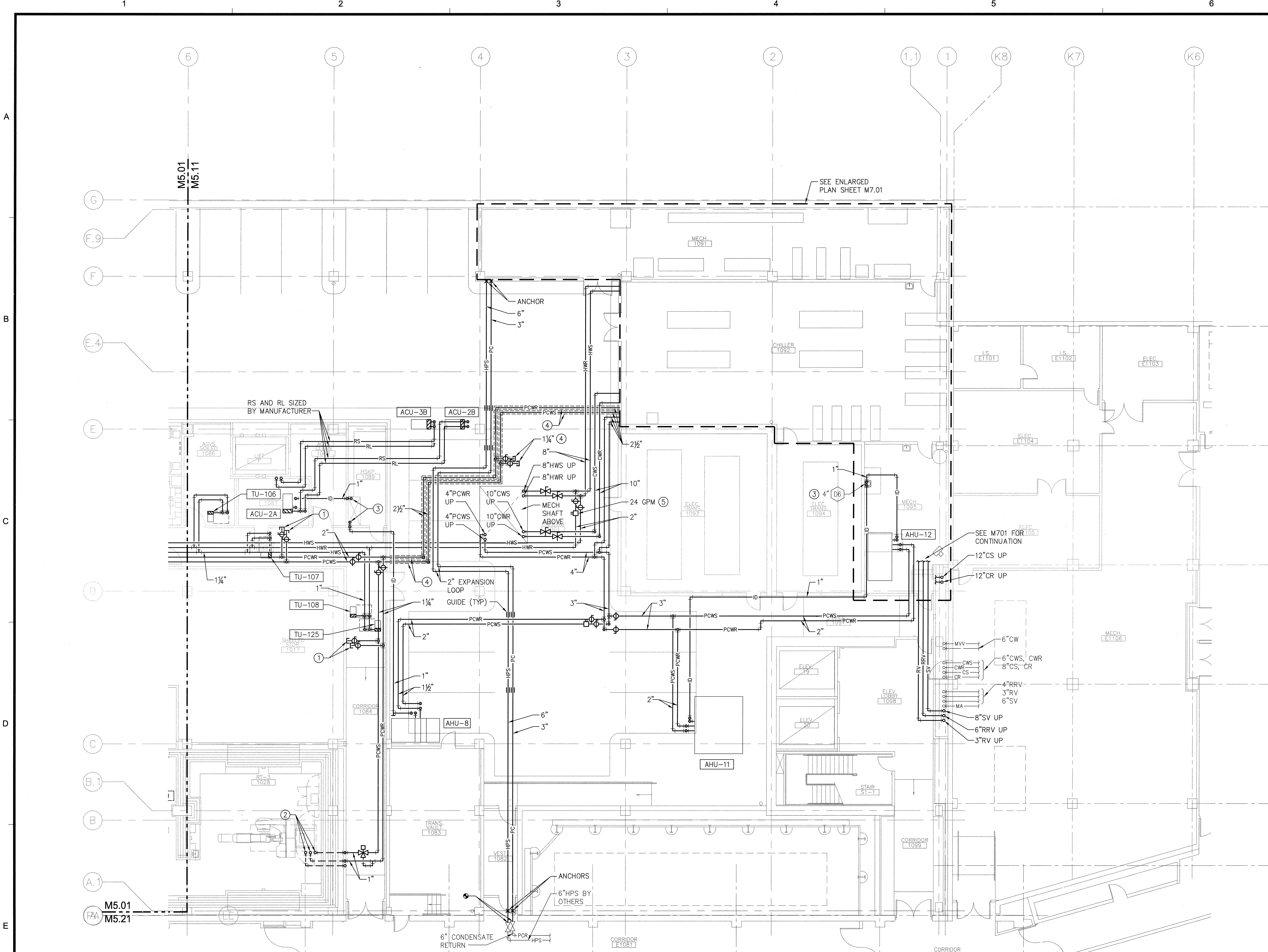
1ST FLOOR PLAN - NORTH - HVAC PIPING SCALE: 1/8"=1'-0"
