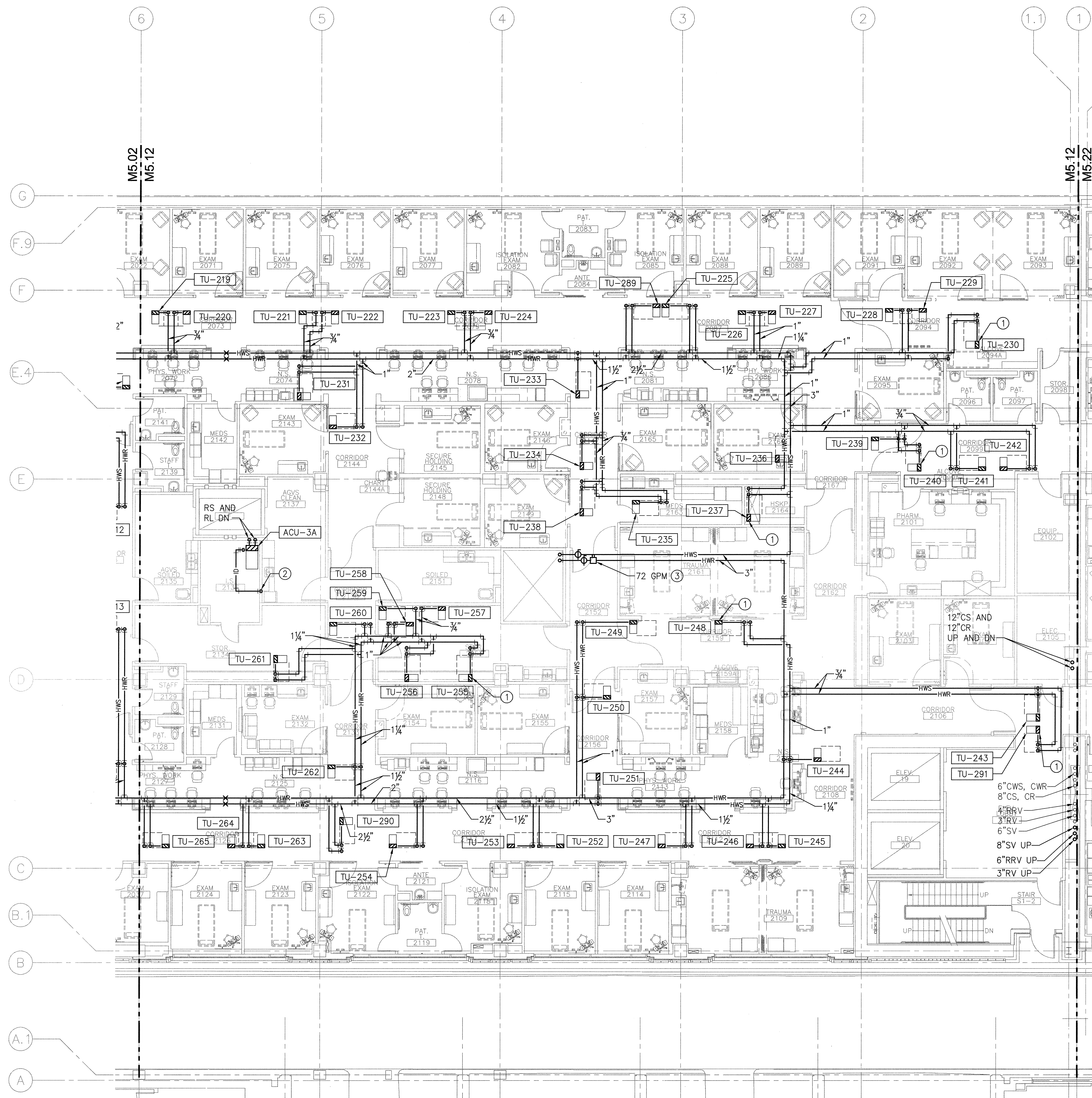
2ND FLOOR PLAN - NORTH - HVAC PIPING SCALE: 1/8"=1'-0"
