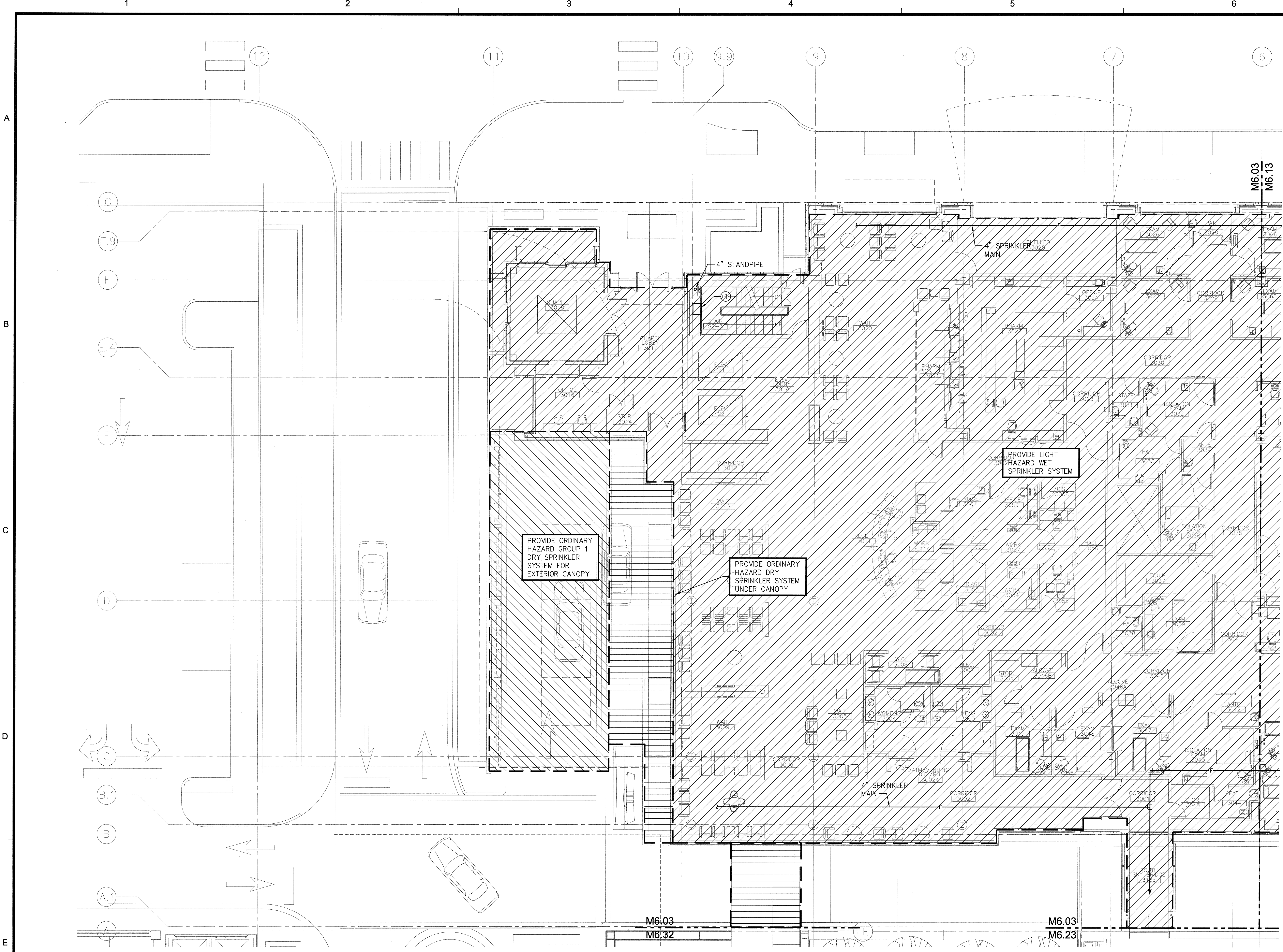
3RD FLOOR PLAN - SOUTH - FIRE PROTECTION SCALE: 1/8"=1'-0"
