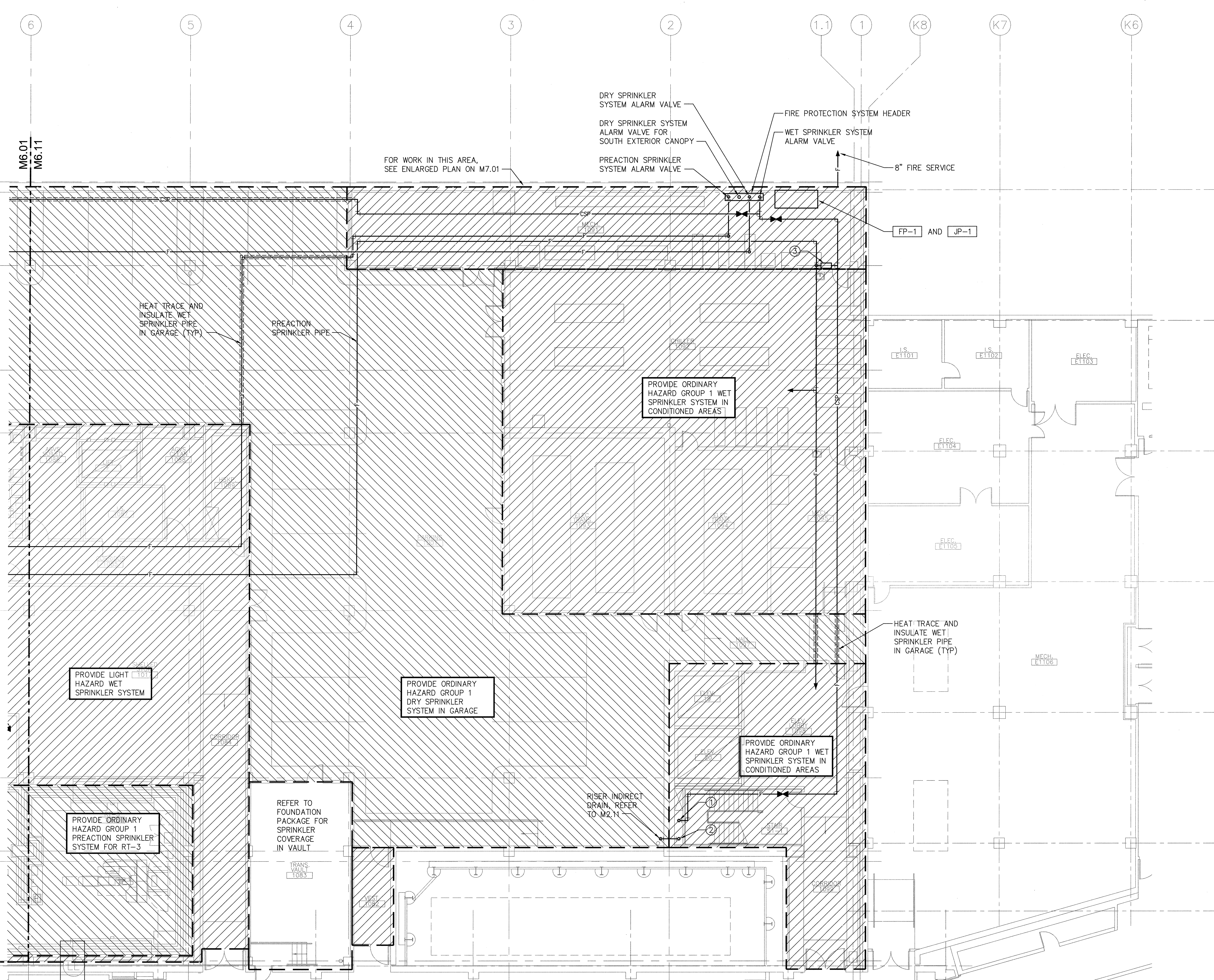
1ST FLOOR PLAN - NORTH - FIRE PROTECTION SCALE: 1/8"=1'-0"
