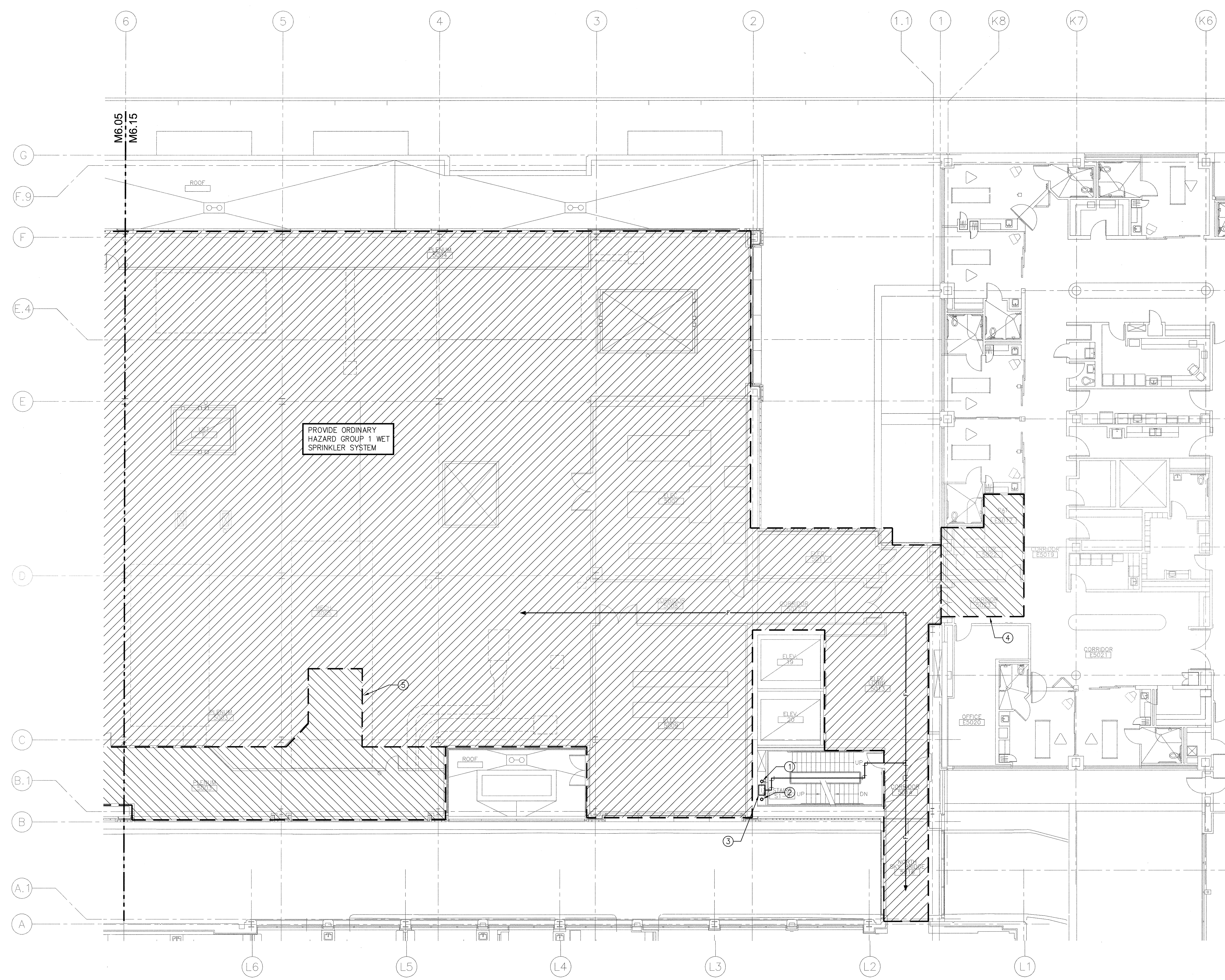
5TH FLOOR PLAN - NORTH - FIRE PROTECTION SCALE: 1/8"=1'-0"
