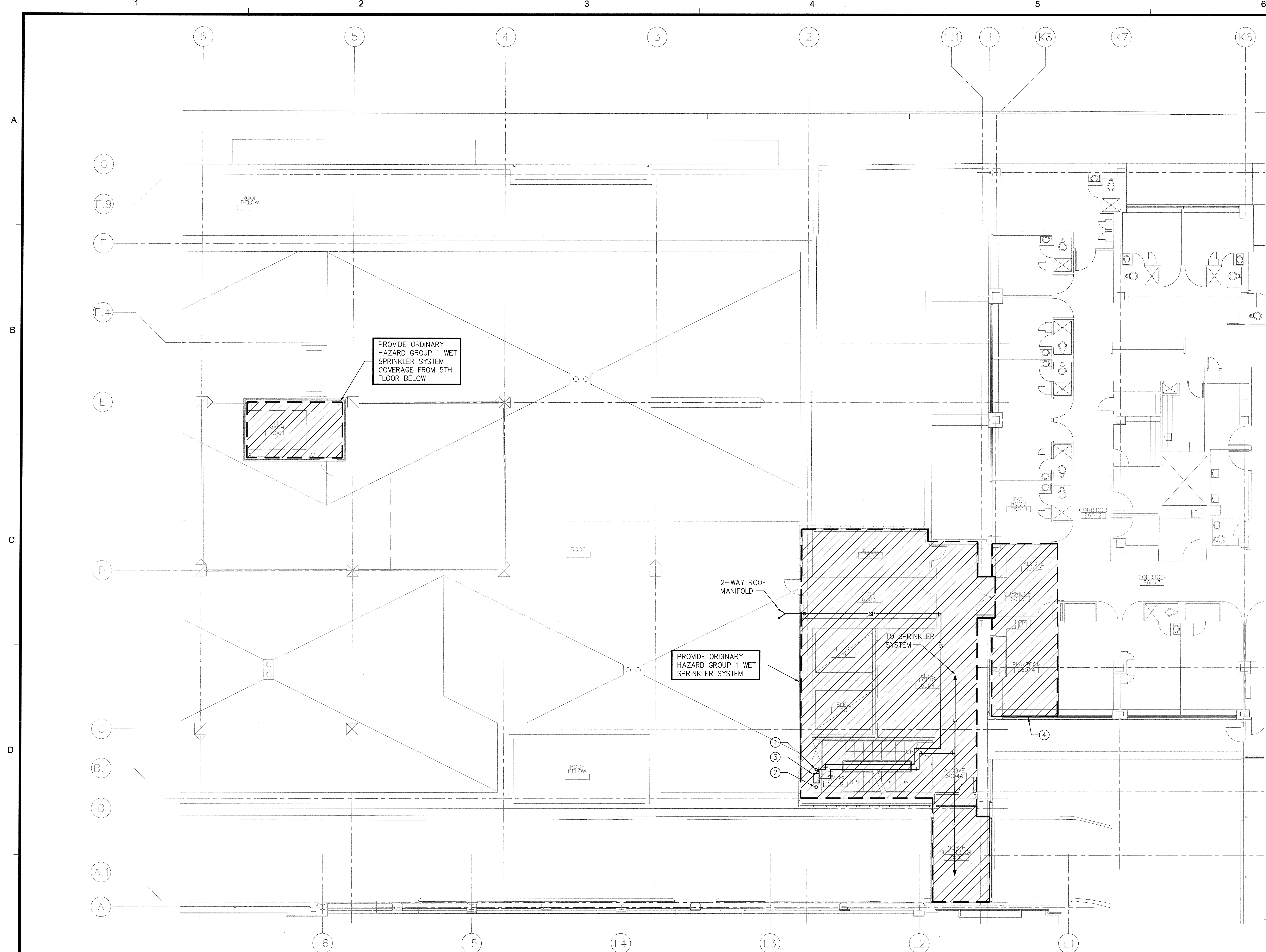
6TH FLOOR PLAN - NORTH - FIRE PROTECTION
