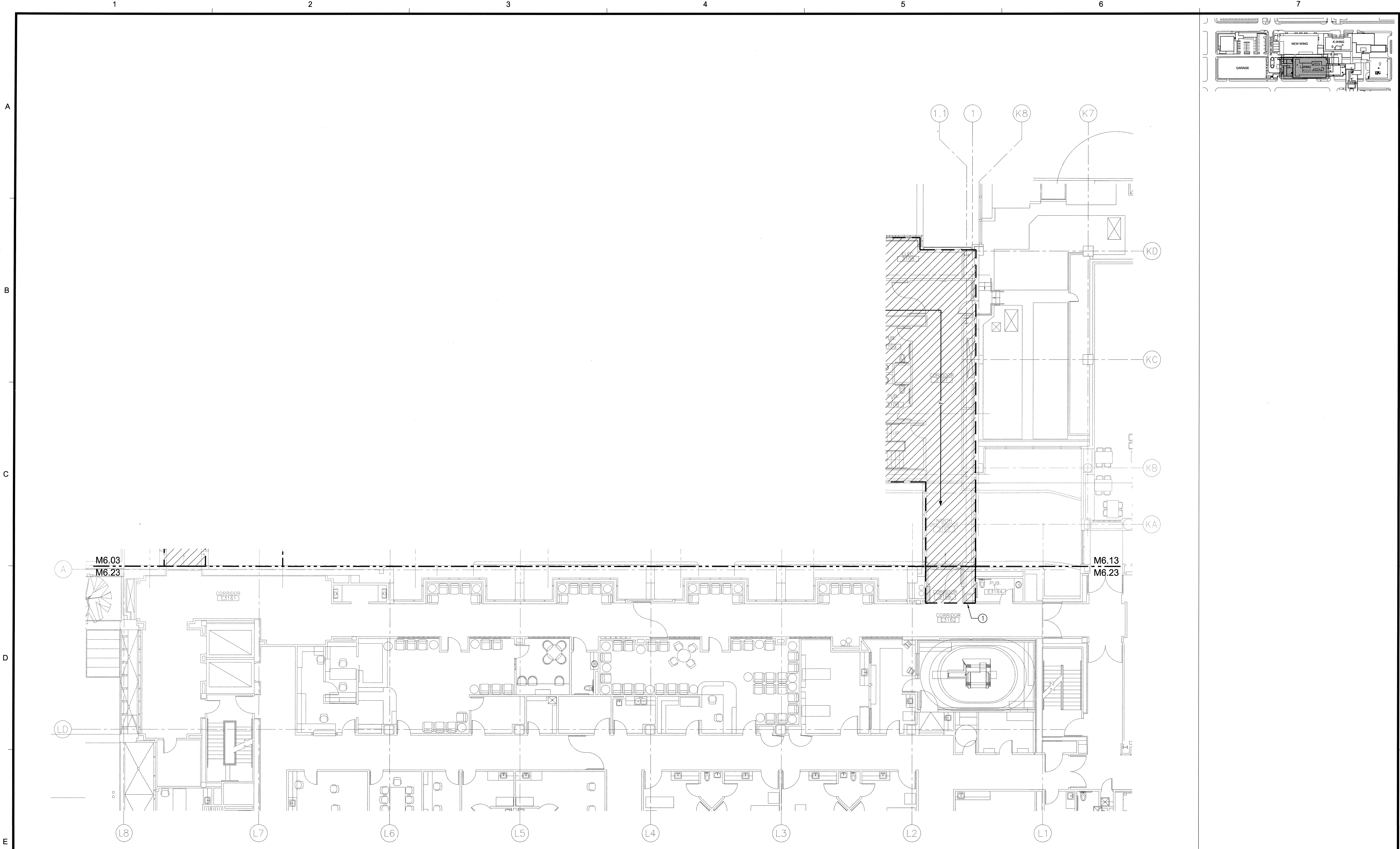
3RD FLOOR PLAN - L & K WING REMODEL - FIRE PROTECTION SCALE: 1/8"=1'-0"
