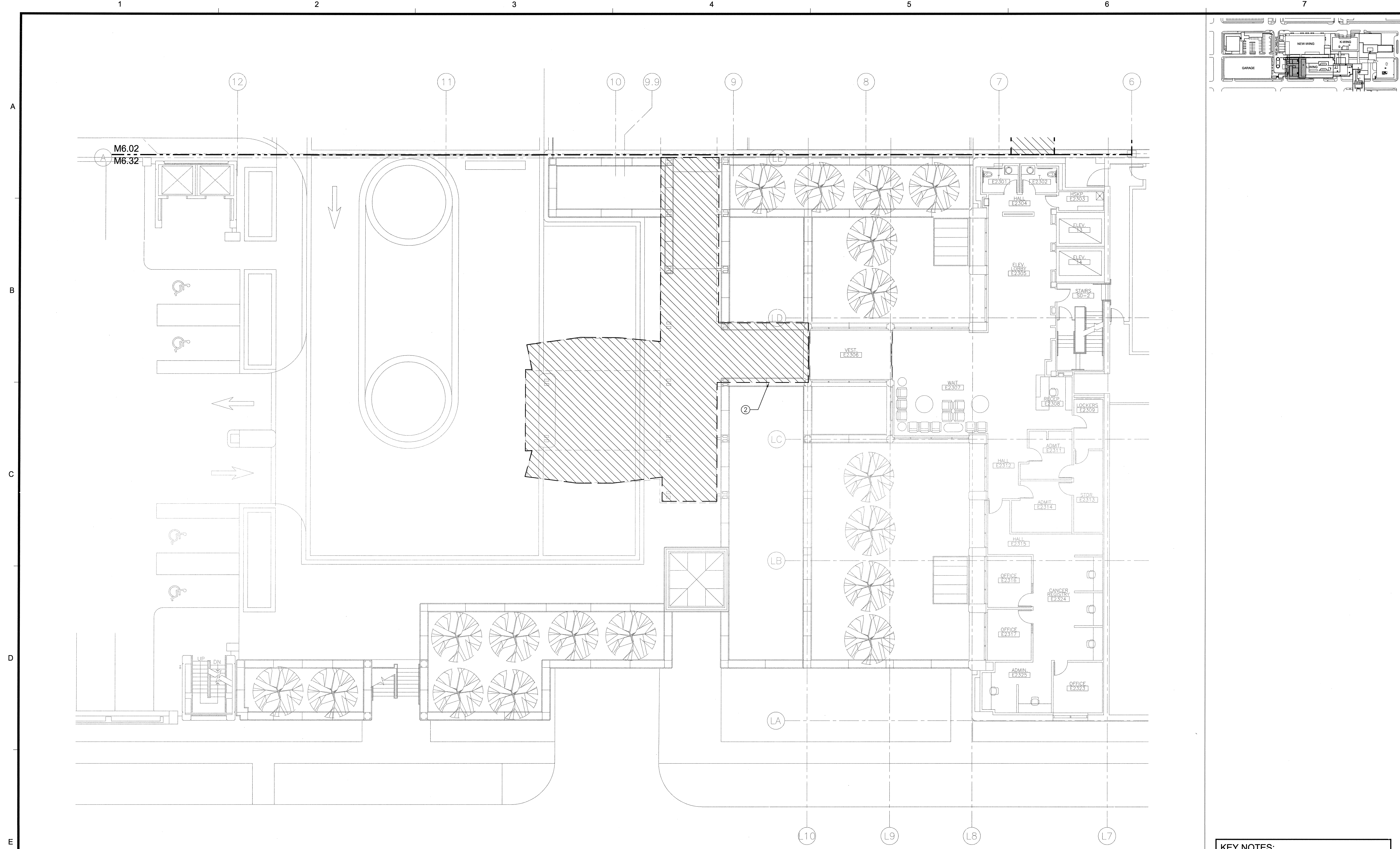
2ND FLOOR PLAN - L WING & PLAZA REMODEL - FIRE PROTECTION SCALE: 1/8"=1'-0"
